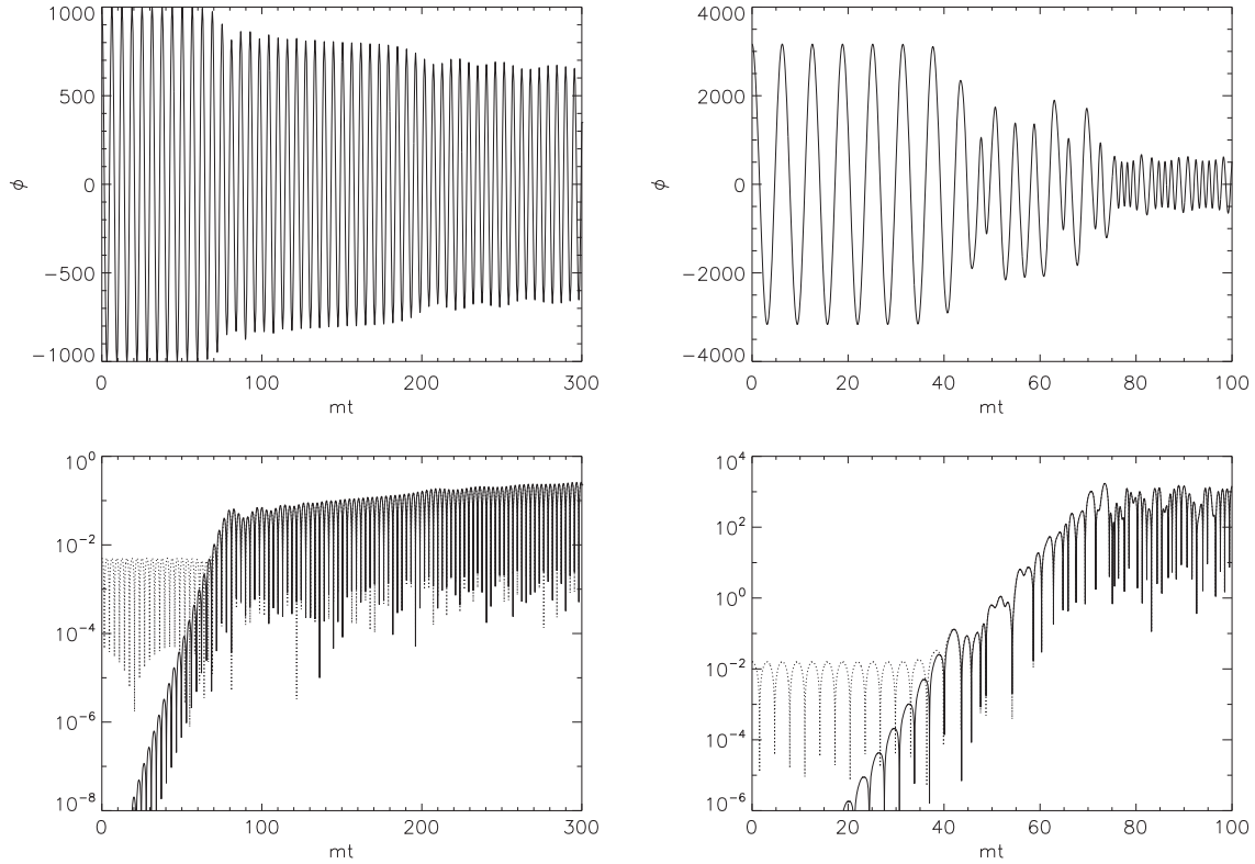
FIG. 2. Numerical solutions to the full set of equations (1) are shown for the inflaton field \phi in the upper panels. In the lower panels |\delta\phi_e| (dashed curves) and |\delta\phi_c| (solid curves) are plotted. For each plot g = 10^{-3} . For the upper left panel g^2\phi_0^2 = 1 and the upper right one g^2\phi_0^2 = 10 . In the lower left panel \delta\phi_e is the difference between solutions to (1) with g^2\phi_0^2 = 1 + 10^{-5} and g^2\phi_0^2 = 1 . In the lower right panel \delta\phi_e is the difference between solutions to (1) with g^2\phi_0^2 = 10(1 + 10^{-5}) and g^2\phi_0^2 = 10 .
