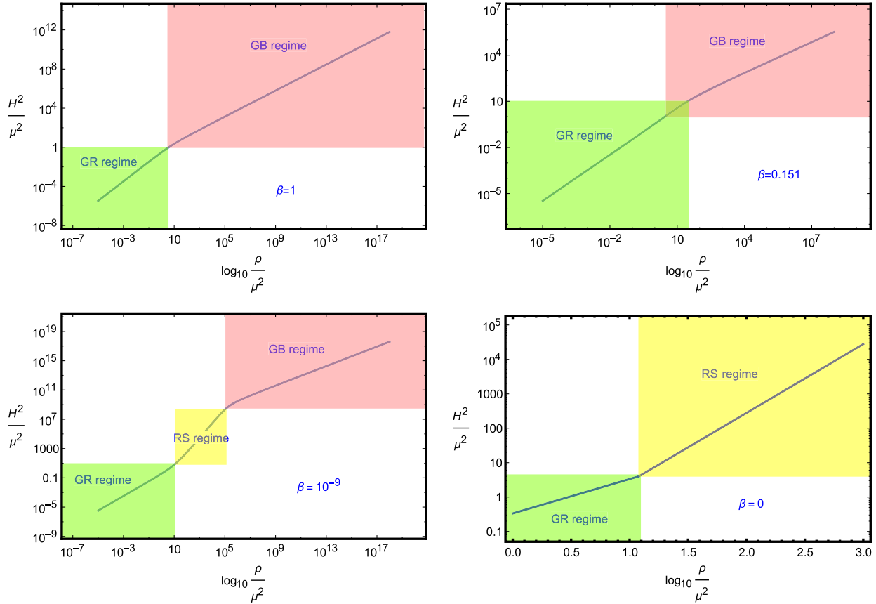
FIG. 1 (color online). The evolution of brane universe with different choices of \beta . The vertical and horizontal axis describe the inflationary Hubble scale H^2/\mu^2 and energy density scale \rho/\mu^2 on the brane, respectively, for a given extra dimension scale \mu . With decreasing \beta from 1 to 0, the GB regime is pushed toward to even higher energy scale and the RS regime grows slowly to finally dominate after its emergence when GB energy scale finally wins over the RS energy scale.
