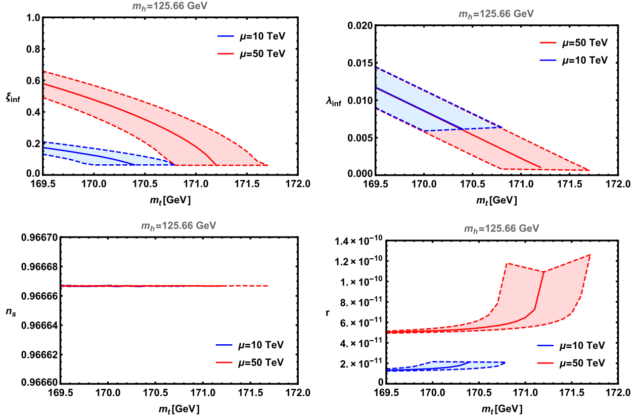
FIG. 5 (color online). Numerical results of nonminimal coupling \xi_{\text{inf}} , Higgs quartic coupling \lambda_{\text{inf}} , scalar spectral index n_s and tensor-to-scalar ratio r during inflation with respect to the top quark mass assuming the Higgs mass m_h = 125.66 GeV. The extra dimension scale is 10 TeV for the blue region and 50 TeV for the red region respectively, where the 1\sigma uncertainties are mainly from strong coupling \alpha_s along with other theoretical uncertainties from the threshold corrections.
