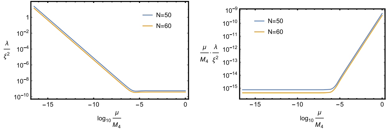
FIG. 3 (color online). The prediction of combined parameter \frac{\lambda}{\xi^2} for Higgs inflation with respect to the energy scale \mu of extra dimension in the Gauss-Bonnet braneworld. For \mu larger than 10^{12} GeV, \frac{\lambda}{\xi^2} remains constant around 10^{-10} as in the four-dimensional case. For \mu smaller than 10^{12} GeV, \frac{\lambda}{\xi^2} increases significantly but the product \frac{\mu}{M_4} \frac{\lambda}{\xi^2} remains constant around 10^{-16} . For \mu around TeV scale, \frac{\lambda}{\xi^2} is of order \mathcal{O}(0.1) , which can lead to a naturally small \xi \sim \mathcal{O}(1) for \lambda \sim \mathcal{O}(0.1) .
