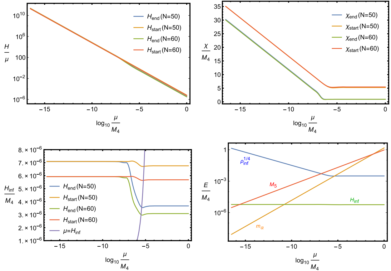
FIG. 2 (color online). The characteristic features of Higgs inflation with respect to the energy scale \mu of extra dimension in the Gauss-Bonnet braneworld. In the first panel, GR regime with \frac{H}{\mu} \ll 1 is found for \mu \gtrsim 10^{12} GeV and GB regime with \frac{H}{\mu} \gg 1 is found for \mu \lesssim 10^{12} GeV. In the second panel, the field values at the start/end point of inflation remain constant in the GR regime but increase significantly in the GB regime. However, the field excursion of inflation is about 5M_4 for all \mu . In the third panel, the inflationary Hubble scales are shown with respect to the extra dimension scale. In the left hand side of purple line where the inflationary Hubble scale equals to the extra dimension scale, the extra dimension scale appears below the inflationary Hubble scale. In the last panel, we summarize several typical energy scales with respect to the extra dimension scale.
