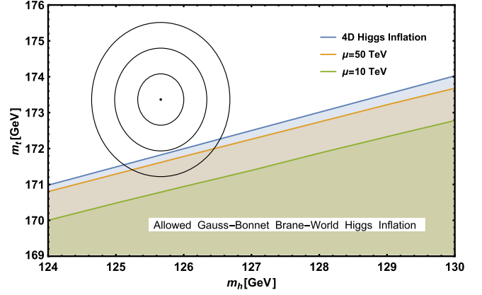
FIG. 6 (color online). The upper bound of top quark mass m_t as a function of Higgs mass m_h where we have taken into account the 1\sigma uncertainties from strong coupling \alpha_s along with other theoretical uncertainties from the threshold corrections. As comparisons, we also provide the upper bound set by four-dimensional Higgs inflation and the experimental constraint on m_t and m_h .
