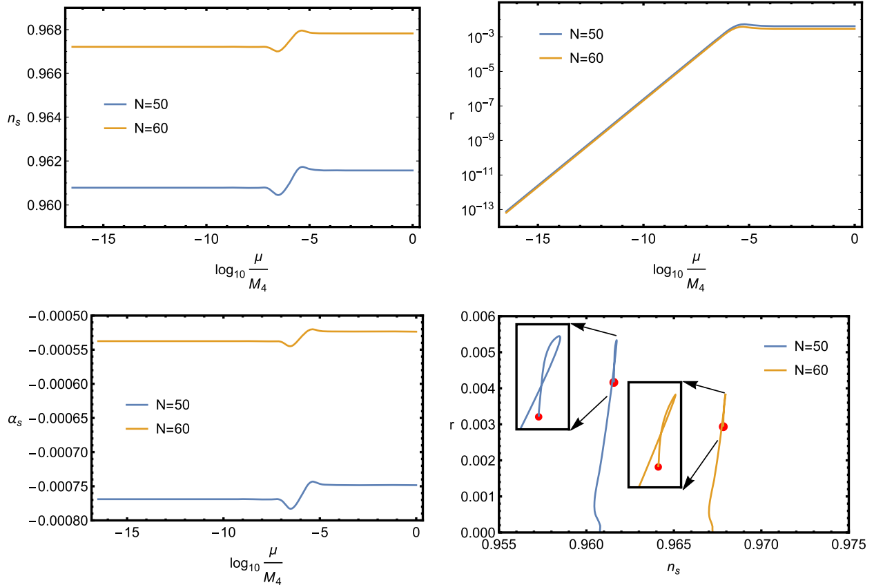
FIG. 4 (color online). Inflationary predictions for Higgs inflation in the Gauss-Bonnet braneworld. The first three panels show the predictions of scalar spectral index n_s , tensor-to-scalar ratio r , and the running of scalar spectral index \alpha_s with respect to the energy scale \mu of extra dimension. With decreasing \mu , r drops significantly while n_s and \alpha_s remain almost the same as in the four-dimensional case. In the last panel, the inflationary predictions of n_s and r are showed in the n_s - r plane, where the red points represent the case of four-dimensional Higgs inflation.
