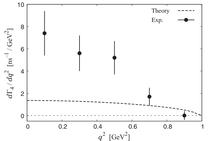
FIG. 7. Differential decay width of the D_s^+ \rightarrow f_0(980)e^+\nu_e decay mode followed by f_0(980) \rightarrow \pi^+\pi^- , with q^2 = [M_{\text{inv}}^{(l\nu)}]^2 . The experimental data are taken from Ref. [27]. The experimental points should be rescaled dividing by about a factor of two if the absolute rate for the f_0(980) production of the reanalysis of Ref. [47] were used.
