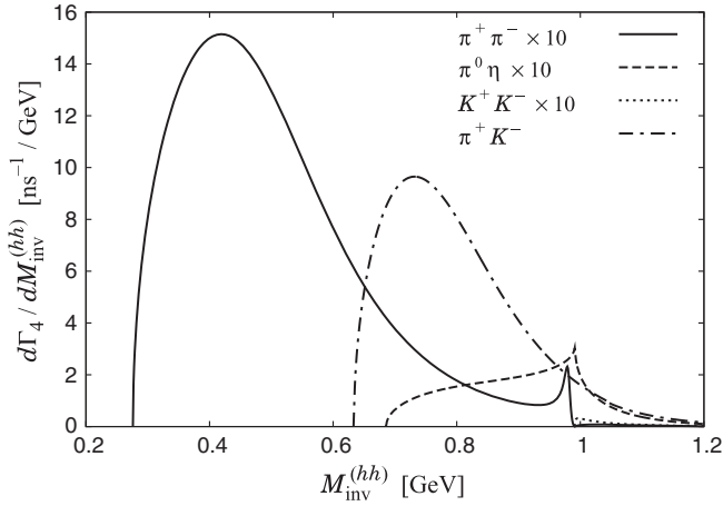
FIG. 4. Meson-meson invariant mass distributions for the semileptonic decay D^+ \rightarrow PP e^+ \nu_e with PP = \pi^+ \pi^-, \pi^0 \eta, K^+ K^-, and \pi^+ K^- in s wave. We multiply the \pi^+ \pi^-, \pi^0 \eta, and K^+ K^- mass distributions, which are Cabibbo-suppressed processes, by 10.
