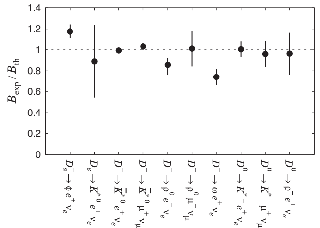
FIG. 8. Ratio of the experimental to theoretical branching fractions for the semileptonic D decays into vector mesons.
