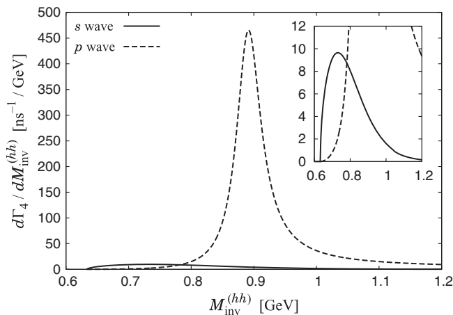
FIG. 11. \pi^+K^- invariant mass distribution for the semileptonic decay D^+ \rightarrow \pi^+K^-e^+\nu_e both in s and p waves.
