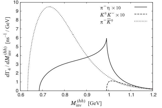
FIG. 5. Meson-meson invariant mass distributions for the semileptonic decay D^0 \rightarrow PP e^+ \nu_e with PP = \pi^- \eta, K^0 K^-, and \pi^- \bar{K}^0 in s wave. We multiply the \pi^- \eta and K^0 K^- mass distributions, which are Cabibbo-suppressed processes, by 10.
