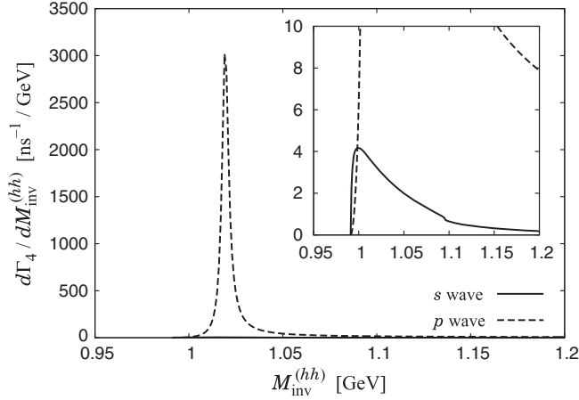
FIG. 10. K^+K^- invariant mass distribution for the semileptonic decay D_s^+ \rightarrow K^+K^-e^+\nu_e both in s and p waves.
