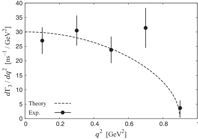
FIG. 9. Differential decay width of the D_s^+ \rightarrow \phi(1020)e^+\nu_e decay mode followed by \phi(1020) \rightarrow K^+K^- , with q^2 = [M_{\text{inv}}^{(\nu)}]^2 . The experimental data are taken from Ref. [27]. The theoretical value is multiplied by the branching fraction of the \phi(1020) meson to K^+K^- , \mathcal{B}[\phi(1020) \rightarrow K^+K^-] = 48.9\% [1].
