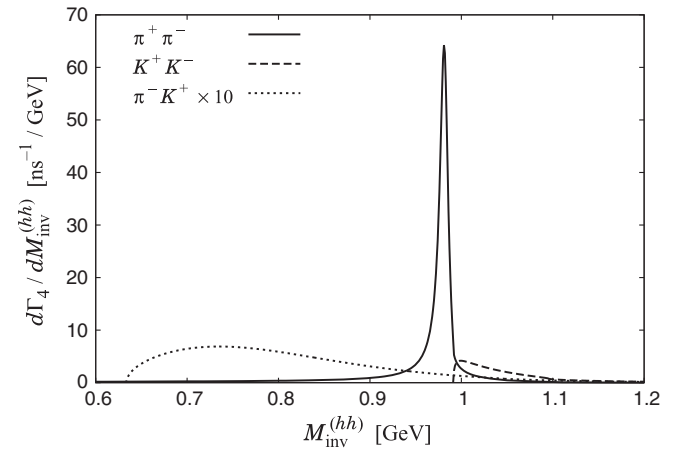
FIG. 3. Meson-meson invariant mass distributions for the semileptonic decay D_s^+ \rightarrow PP e^+ \nu_e with PP = \pi^+ \pi^-, K^+ K^-, and \pi^- K^+ in s wave. We multiply the \pi^- K^+ mass distribution, which is a Cabibbo-suppressed process, by 10.
