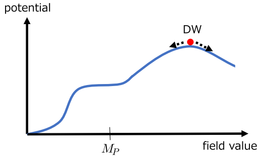
FIG. 10 (color online). Schematic figure for the maximum that yields the domain wall, which becomes the source for the eternal inflation.
