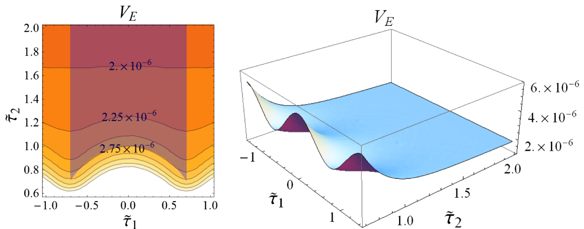
FIG. 7 (color online). Contour and 3D plots are shown in the left and right panels, respectively, for the energy density V_E in the Einstein frame as a function of \tilde{\tau}_1 = rA/\sqrt{\alpha'} and \tilde{\tau}_2 = r/\sqrt{\alpha'} , with all their values being given in \alpha' = 1 units. The shaded fundamental region and the existence of the \sqrt{2} -shift are the same as in Fig. 6. We see that the potential becomes runaway for the large radius limit r \gg \sqrt{\alpha'} .
