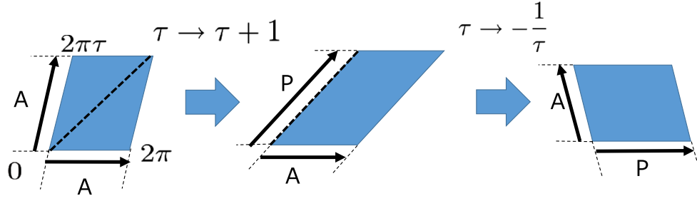
FIG. 14 (color online). A and P denote the antiperiodic and periodic boundary conditions, respectively. The horizontal direction is the spatial one, \sigma . Given the all-A boundary condition for both the time and spatial directions, the modular invariance necessitates the all-P boundary condition for the time or spatial direction.
