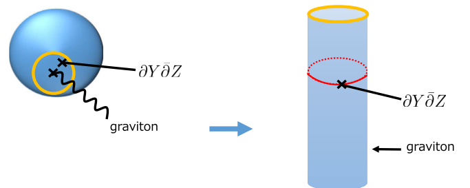
FIG. 4 (color online). Left: The Higgs emission vertex \partial Y \bar{\partial} Z is single-valued around the graviton emission vertex because Y and Z are independent of the spacetime coordinate X^\mu . Right: Exponential mapping around the graviton emission vertex. \partial Y and \bar{\partial} Z are periodic around the cylinder, e.g. around the (red) circle.
