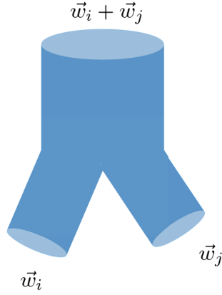
FIG. 15 (color online). Schematic picture for the string interaction joining \vec{w}_i and \vec{w}_j strings to make \vec{w}_i + \vec{w}_j string. If there exist the sets of boundary conditions \vec{w}_i and \vec{w}_j , then there must be \vec{w}_i + \vec{w}_j in W .
