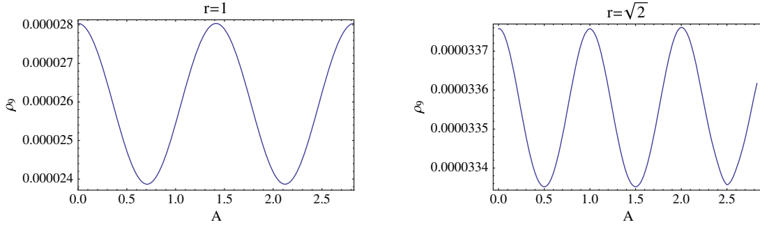
FIG. 5 (color online). The potential \rho_9 in Jordan frame as a function of A with r = \sqrt{\alpha'} (left) and \sqrt{2\alpha'} (right), all in units of \alpha' = 1 . We can see the periodicity A \rightarrow A + \sqrt{2\alpha'}/r , up to the distortions due to numerical errors.
