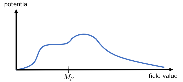
FIG. 11 (color online). Schematic figure for the Higgs potential smoothly connected to the runaway direction.
