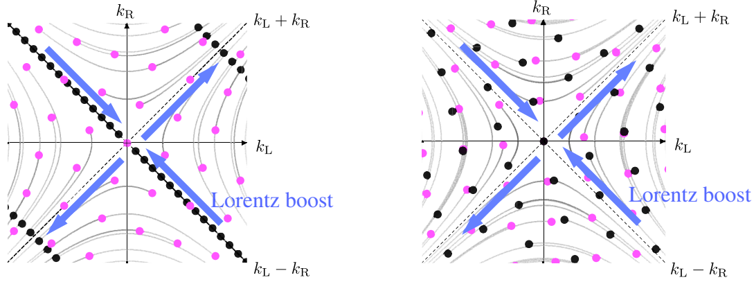
FIG. 3 (color online). Schematic picture of the momentum boost in the k_R vs k_L plane. The light cone in the momentum space is depicted by the dashed diagonal lines. The sets of lighter (magenta) and black dots represent the initial momentum lattice and the one after the boost, respectively. Left: There exists a point of the initial lattice on the light cone. Then there exist infinite amount of its integer multiplications on the light cone. In the infinite boost limit, they are contracted to form a decompactified dimension, which is represented by the black dots. Right: There is no initial point on the light cone, and such a decompactification does not occur.
