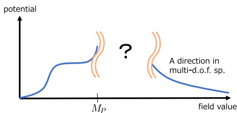
FIG. 9 (color online). Schematic figure for the Higgs potential. Low energy side is determined phenomenologically. High energy side represents a runaway direction in the multidegrees of freedom space.
