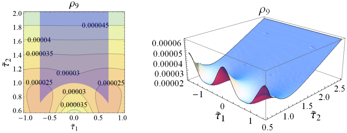
FIG. 6 (color online). Contour and 3D plots are shown in the left and right panels, respectively, for the energy density \rho_9 in the Jordan frame as a function of \tilde{\tau}_1 = rA/\sqrt{\alpha'} and \tilde{\tau}_2 = r/\sqrt{\alpha'} , with all their values being given in \alpha' = 1 units. In the left, we shade the fundamental region for the T-dual transformation: |\tau_1| \leq 1/\sqrt{2} , |\tau_2| \geq 1 . We can see the shift-symmetry \tilde{\tau}_1 \rightarrow \tilde{\tau}_1 + \sqrt{2} , up to distortions due to numerical errors.
