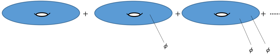
FIG. 2 (color online). Partition function under the presence of the background \phi . Summing up all the possible insertions of \phi , it exponentiates to yield Eq. (6). This picture shows the one-loop case.
