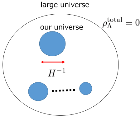
FIG. 13 (color online). Universe is divided into parts that will eventually become causally disconnected to each other in the end of their histories.
