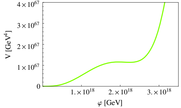
FIG. 1 (color online). The SM Higgs potential V as a function of the Higgs field \varphi . Here we take M_H = 125 GeV and tune the top mass in such a way that the potential becomes flat; see e.g. Ref. [65].
