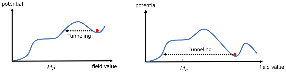
FIG. 12 (color online). Schematic figure for the Higgs potential. On the left, the false vacuum has higher energy than the quasiflat potential in the SM, while on the right, it has lower energy.
