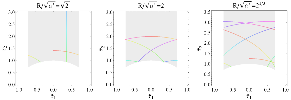
FIG. 8 (color online). The trajectory that starts from \eta = 0 at (\tilde{\tau}_1, \tilde{\tau}_2) = (0, R/\sqrt{\alpha'}) for a fixed value of R/\sqrt{\alpha'} being \sqrt{2} , 2, and 2^{1/3} in the left, center, and right panels, respectively, showing the runaway, periodic, and chaotic limits. We have shaded the fundamental region for the T-dual transformations.
