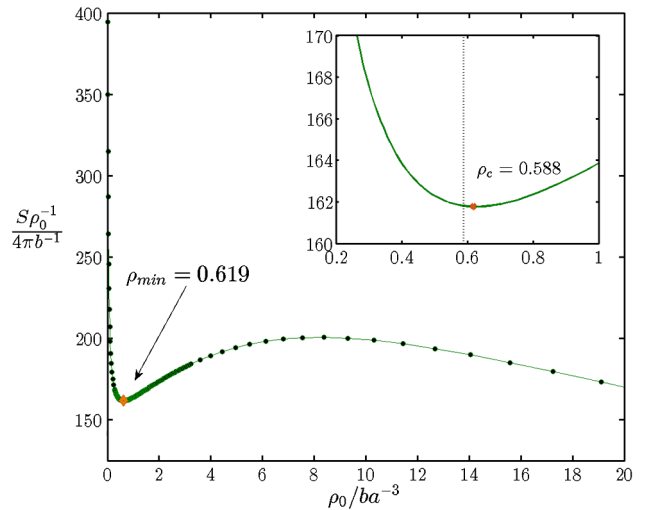
FIG. 7 (color online). Configurational entropy times \rho_0^{-1} for the OV neutron star vs central density \rho_0 . Stars with \rho_0 > \rho_c = 0.588ba^{-3} are perturbatively unstable to gravitational collapse. The inset shows the result near the CE minimum.
