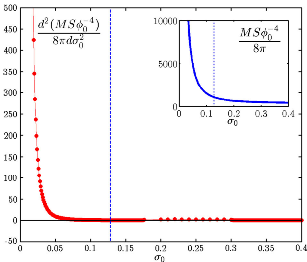
FIG. 12 (color online). The inset shows the quantity S\phi_0^{-4}M as a function of the scalar field's central value \sigma_0 for \Lambda = 100 . The main plot shows the second derivative of S\phi_0^{-4}M with respect to \sigma_0 , displaying the same saddle ridge behavior found for polytropes.
