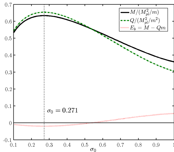
FIG. 9 (color online). Boson star mass (continuous line) and conserved charge Q (dot-dashed line) vs central value of the scalar field \sigma_0 . We also show the binding energy E_b (dotted line). Stars with \sigma_0 > \sigma_c = 0.271 are known to be unstable to gravitational collapse.
