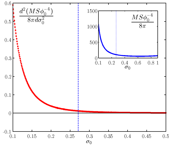
FIG. 11 (color online). The inset shows the quantity S\phi_0^{-4}M as a function of the scalar field's central value \sigma_0 for \Lambda = 0 . The main plot shows the second derivative of S\phi_0^{-4}M with respect to \sigma_0 , displaying the same saddle ridge behavior found for polytropes.
