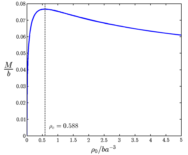
FIG. 6 (color online). OV neutron star mass vs central density \rho_0 . Stars with \rho_0 > \rho_c = 0.588ba^{-3} are known to be unstable to gravitational collapse.
