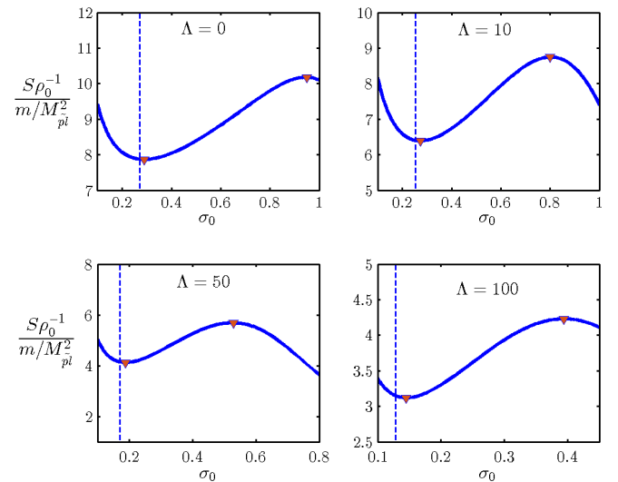
FIG. 10 (color online). The configurational entropy for boson stars multiplied by inverse central density S\rho_0^{-1} as a function of the scalar field's central value \sigma_0 for different values of the scalar field self coupling \Lambda . The dashed vertical line denotes \sigma_c , the instability boundary for the star under radial perturbations. As in the case with neutron stars, the CE provides a reliable estimate for the critical mass, with precision better than \sim 1\% . Values of maximum stellar masses for different values of \Lambda are listed in Table I.
