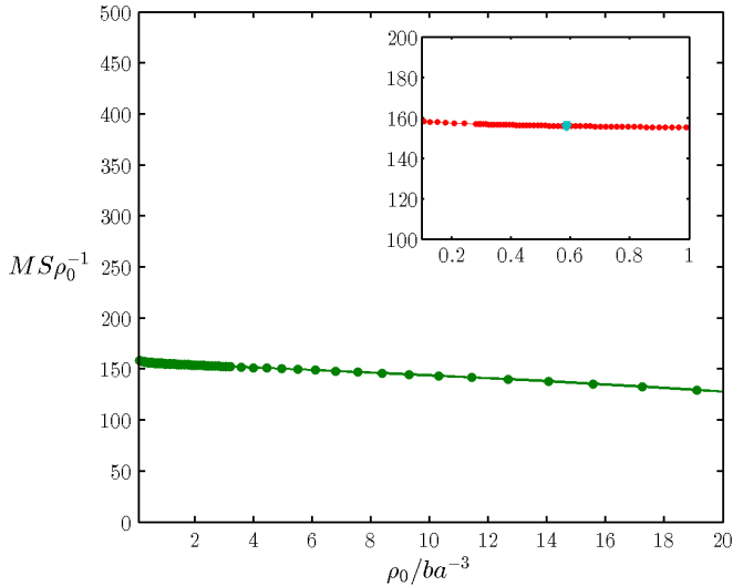
FIG. 8 (color online). Behavior of the quantity S\rho_0^{-1}M as a function of central density \rho_0 for OV neutron stars. The approximate linear scaling persists for a wide range of central densities. The inset shows the result near \rho_c = 0.588ba^{-3} , the critical value for stability.
