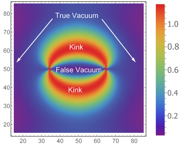
FIG. 2 (color online). The action density of the confining string \bar{\sigma} obtained by numerically minimizing, via Gauss-Seidel relaxation, the action (1) with the correct monodromies. The lattice has spacing 1/M , size 100 \times 100 , and M/m = 20 . The classical \log R growth of the transverse separation from the model of Fig. 1 is also seen to hold upon studying different size strings.
