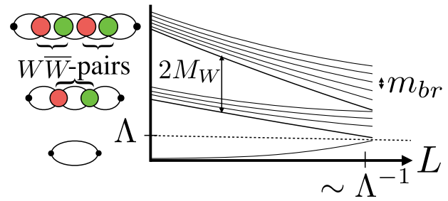
FIG. 4 (color online). A sketch of the Abelian string spectrum, corresponding to the tower of W\bar{W} -boson pairs attached to the double string, and the breather mode excitations m_{br} .
