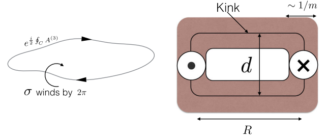
FIG. 1 (color online). Left: the Wilson loop and the monodromy of \sigma . Right: Sketch of the confining string configuration \bar{\sigma} with the correct monodromy, composed of two domain walls. The dot and cross represent probe quarks a distance R apart. The maximum distance between the walls, of thickness 1/m , is d .
