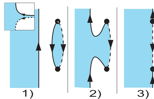
FIG. 3 (color online). A sketch of how a q\bar{q} pair can fuse into the DW (from left to right). The shaded and white regions represent distinct vacua of the theory. The solid black line represents the BPS_1 DW, while the dashed line represents the anti- BPS_2 DW, while the arrows represent their electric fluxes. The black dots are the quark and the antiquark. The inlay in the upper left corner shows a fundamental string ending on a DW.
