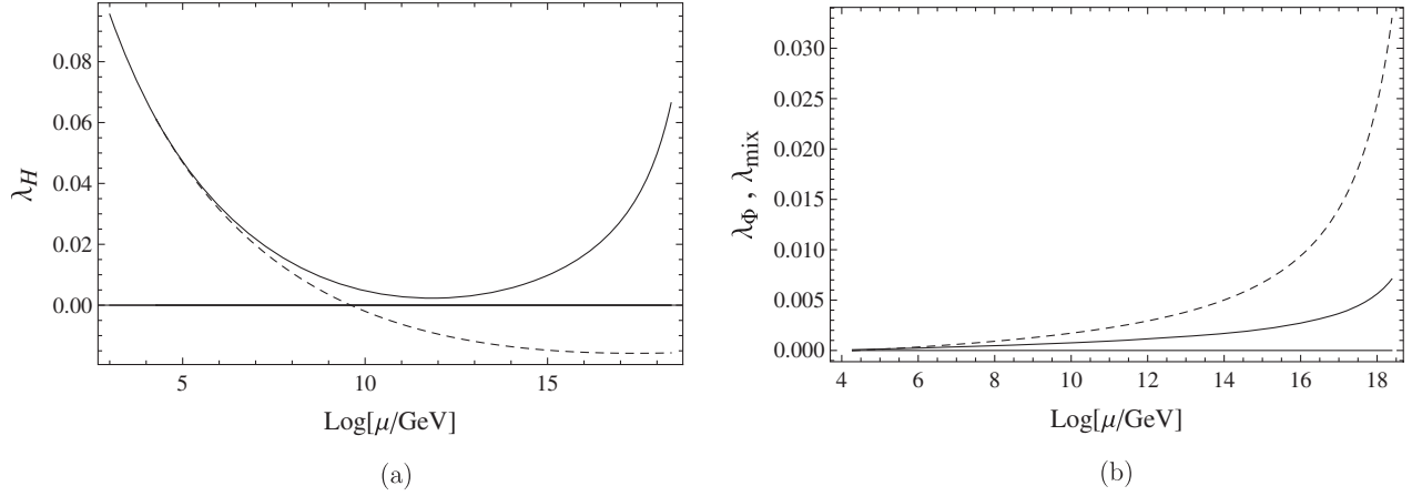
FIG. 1. (a) The evolutions of the Higgs quartic coupling \lambda_H (solid line) for the inputs m_t = 173.34 GeV and m_h = 125.03 GeV, along with the SM case (dashed line). (b) The RG evolutions of \lambda_\Phi (solid line) and \lambda_{\text{mix}} (dashed line). Here, we have taken x_H = 2 , v_\phi = 19 TeV and g'(v_\phi) = 0.09 .
