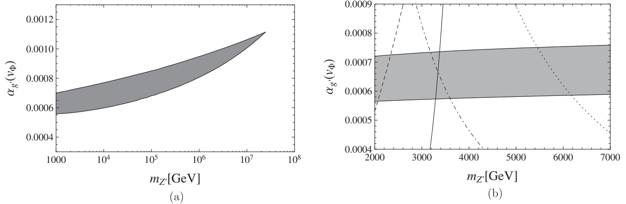
FIG. 3. (a) The result of parameter scan for v_\phi and g' with a fixed x_H = 2 , shown in (m_{Z'}, \alpha_{g'}) -plane. (b) The allowed region at the TeV scale in (a) is magnified, along with the LEP bound (dashed line) and the LHC bound (solid line) from direct search for Z' boson resonance. The region on the left side of the lines are excluded. Here, the naturalness bounds for 10% (dotted line) and 30% (dashed-dotted line) fine-tuning levels are also depicted.
