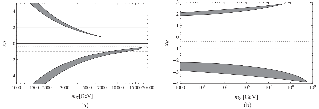
FIG. 2. (a) The result of parameter scan for x_H and g' with a fixed v_\phi = 19 TeV, shown in (m_{Z'}, x_H) -plane with m_{Z'} = \sqrt{(x_\Phi g' v_\phi)^2 + (x_H g' v_h)^2} \approx x_\Phi g' v_\phi . As a reference, horizontal lines are depicted for x_H = 2, 0 [ \text{U}(1)_{B-L} case], -16/41 [orthogonal case], and -1 [ \text{U}(1)_R case]. (b) Same as (a), but parameter scan for x_H and v_\phi with a fixed g' = 0.09 .
