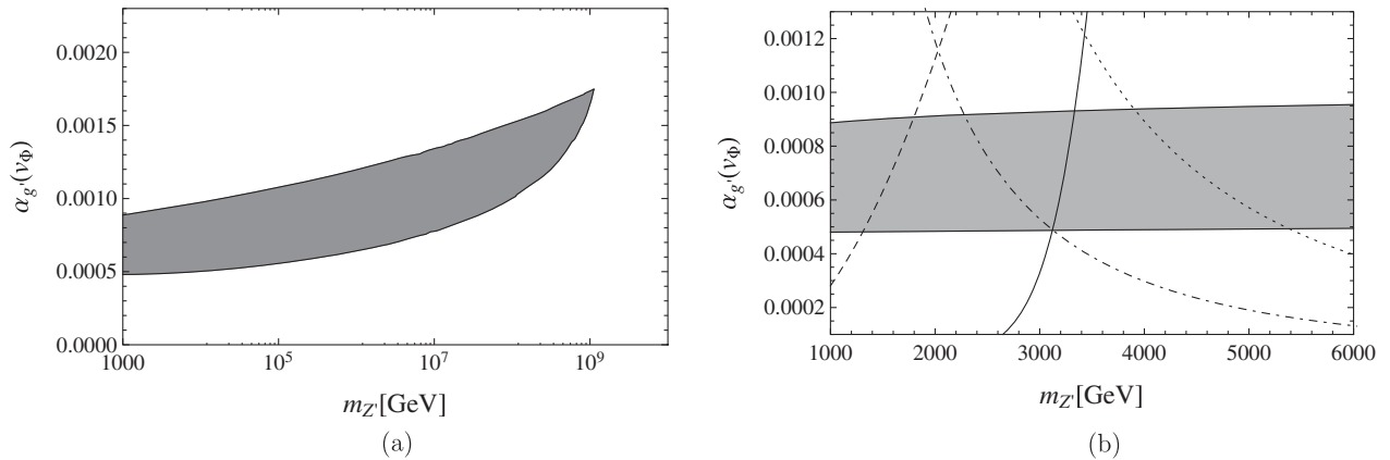
FIG. 4. (a) Same as Fig. 3(a), but for x_H = -2.5 . (b) Same as Fig. 3(b), but for x_H = -2.5
