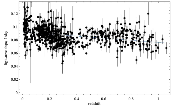
FIG. 2 (color online). The light-curve slope \lambda versus the redshift z for the sample of supernovae considered in this work.
