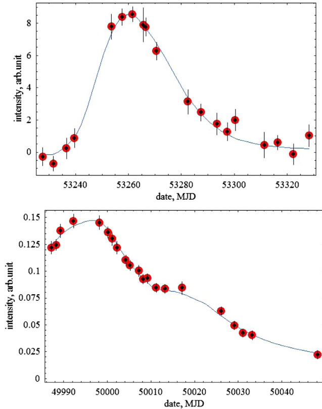
FIG. 1 (color online). Example light curves in the R band: SNLS-04D1hy ( z = 0.85 ; top panel) and SN 1995ac ( z = 0.049 ; bottom panel). The lines represent best fits obtained using redshift-corrected templates.
