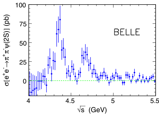
FIG. 11 (color online). The measured e^+e^- \rightarrow \pi^+\pi^-\psi(2S) cross section for \sqrt{s} = 4.0 to 5.5 GeV. The errors are the sum in quadrature of the summed statistical errors of the numbers of signal and background events and the systematic errors.
