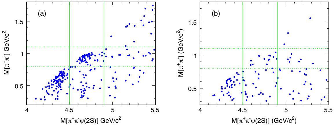
FIG. 3 (color online). Invariant mass of the \pi^+\pi^- recoiling against the \psi(2S) versus the invariant mass of the \pi^+\pi^-\psi(2S) in the \pi^+\pi^-J/\psi mode (a) and \mu^+\mu^- mode (b). The horizontal dashed lines show the belt of f_0(980) , while the vertical solid lines demarcate the regions with the Y(4360) and Y(4660) states and the higher-mass combinations.
