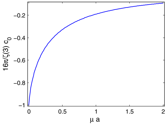
FIG. 1 (color online). Coefficient 16\pi c_0/\zeta(3) as a function of \mu a .
