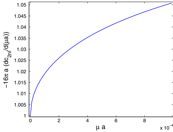
FIG. 3 (color online). Logarithmic derivative -16\pi\mu a dc_{2nl}/d\mu a as a function of \mu a .
