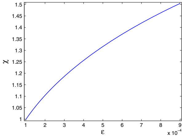
FIG. 4 (color online). \chi (55) as a function of \epsilon = a/R (circle-line geometry) for \mu R = 0.1 . \chi goes to 1 for small values of \epsilon , showing that the NTLO correction in this case is similar to the one of the parabola-line configuration.
