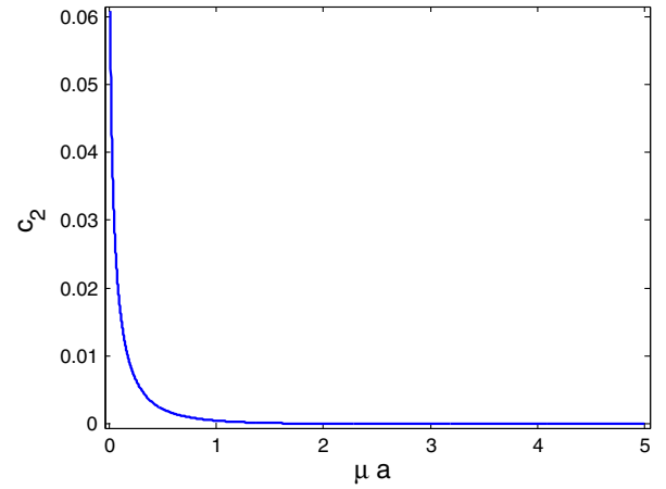
FIG. 2 (color online). Coefficient c_2 as a function of \mu a .
