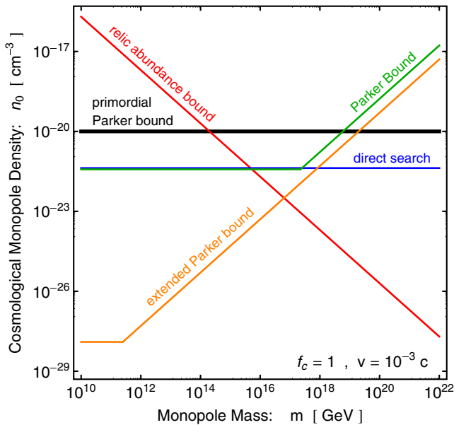
FIG. 1 (color online). A summary of upper bounds on the magnetic monopole abundance from this work and the literature. Black : the requirement of survival of the primordial magnetic field (‘‘primordial Parker bound’’), derived here in Eq. (16). Red : the cosmological abundance bound in Eq. (1). Blue : direct search constraints [36] (see the magnetic monopole review). Green : the requirement of survival of the Galactic magnetic field (Parker bound), given by Ref. [37]. Orange : the requirement of survival of the Galactic seed field (‘‘extended Parker bound’’), given by Ref. [38]. We take v \approx 10^{-3} and assume that monopoles are unclustered, f_c \approx 1 . If the monopoles are clustered then the Parker bound, extended Parker bound, and direct search limits move down by a factor of f_c \sim 10^5 .
