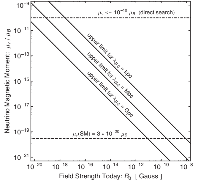
FIG. 2. The requirement that spin-flip transitions are out of equilibrium at the QCD epoch leads to an upper bound the neutrino magnetic moment given by Eq. (64).
