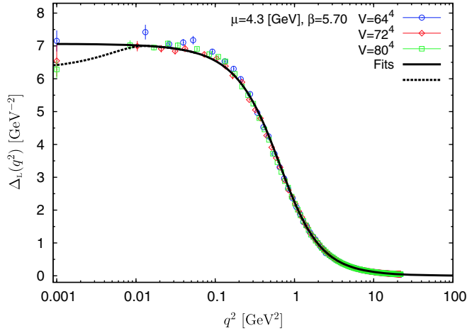
FIG. 2 (color online). The lattice SU(3) gluon propagator evaluated in the Landau gauge [4] and the corresponding fit used in our calculation [27]. The dashed curve shows a fit featuring an IR maximum which is due to the presence of (divergent) contributions to the gluon (inverse) dressing function [42]. All functions are renormalized at \mu = 4.3 GeV.
