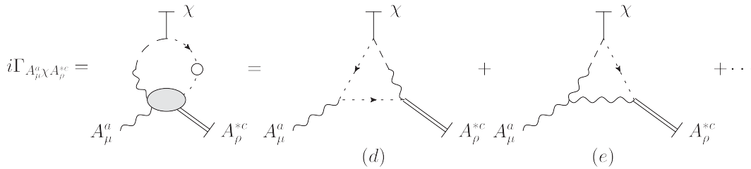
FIG. 6. One-loop diagrams contributing to the auxiliary function \Gamma_{A_\mu \chi A_\nu^c} appearing in the gluon two-point Nielsen identity (3.12).
