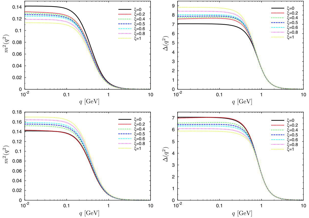
FIG. 8 (color online). \xi -dependence of the gluon mass (left panels) and gluon propagator (right panels) as predicted by the Ansatz (3.20) for a_1 = -0.2 (upper panels) and a_1 = 0.2 (lower panels).
