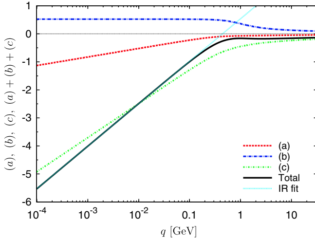
FIG. 5 (color online). Contributions of the one-loop dressed auxiliary functions to the ghost two-point function Nielsen identity. The IR region is perfectly described by the predicted c_{\text{NI}} \log q^2/\mu^2 behavior yielding c_{\text{NI}} = 0.33 .
