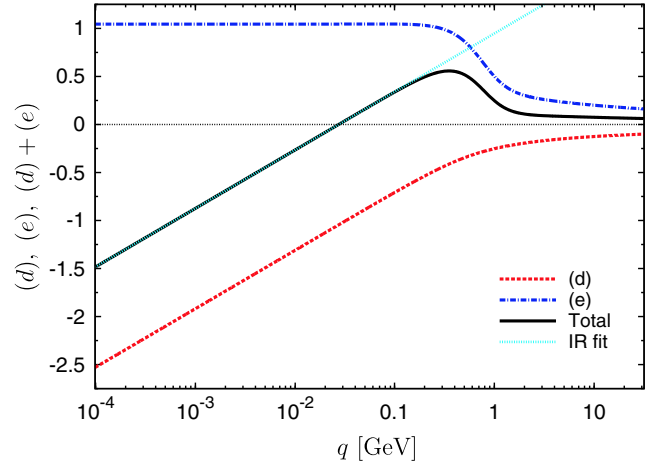
FIG. 7 (color online). Contributions of the one-loop dressed auxiliary functions to the gluon two-point function Nielsen identity. Also in the gluon case the IR region is perfectly described by the predicted b \log q^2/\mu^2 behavior, now with c_{\text{NI}} = 0.13 .
