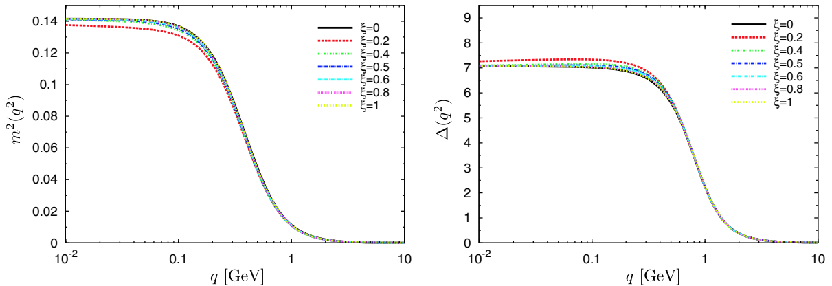
FIG. 9 (color online). \xi -dependence of the gluon mass (left) and gluon propagator (right) as predicted by the Ansatz (3.20) for a_1 = 0 .
