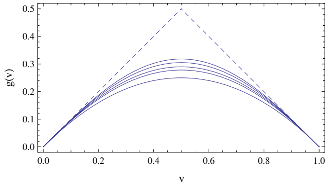
FIG. 2 (color online). The functions g(v) in the expression for the modular Hamiltonian of the null slab, for conformal field theories with a bulk dual. Here d = 2, 3, 4, 8, \infty from bottom to top. Near the boundaries ( v \rightarrow 0 , v \rightarrow 1 ), we find g \rightarrow 0 , g' \rightarrow \pm 1 , in agreement with the modular Hamiltonian of a Rindler wedge. We also note that the functions are concave (see Sec. IV). In particular, we see that |g'| \leq 1 , in agreement with our general argument of Sec. III.
