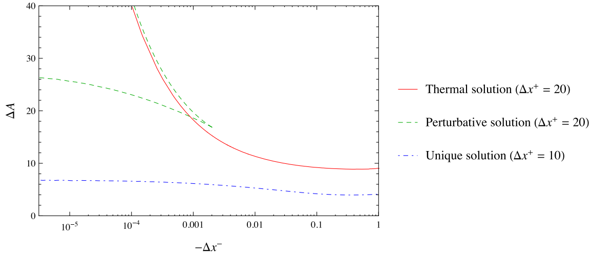
FIG. 6 (color online). The vacuum-subtracted extremal surface area versus \Delta x^- for fixed \Delta x^+ ( \Delta x^+ = 20 and \Delta x^+ = 10 for d = 3 is shown). This numerical simulation demonstrates that, for sufficiently large \Delta x^+ (in d = 3 , the condition is \Delta x^+ \gtrsim 15 ), there exists a phase transition at finite \Delta x^- to a different, perturbative class of solutions. At smaller \Delta x^+ , there is no such phase transition.
