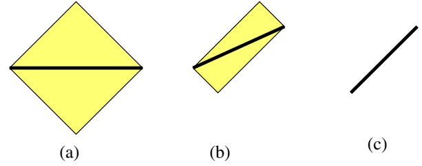
FIG. 3 (color online). Operator algebras associated to various regions. (a) Operator algebra associated to the domain of dependence (yellow) of a spacelike interval. (b) The domain of dependence of a boosted interval. (c) In the null limit, the domain of dependence degenerates to the interval itself.
