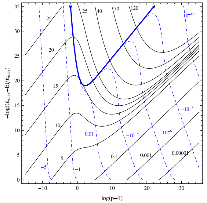
FIG. 5 (color online). Curves of constant \Delta x^+ (black solid curves) and \Delta x^- (blue dashed curves), in the logarithmic parameter space defined by (\log(p - 1), -\log(E_{\max}(p) - E)/E_{\max}(p)) . The value p = 1 maps to -\infty and p = \infty maps to +\infty on the horizontal axis, while E = 0 maps to 0 and E = E_{\max}(p) maps to +\infty on the vertical axis. The thick blue contour represents the null solutions with \Delta x^- = 0 . Above this contour, the boundary interval is timelike. If \Delta x^+ \gtrsim 15 and we follow a contour of constant \Delta x^+ , we find two solutions with exact \Delta x^- = 0 . For all contours of fixed \Delta x^+ , there exists an asymptotic null solution in the limit p \rightarrow \infty .
