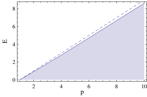
FIG. 4 (color online). The maximum value E_{\max}(p) of E for getting a surface that returns to the boundary (solid line). For comparison, we also plotted the line E = p - 1 (dashed line). The extremal surface solutions of interest appear in the region p > 1 , 0 < E < E_{\max}(p) . Here, we have taken d = 3 .
