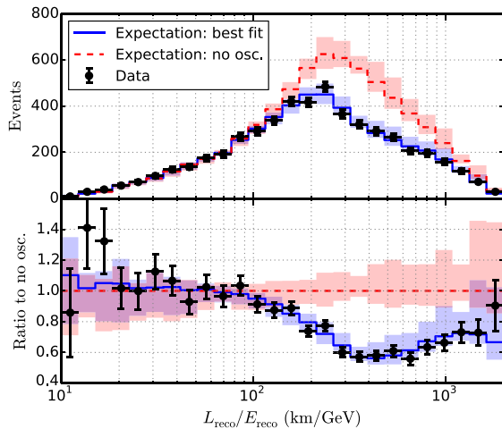
FIG. 6 (color online). Distribution of events as a function of reconstructed L/E . Data are compared to the best fit and expectation with no oscillations (top), and the ratio of data and best fit to the expectation without oscillations is also shown (bottom). Bands indicate estimated systematic uncertainties.
