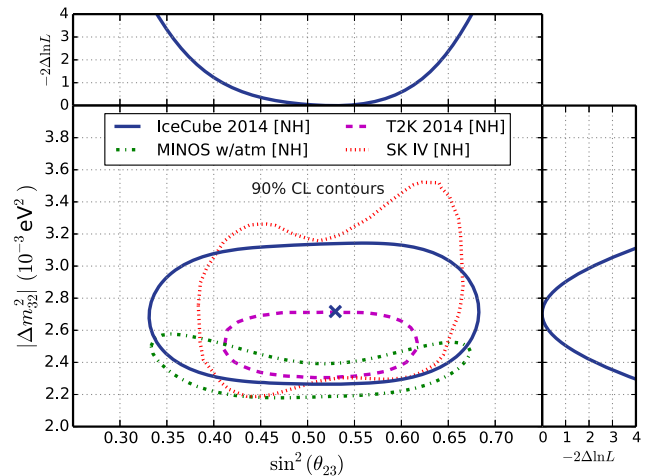
FIG. 7 (color online). 90% confidence contours of the result in the \sin^2 \theta_{23} - \Delta m^2_{32} plane in comparison with the ones of the most sensitive experiments [8–10]. The log-likelihood profiles for individual oscillation parameters are also shown (right and top). A normal mass ordering is assumed.
