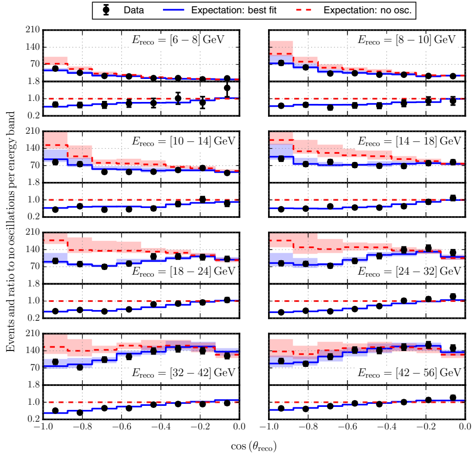
FIG. 5 (color online). Comparison between data and expectations for the case of oscillations and no oscillations. In each figure the zenith distribution for an energy band is shown (top), and the ratio of the data and the best fit to no oscillations is shown (bottom). The binning corresponds to that used for obtaining the best-fit oscillation parameters. Bands indicate the impact of the assumed systematic uncertainties.
