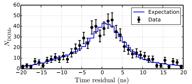
FIG. 3 (color online). Difference in arrival time between direct photons and the expected hyperbola from the track fit, comparing simulation with 5% of the final data sample.
