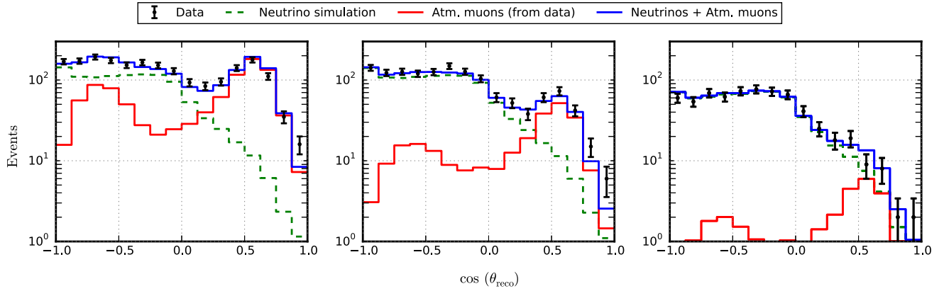
FIG. 2 (color online). Zenith angle distributions of neutrino simulation and atmospheric muons derived from data for three subsequent steps in the event selection with increasing veto cuts. To go from the first to the second panel the veto cut which uses a muon track hypothesis is applied. A cut on the charge observed above and prior to the trigger is used to go from the second to the third panel. A comparison is also made to a 10% control sample of the data. The small excess in the data around \cos \theta_z \approx 0.3 in the first panel are atmospheric muons that could not be tagged. Note that the region \cos \theta_z > 0 is not used in the final analysis of the data.
