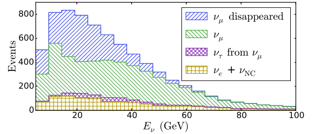
FIG. 4 (color online). True energy distribution of simulated neutrino events in the final sample, with hatched areas representing each component. Only events used for the final result are considered [ E_{\text{reco}} = [6, 56] GeV, and \cos(\theta_{\text{reco}}) < 0 ]. The missing \nu_{\mu} component is also shown.
