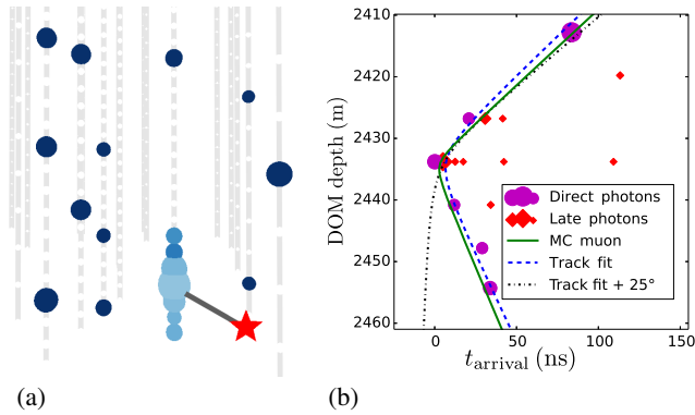
FIG. 1 (color online). A simulated 12 GeV \nu_\mu interacting in DeepCore and producing an 8 GeV muon (42-m range) and a 4 GeV hadronic shower. In (a), the dashed vertical lines are detector strings, the star marks the position of the interaction vertex and the solid line is the muon track. Twenty DOMs record photons; they have colors related to the photon arrival time (lighter is earlier) where their size is proportional to the charge observed. In (b), the DOM depth as a function of the arrival time of photons at the string with most light collected is shown. Marker sizes scale with charge. The expected hyperbolae from simulation, a track fit and the same fit altered by 25^\circ are also shown.
