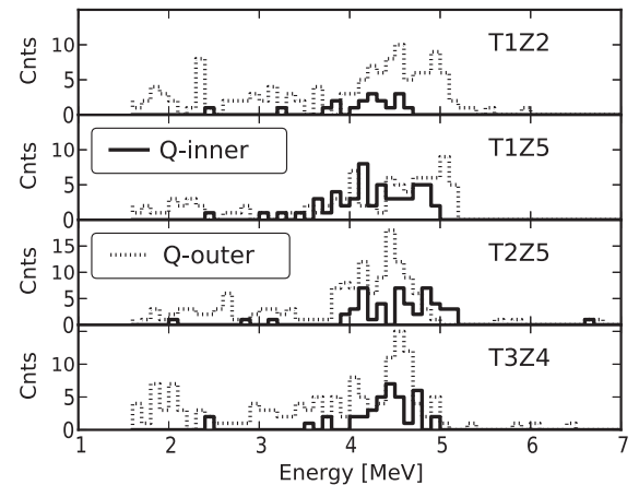
FIG. 8. Spectra of alpha events observed in (from top to bottom) detector T1Z2, T1Z5, T2Z5, and T3Z4. Our analysis assumes that any alpha with energy > 4 MeV is from a ^{210}\text{Po} decay. Shown are alpha events detected on the inner (“Q-inner,” solid) and outer (“Q-outer,” dashed) electrodes. Q-outer events most likely originate from the copper housings.
