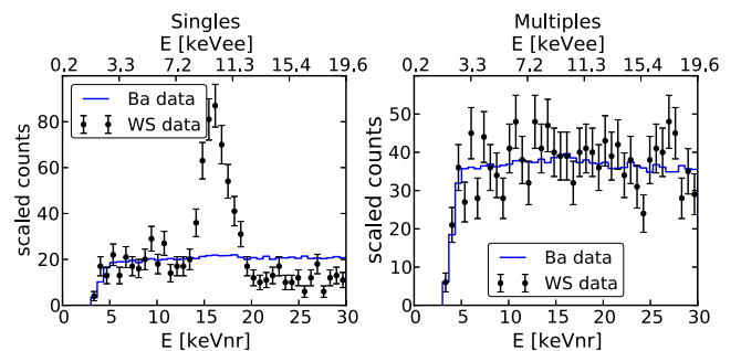
FIG. 3 (color online). WS data and Ba calibration data for events within the ER band for detector T1Z2, given in NR (ER) equivalent phonon energy along the bottom (top) axis. The 10.4 keVee (17 keVnr) Ge activation line is clearly seen in the single-scatter WIMP-search data (left panel) but absent in the Ba calibration and multiple-scatter WIMP-search data (right panel).
