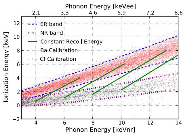
FIG. 1 (color online). Events in the ionization- versus recoil-energy plane for one detector. Events from ^{133}\text{Ba} and ^{252}\text{Cf} calibration data are shown. The recoil-energy scale is given by the total phonon energy minus the Neganov-Luke phonon [5] contribution. The keVnr scale (bottom x axis) gives the correct recoil energy at the center of the NR band, while the keVee scale (top x axis) gives the correct recoil energy at the center of the ER band.
