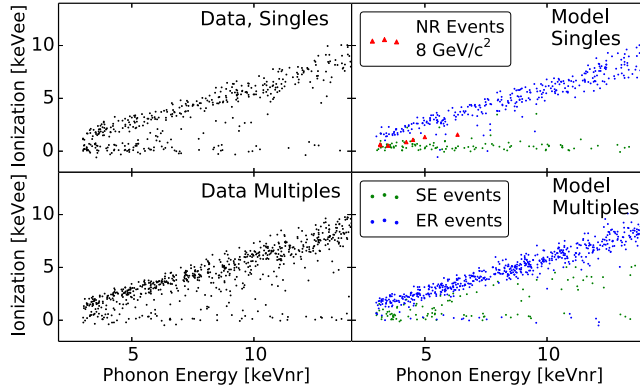
FIG. 10 (color online). A comparison between WIMP-search data (left column) and the background model (right column) for one detector (T1Z2), with a NR component representative of an 8 \text{ GeV}/c^2 WIMP shown with the background-model singles. The number of points displayed for the background model has been reduced to match the number in the WIMP-search data. The likelihood fit is performed in this two-dimensional space of ionization versus phonon energy.
