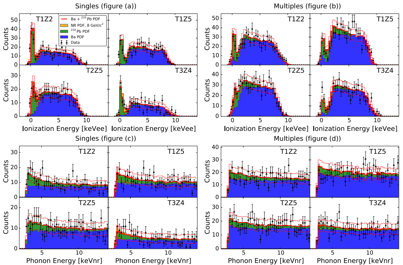
FIG. 9 (color online). Stacked histograms of either phonon or ionization energy. Figures (a) and (c) show the ML best-fit result to WIMP-search data singles, while Figs. (b) and (d) show the ML best fit to WIMP-search data multiples. Figures (a) and (b) show the projection in ionization energy while (c) and (d) show the projection in phonon energy. The four canvases in each figure show the result for each of the four detectors. The combined components of the surface-event background model are represented by the solid green histogram (legend title: ^{210}\text{Pb} PDF), while the gamma-background model is shown in blue (legend title: Ba PDF). The combined probability density functions from simulation and calibration data are shown as the thick line on top of the solid histograms (the thin lines indicate the statistical uncertainties), while the WIMP-search data are shown in black error bars. The orange histogram (legend title: NR PDF) represents the best-fit nuclear recoil-like component. The agreement is good, with T3Z4 having the worst fit of the four detectors caused by two histogram bins after the low-energy peak [Figs. (a) and (b)] which are not fit well. The low-energy peak of that detector in the multiples is also not fit well, which may be a result of miscalibration due to a lack of penetration-depth calibration data for this detector.
