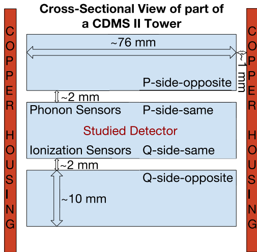
FIG. 2 (color online). A simple detector schematic (not to scale), showing an analyzed detector in the center along with the two neighboring detectors. The detectors are surrounded by copper housings. Detectors had phonon sensors on their top surfaces and ionization sensors on the bottom. Surface events originating from decays on the “studied detector” are named “P-side-same” or “Q-side-same” depending on whether the decay occurred on the phonon or ionization side. In simulations, surface events (SEs) on the studied detector that originate from a decay on a detector adjacent to the studied detector are either named “P-side-opposite” or “Q-side-opposite” depending on whether the decay caused an energy deposition on the phonon or ionization side of the studied detector.
