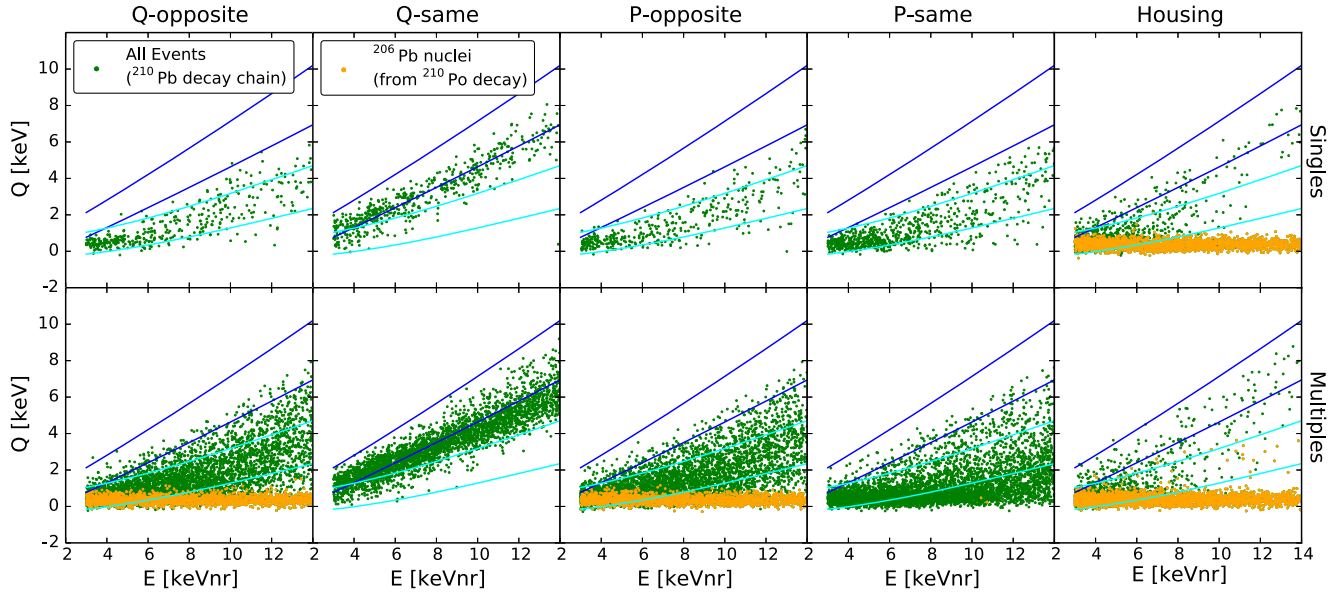
FIG. 7 (color online). Expected distribution of background events in the plane of ionization versus recoil energy (for a generic CDMS II Ge detector), from simulations of surface events originating from the adjacent detector and striking the detector’s charge side (far left column), from the detector’s charge side (second column from left), from the adjacent detector and striking the detector’s phonon side (third column), from the detector’s phonon side (fourth column), and from the housing (last column), as labeled (see Fig. 2 for a schematic). The top row shows single-scatter events and the bottom shows multiple-scatter events. The upper dark (blue) pair of curves represents the electron recoil band while the nuclear recoil band is shown by the lower, lighter (teal) pair of curves. Events from ^{210}\text{Po} decays that produce nuclear recoils are highlighted in a lighter shade (orange) at Q near zero. This simulation has \sim 100\times more events than expected in the WIMP-search data. Note that the relative numbers of events in each plot are fixed here; none of the relative normalizations (either of the 5 components or of singles to multiples) are allowed to float. Furthermore, note that decays on different surfaces cause quite different spectra, which need to be considered for a reliable background model.
