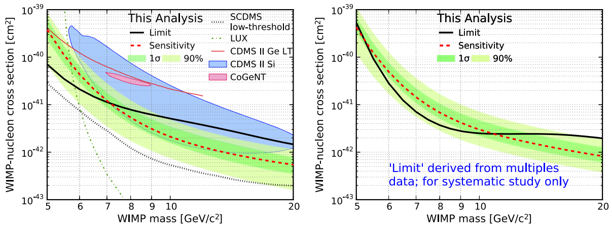
FIG. 12 (color online). Left panel: The limit (with standard halo assumptions and standard nuclear form factors as used in [4,10,11]) computed for this analysis is shown as the thick solid black line. The thick, dashed (dark-red) line is our best estimate for the expected sensitivity of this analysis, with the green (light-green) shaded region directly around it indicating the 1\sigma (90%) uncertainty. The limit is stronger than the estimated sensitivity below \sim 7 \text{ GeV}/c^2 , while at larger WIMP masses the limit is systematically above the sensitivity, indicating a systematic effect not yet taken into account. Right panel: This figure shows the limit calculated using multiples data instead of singles data. Multiples data do not contain WIMPs, and therefore the expected sensitivity and the limit should be identical to within statistical fluctuations. A similar trend of a stronger than expected limit at lower WIMP masses and a weaker than expected limit at higher masses is observed, indicating that the same systematic effect that is present in the singles is also present in the multiples data, although to a lesser extent.
