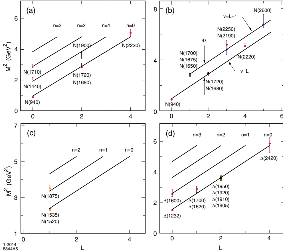
FIG. 1 (color online). Orbital and radial baryon excitation spectrum. (a) Positive-parity spin- \frac{1}{2} nucleons and (b) spectrum gap between the negative-parity spin- \frac{3}{2} and the positive-parity spin- \frac{1}{2} nucleons families. (c) Minus-parity spin- \frac{1}{2} N and (d) plus- and minus-parity spin- \frac{1}{2} and spin- \frac{3}{2} \Delta families. We have used in this figure the value \sqrt{\lambda_B} = 0.49 GeV for nucleons and 0.51 GeV for the deltas.
