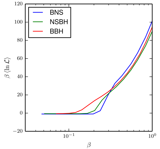
FIG. 5 (color online). The integrand of the evidence integral [Eq. (41)] versus \beta for the analyses of synthetic GW signals in § VB. The evidence is given by the area under each curve. Table I gives the results of the integration together with the estimated error in the quadrature, following the procedure described in § IV C. The jaggedness of the curves illustrates that the temperature spacing required for convergent MCMC simulations is larger than that required for accurate quadrature to compute the evidence; the flatness at small \beta illustrates that, for these simulations, the high-temperature limit is sufficient for convergence of the evidence integral.
