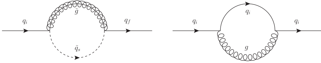
FIG. 1. Quark self-energy diagrams.
