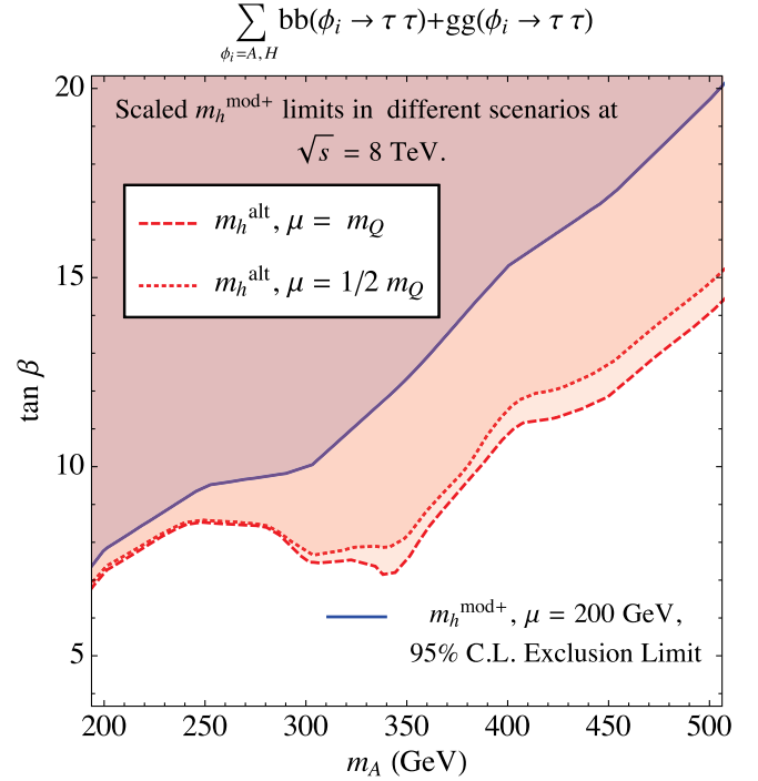
FIG. 7 (color online). Direct search bounds from the inclusive \tau^+\tau^- mode in our benchmarks at LHC8. The solid line displays the current CMS bounds in the m_h^{\text{mod+}} scenario with \mu = 200 GeV [36].
