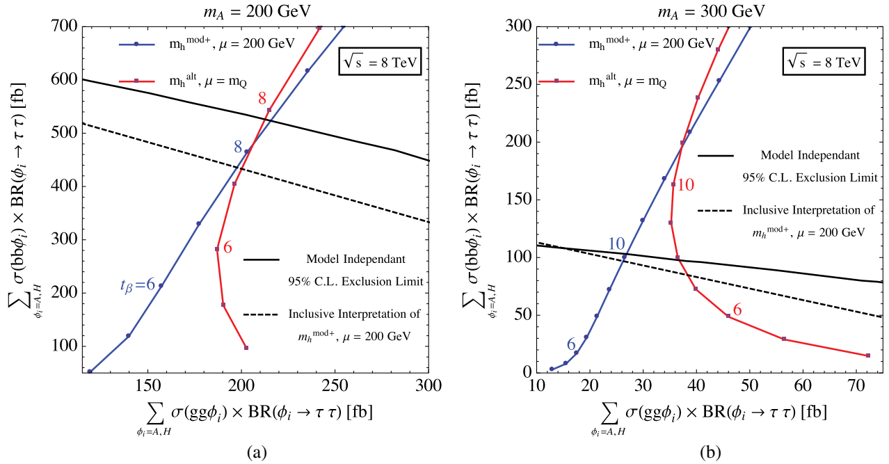
FIG. 10 (color online). Comparison of exclusion limits obtained via the model-independent analysis and our inclusive interpretation of the limits for the m_h^{\text{mod}+} scenario, with \mu = 200 GeV. The dots represent values of t_\beta in units of 1, where values are labeled in blue or red corresponding to the m_h^{\text{mod}+} scenario, with \mu = 200 GeV, and m_h^{\text{alt}} scenario, with \mu = m_Q , respectively.
