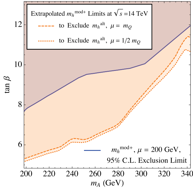
FIG. 8 (color online). The dashed and dotted line exhibit the projected bounds at \sqrt{s} = 14 TeV in the m_h^{\text{mod}+} scenario with \mu = 200 GeV, such that all values of t_\beta are excluded in the m_h^{\text{alt}} scenario for large values of \mu . The solid line displays the current CMS bounds in the m_h^{\text{mod}+} scenario with \mu = 200 GeV [36].
