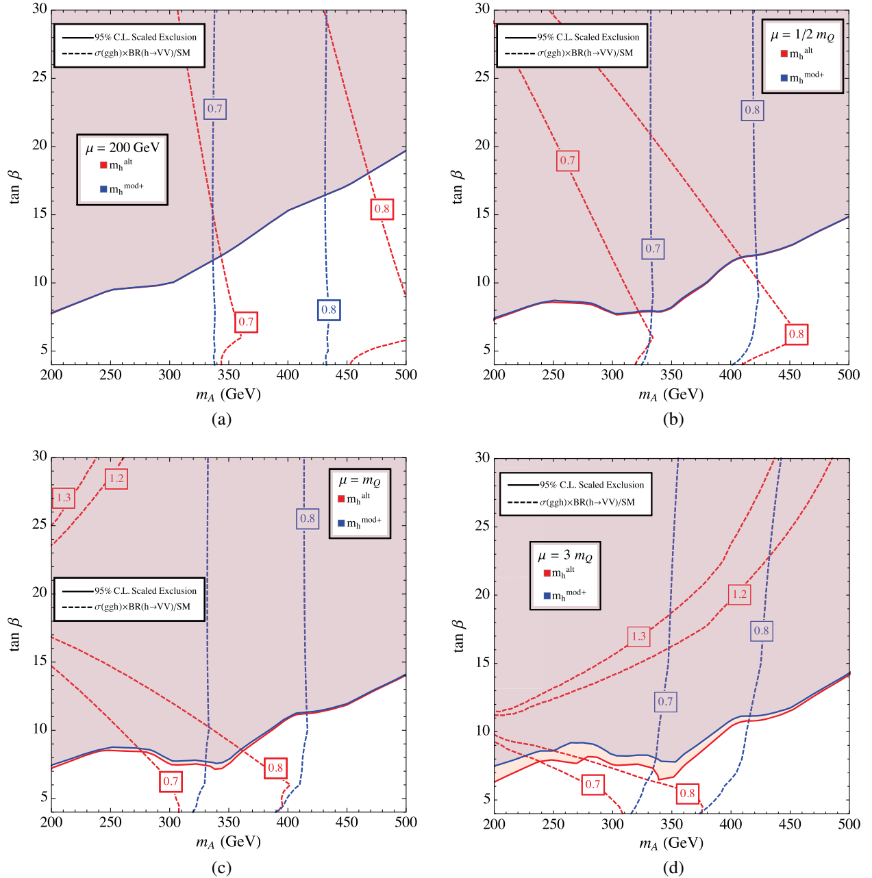
FIG. 9 (color online). Dashed contours show deviations of the signal strength into massive gauge bosons for the lightest CP -even Higgs boson with respect to the SM values in the m_h^{\text{mod+}} (blue line) and m_h^{\text{alt}} (red line) scenarios in the m_A - t_\beta plane for different values of \mu . Shaded regions denote parameters excluded by direct searches for heavy CP -even and CP -odd Higgs bosons decaying into pairs of \tau leptons.
