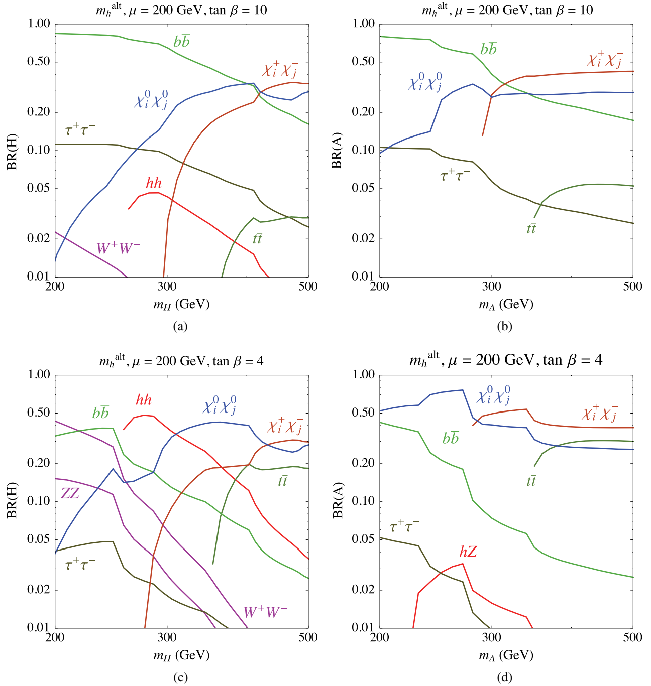
FIG. 3 (color online). Branching ratios of the heavy CP -even (left panels) and CP -odd (right panels) Higgs bosons as a function of their respective masses in the m_h^{\text{alt}} scenario, for t_\beta = 10 (top panels) and t_\beta = 4 (bottom panels), for small values of the Higgsino mass parameter, \mu = 200 GeV.
