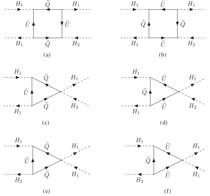
FIG. 1. One-loop diagrams contributing to the coefficient Z_6 of the Higgs basis operator (H_1^\dagger H_1)(H_1^\dagger H_2) . Using the interaction Lagrangian given in Eq. (52), one sees that the parametric dependence for the six diagrams are h_t^4 s_\beta^3 c_\beta X_t^3 Y_t for (a),(b); h_t^4 s_\beta^3 c_\beta X_t^2 for (c),(d); and h_t^4 s_\beta^3 c_\beta X_t Y_t for (e),(f).
