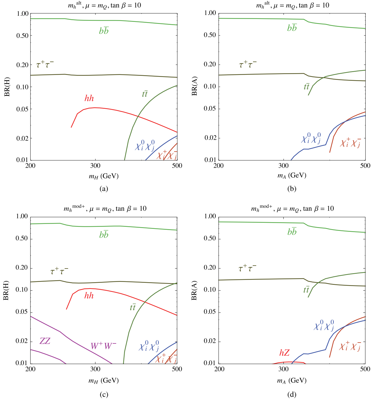
FIG. 4 (color online). Branching ratios of the heavy CP -even (left panels) and CP -odd (right panels) Higgs bosons as a function of their respective masses for t_\beta = 10 in the m_h^{\text{alt}} scenario (top panels) and m_h^{\text{mod}+} scenario (bottom panels), for large values of the Higgsino mass parameter, \mu = m_Q .
