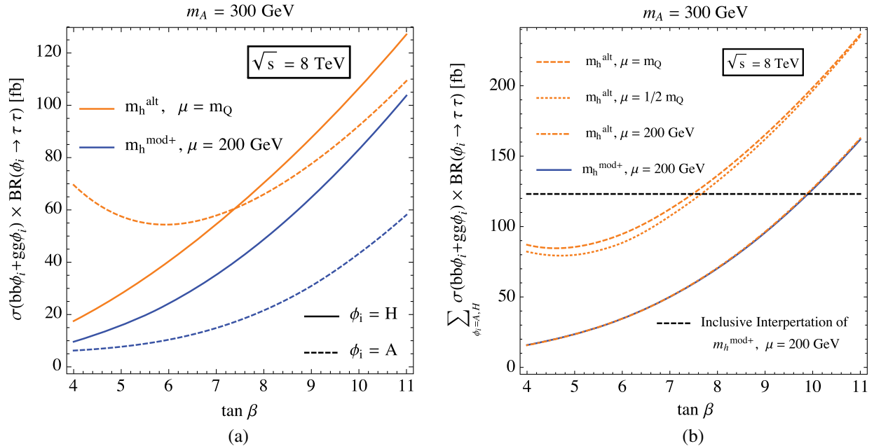
FIG. 6 (color online). Inclusive production cross section times branching ratio in the \tau^+ \tau^- mode for m_A = 300 GeV. The black dashed line in the right panel denotes the extracted upper limit from CMS bounds presented in Ref. [36].
