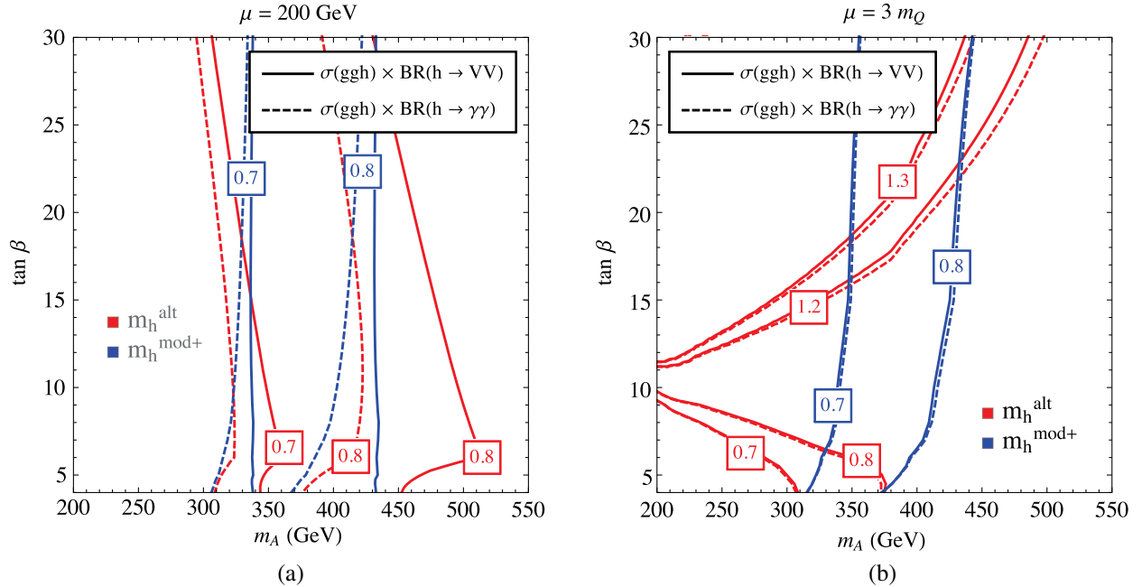
FIG. 11 (color online). Deviation of the signal strengths with respect to the SM values for the lightest Higgs boson decaying into two photons and two massive gauge bosons.
