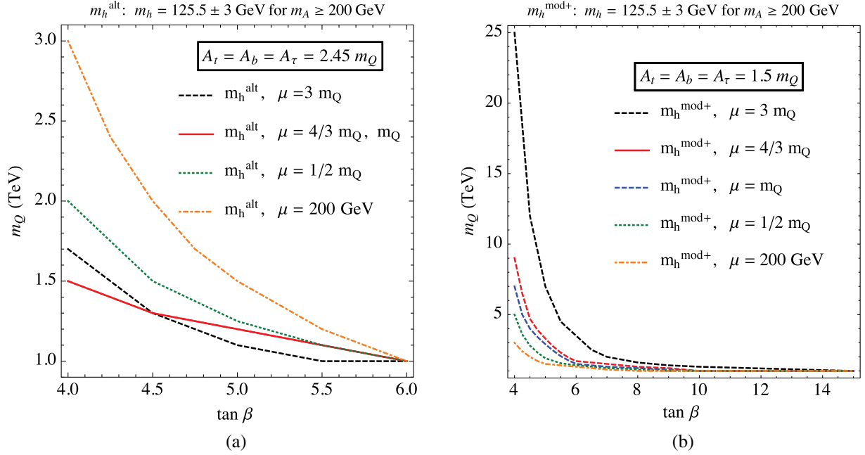
FIG. 2 (color online). Values of m_Q necessary to accommodate the proper value of the lightest CP -even Higgs mass, for different values of \mu in the m_h^{\text{alt}} and m_h^{\text{mod+}} scenarios.
