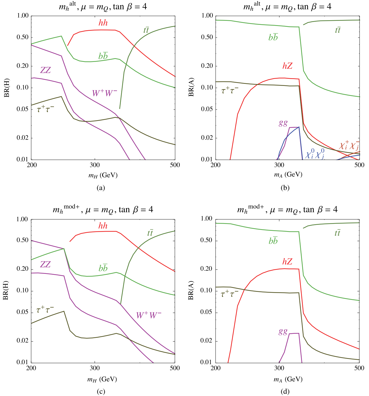
FIG. 5 (color online). Branching ratios of the heavy CP -even (left panels) and CP -odd (right panels) Higgs bosons as a function of their respective masses for t_\beta = 4 in the m_h^{\text{alt}} scenario (top panels) and m_h^{\text{mod}+} scenario (bottom panels), for large values of the Higgsino mass parameter, \mu = m_Q .
