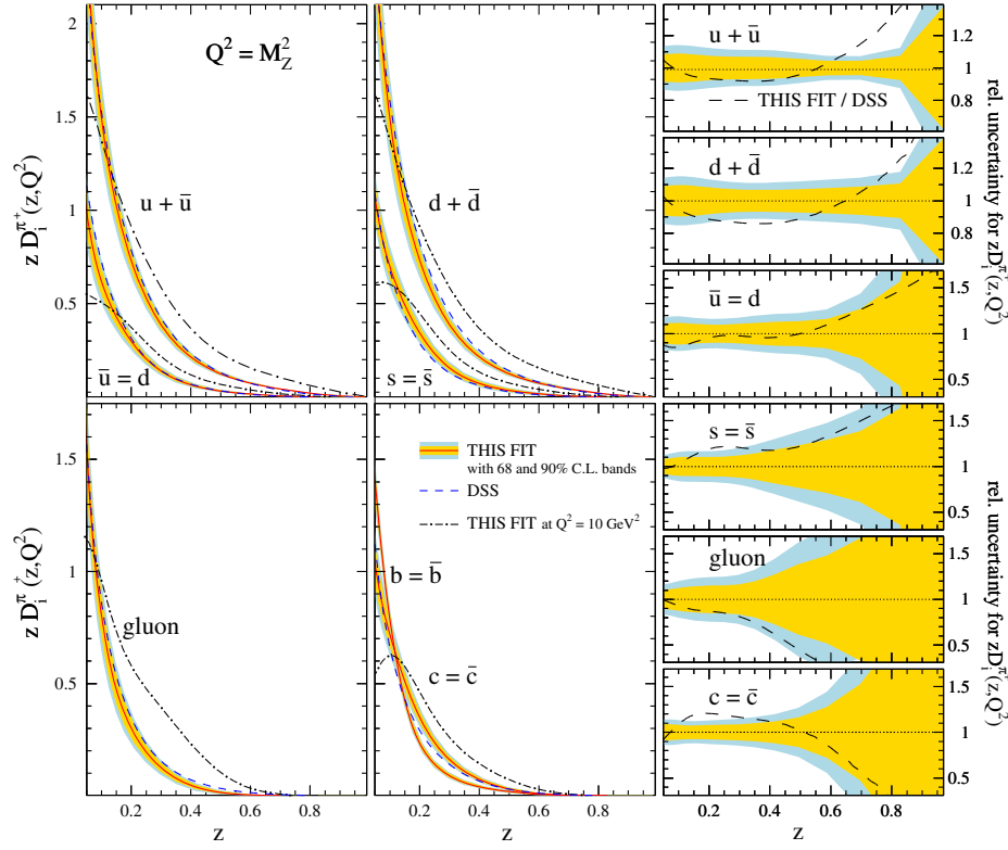
FIG. 2 (color online). As in Fig. 1 but now for Q^2 = M_Z^2 . Note that here also a bottom-to- \pi^+ fragmentation function is shown.
