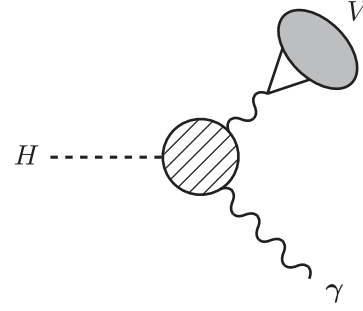
FIG. 2. The Feynman diagram for the indirect amplitude for H \rightarrow V + \gamma . The hatched circle represents top-quark or W -boson loops, and the shaded blob represents the quarkonium wave function.
