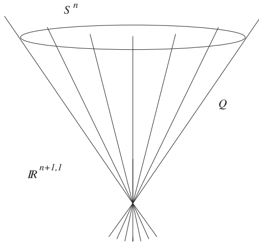
FIG. 1. The flat model for a conformal manifold. The n -sphere with its canonical conformal class of metrics is given by the space of lightlike rays Q in \mathbb{R}^{n+1,1} .
