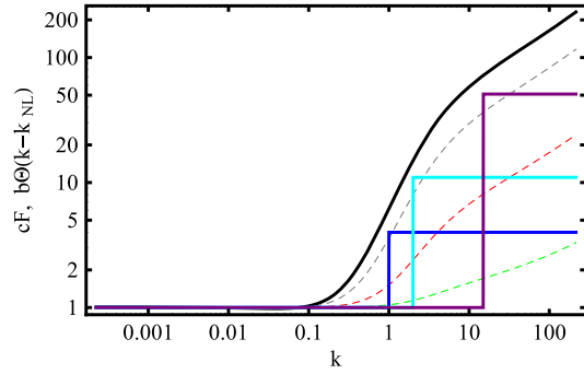
FIG. 1 (color online). Log-Log plot of the “transfer functions” (5) at redshift z = 1 multiplied by c = 1 (solid black), c = 0.5 (upper dashed, gray), c = 0.1 (middle dashed, red) c = 0.01 (bottom dashed, green). Solid blue, cyan and purple curves are the step functions in (6) with b = 3 , k_{\text{NL}} = 1 \text{ Mpc}^{-1} ; b = 10 , k_{\text{NL}} = 2 \text{ Mpc}^{-1} ; b = 50 , k_{\text{NL}} = 15 \text{ Mpc}^{-1} , respectively. Position of each step is given by k_{\text{NL}} .
