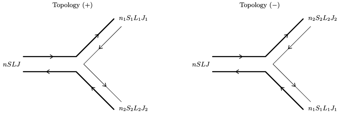
FIG. 4. Quark line topologies. The two topologies differ in the arrangement of the quarks from the initial meson ( Q and \bar{Q} ) and the created pair ( q and \bar{q} ) in the final states. In the (+) topology the mesons with quantum numbers n_1S_1L_1J_1 and n_2S_2L_2J_2 are respectively Q\bar{q} and q\bar{Q} states. The (-) topology describes the opposite situation.
