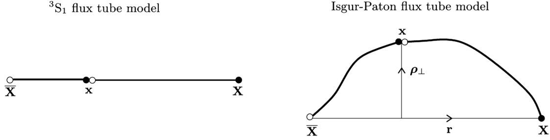
FIG. 1. The geometry of quark-pair creation in the {}^3S_1 and Isgur-Paton flux tube models. The initial Q and \bar{Q} are at \mathbf{X} and \bar{\mathbf{X}} respectively, and the created q\bar{q} pair is at \mathbf{x} .
