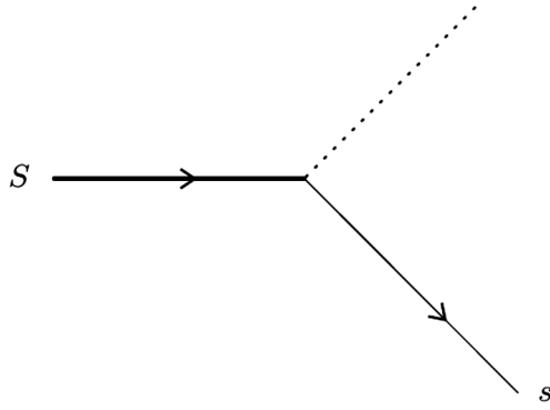
FIG. 3. The projections of quark spin in the pseudoscalar-meson emission model, and the corresponding process in nonflip, triplet models.
