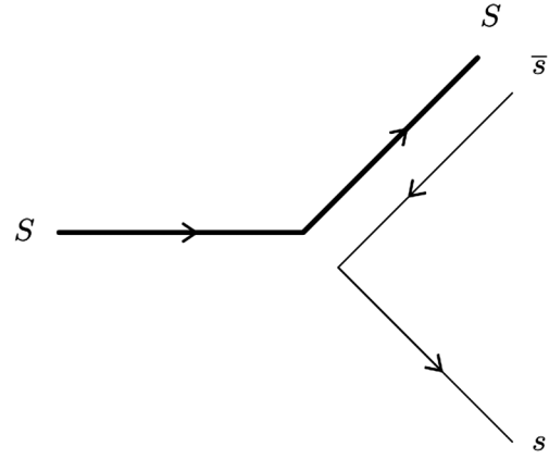
FIG. 3. The projections of quark spin in the pseudoscalar-meson emission model, and the corresponding process in nonflip, triplet models.
