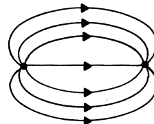
FIG. 1. Electric field of a high-energy pair a short time after their production.
