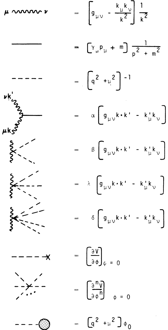
FIG. 10. Feynman rules for the model of Sec. V.
