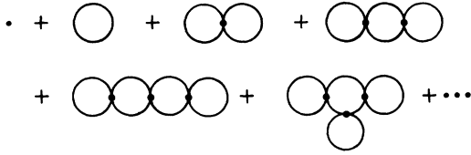
FIG. 3. Graphs that dominate V(\hat{\phi}) in large- n limit.
