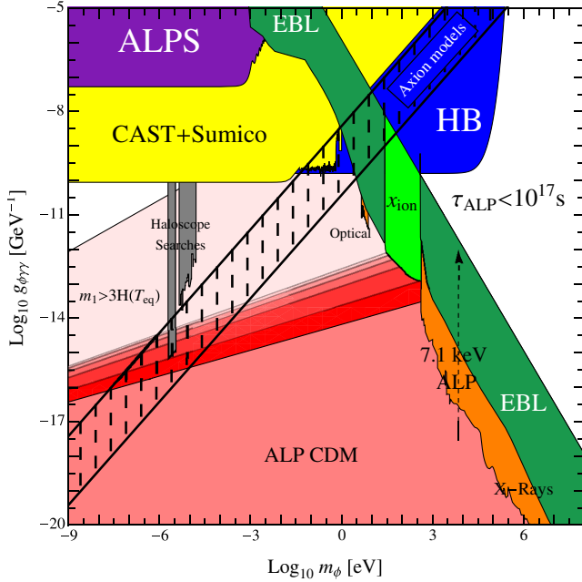
FIG. 1 (color online). Parameter space for axionlike particle dark matter [10]. The thick black line indicates the region which could explain the 3.55 keV line assuming that the 7.1 keV ALP makes up all of the dark matter. The dashed black line shows the possible couplings when the ALP is only a fraction of the dark matter. The limits shaded in green and in orange assume that the ALP gives the full dark matter density. Accordingly, they weaken with the dark matter fraction \sim 1/\sqrt{x_{\phi}} .
