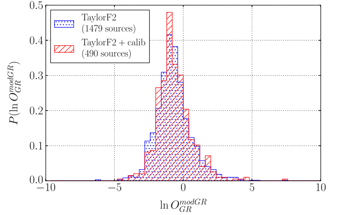
FIG. 4 (color online). Single-source background distributions for TaylorF2 injections without calibration errors (blue, dotted) and with frequency dependent amplitude and phase errors modeled as in [71] (red, dashed), both analyzed with TaylorF2 waveforms cut off at 400 Hz.
