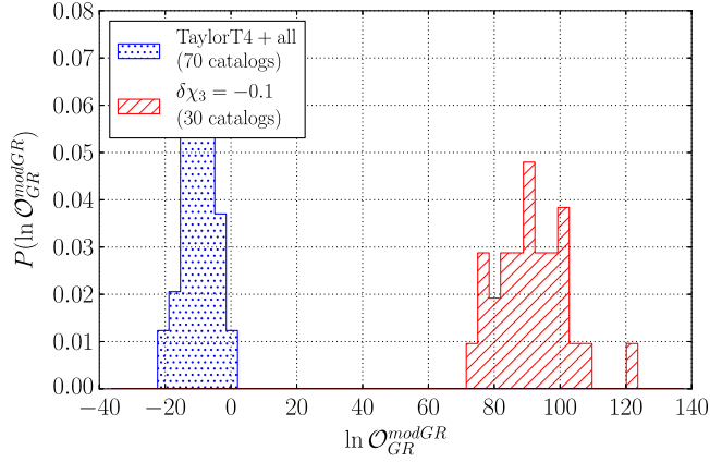
FIG. 9 (color online). Log odds ratio distributions for catalogs of 15 sources each. The blue, dotted histogram is the GR background for TaylorT4 signals with precessing spins, neutron star tidal deformation, and instrumental calibration errors. The red, dashed one is a foreground distribution for signals with the same effects present, and with a GR violation that takes the form of a constant -10\% shift at 1.5 PN, as explained in the main text. In both cases, the recovery is with (anti-)aligned spinning TaylorF2 waveforms cut off at 400 Hz.
