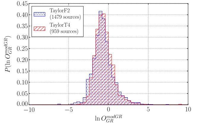
FIG. 2 (color online). Single-source background distributions for TaylorF2 injections (blue, dotted) and TaylorT4 injections (red, dashed), both analyzed with TaylorF2 waveforms cut off at 400 Hz.
