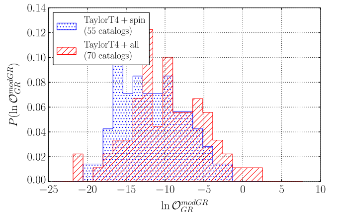
FIG. 8 (color online). The same comparison as in Fig. 7, but now for catalogs of 15 sources each. Note how GR is typically much more favored when information from multiple GR sources is combined.
