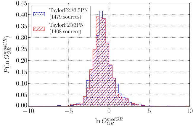
FIG. 3 (color online). Single-source background distributions for TaylorF2 injections to 3.5 PN, where in one case the recovery waveform is also TaylorF2 to 3.5 PN (blue, dotted) and in the other case, TaylorF2 to 3PN (red, dashed), both cut off at 400 Hz.
