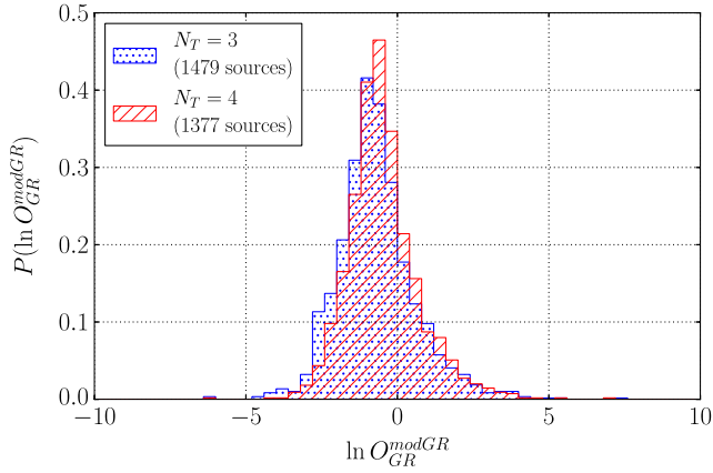
FIG. 5 (color online). Single-source background distributions for TaylorF2 injections with TaylorF2 recovery, in one case with three testing parameters (blue, dotted) and in the other with four (red, dashed).
