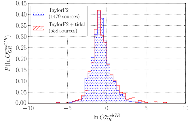
FIG. 1 (color online). Single-source background distributions for TaylorF2 injections without tidal effects (blue, dotted) and injections with strong tidal deformability (red, dashed), both analyzed with TaylorF2 waveforms that are cut off at f = 400 Hz.
