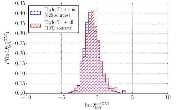
FIG. 7 (color online). Single-source background distributions for TaylorT4 injections with precessing spins (blue, dotted) and TaylorT4 injections with precessing spins, tidal effects, and calibration errors (red, dashed). In both cases, the recovery is with (anti-)aligned spinning TaylorF2 cut off at 400 Hz.
