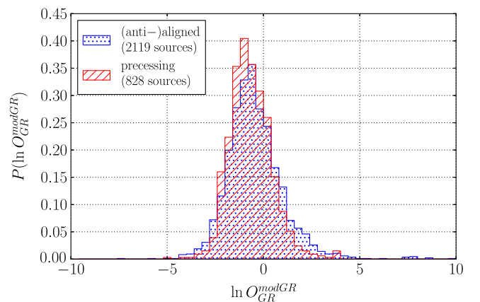
FIG. 6 (color online). Single-source background distributions for TaylorF2 injections with (anti-)aligned spins (blue, dotted) and TaylorT4 injections with precessing spins (red, dashed). In both cases the recovery is with TaylorF2 waveforms cut off at 400 Hz.
