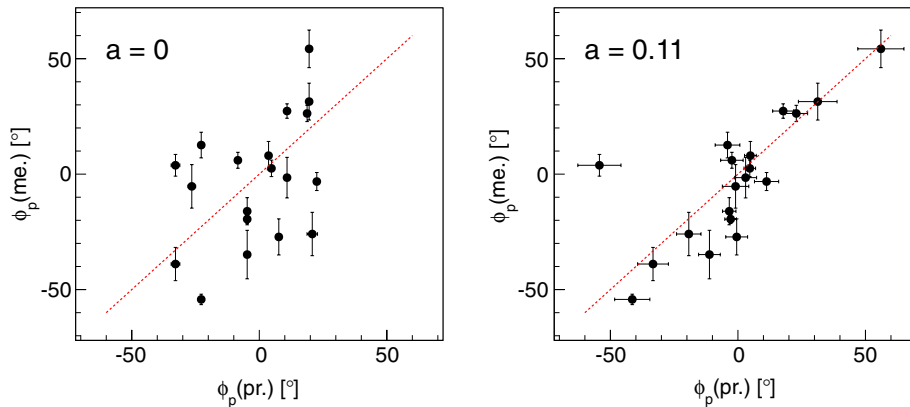
FIG. 14 (color online). Left panel: the measured polarization angle for pure geomagnetic emission, a = 0 [see Eqs. (8) and (10)], versus the predicted polarization angle for the data set recorded with the prototype. Right panel: the same data set but for a value of a = 0.11 \pm 0.07 . See also the captions to Figs. 8 and 10.
