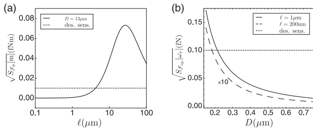
FIG. 2. (a) Patch torque power spectrum for the Birmingham experiment, and (b) patch force power spectrum for the IUPUI experiment. Both calculations are performed with V_{\text{rms}} = 4.5 mV. Fig. 2(b) shows two curves corresponding to different patch sizes: one given by the thickness of the gold film, \ell = 200 nm (dashed line) and multiplied by 10 to be seen at the shown scale, and another for 1 \mu\text{m} size patches. The horizontal short dashed lines show the design sensitivity of the two setups.
