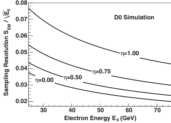
FIG. 30. Sampling contribution S_{EM}/\sqrt{E_0} to the electron fractional energy resolution as a function of the electron energy E_0 for four different electron incident angles \eta = 0.0, 0.5, 0.75, and 1.0 . The strong energy and angular dependencies are caused by the energy lost in the uninstrumented material before the calorimeter.
