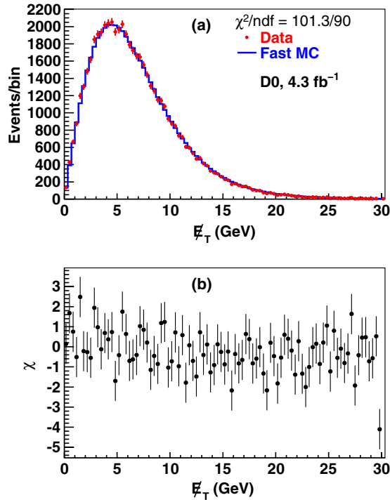
FIG. 56 (color online). (a) Comparison between data and fast MC for the E_T distribution of in Z \rightarrow ee events, and (b) \chi value per bin, where \chi_i = \Delta N_i / \sigma_i . \Delta N_i is the difference between the number of events for data and fast MC, and \sigma_i is the statistical uncertainty in bin i .
