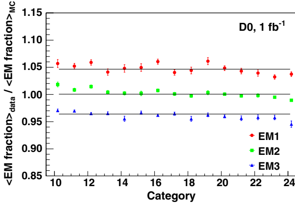
FIG. 8 (color online). The ratio of data to simulation for the means of the EM layer energy fraction distributions in Z \rightarrow ee events for each of the first three EM layers and each of the 15\eta categories shown before the correction described in Sec. VC is applied. Each of the three horizontal lines indicates the result of a fit of a common constant to the 15 data points from a given EM layer.
