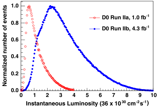
FIG. 4 (color online). Instantaneous luminosity profiles for Run IIa and Run IIb. The instantaneous luminosity is given as a multiple of 36 \times 10^{30} \text{ cm}^{-2} \text{ s}^{-1} . Since there were 36 p\bar{p} bunch crossings per turn in the Tevatron Collider, the values in the abscissa can be interpreted as the average bunch instantaneous luminosity.
