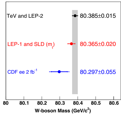
FIG. 14 (color online). Comparisons of experimental measurements of the W -boson mass: “TeV and LEP-2” represents direct measurements of the W -boson mass; “LEP-1 and SLD ( m_t )” represents the standard-model analysis of Z-pole measurements; and “CDF ee 2 \text{fb}^{-1} ” represents this analysis. The horizontal bars represent total uncertainties. For this analysis, the inner uncertainty bar is the measurement uncertainty.
