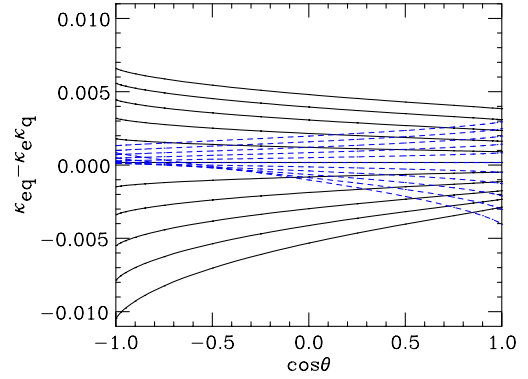
FIG. 19 (color online). Real part of \kappa_{eq} - \kappa_e \kappa_q as a function of \cos\theta for \sin^2\theta_W = 0.2231 . Each curve corresponds to a different value of \sqrt{s} , varying from 66 to 116 GeV. The curves change monotonically with each step of s . The solid (black) curves are for u -type amplitudes, and the dashed (blue) curves are for d -type amplitudes. For the u -type amplitude, the highest mass corresponds to the lowermost curve at \cos\theta = -1 , and for the d -type amplitude, the highest mass corresponds to the uppermost curve at \cos\theta = -1 . The flat lines in the middle correspond to \sqrt{s} = M_Z .
