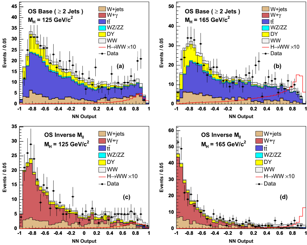
FIG. 10 (color online). Predicted and observed distributions of neural network output variables for networks trained to separate potential Higgs boson events from background contributions in the (a),(b) OS base ( \geq 2 jets) and (c),(d) OS inverse M_{\ell\ell} search samples for Higgs boson mass hypotheses of 125 and 165 \text{GeV}/c^2 . The overlaid signal predictions correspond to the sum of four production modes ( ggH , WH , ZH , and VBF) and are multiplied by a factor of 10 for visibility. Normalizations for background event yields are those obtained from the final fit used to extract search limits.
