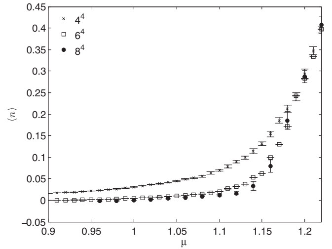
FIG. 1. Average density \langle n \rangle in the critical region for the lattices V = 4^4, 6^4, 8^4 .
