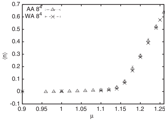
FIG. 3. Comparison of the average density \langle n \rangle obtained with the worm algorithm (WA) [22] with the Aurora algorithm (AA) presented here, for the lattice V = 8^4 . We thank C. Gattringer and T. Kloiber for providing us their results.
