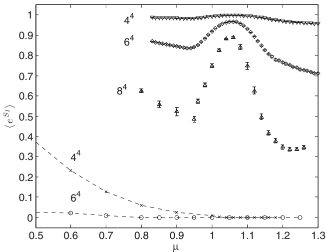
FIG. 4. The data on the top right show the average phase obtained with the Aurora algorithm on lattices 4^4 , 6^4 and 8^4 . It is interesting that the average phase is large precisely in the most interesting region just above \mu = 1 . The dashed lines on the bottom left display, for comparison, the average phase obtained with a naive phase-quenched Monte Carlo algorithm on lattices 4^4 and 6^4 . Even on a 4^4 lattice, the sign problem in the phase-quenched algorithm completely hides the interesting region.
