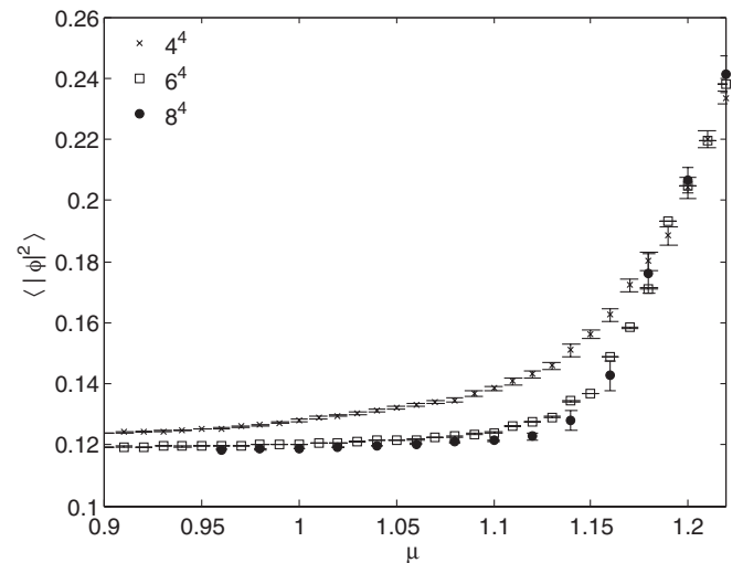
FIG. 2. The same as in Fig. 1 for the observable \langle |\phi|^2 \rangle .
