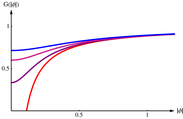
FIG. 1 (color online). Plot of the function G(|\phi|) in the one-loop Coulomb branch metric in YM-CS (namely, S \supset \int G(|\phi|) \partial_\mu \phi_3 \partial^\mu \bar{\phi}_3 ), for different values of k . The four curves correspond to k = 0, 6, 10, 14 (in red, violet, magenta, and blue, respectively), with g = 1 in all cases. For k = 0 , the metric vanishes at \phi = \frac{g}{2\sqrt{2}\pi} , while it stays regular everywhere along the Coulomb branch for k large enough that our perturbative computations can be trusted.
