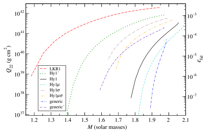
FIG. 9 (color online). The full relativistic maximum quadrupole deformations (and fiducial ellipticity) of hybrid stars vs mass, using the EOSs from Table I in Ref. [29], all with a surface tension of \sigma = 80 \text{ MeV fm}^{-2} and a breaking strain of 0.1.
