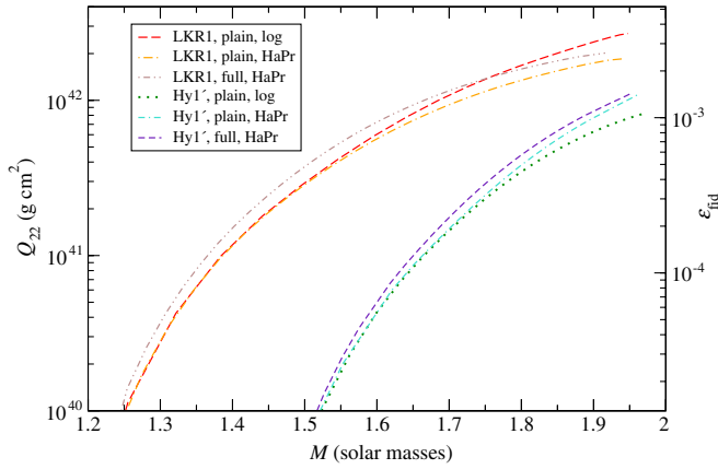
FIG. 11 (color online). The full relativistic maximum quadrupole deformations (and fiducial ellipticity) of hybrid stars vs mass, for the LKR1 and Hy1' EOSs from Ref. [29], with a surface tension of \sigma = 80 \text{ MeV fm}^{-2} , showing the effects of the different interpolation methods and EOS additions. Here, “plain” denotes no additions, while “full” denotes both blob and lattice additions. Similarly, “log” and “HaPr” denote the standard logarithmic and Haensel-Prószyński interpolation, respectively. Note that many of the curves end somewhat short of the maximum mass, due to difficulties with the numerics.
