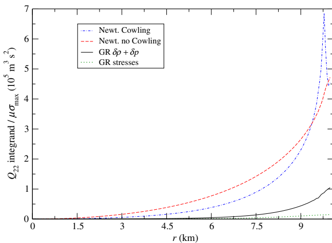
FIG. 3 (color online). The Q_{22} integrands (without the factor of \mu \bar{\sigma}_{\max} ) for the SLy EOS and a maximum mass, 2.05M_{\odot} star, with a compactness of 0.60.
