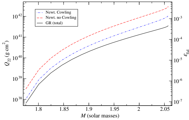
FIG. 7 (color online). The Newtonian Cowling, Newtonian no-Cowling, and full relativistic (including stress contributions) values for the maximum quadrupole deformations (and fiducial ellipticity) of hybrid stars vs mass, using the Hy1 EOS with a surface tension of \sigma = 80 \text{ MeV fm}^{-2} and a breaking strain of 0.1.
