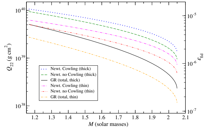
FIG. 5 (color online). The Newtonian Cowling, Newtonian no-Cowling, and full relativistic (including stress contributions) values for the maximum quadrupole deformations (and fiducial ellipticity) due to crustal stresses versus mass for two choices of crustal thickness. These are computed using the SLy EOS with the rough HJA recipe for the shear modulus and a breaking strain of 0.1.
