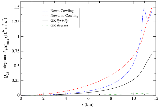
FIG. 2 (color online). The Q_{22} integrands (without the factor of \mu \bar{\sigma}_{\max} ) for the SLy EOS and a 1.40M_{\odot} star with a compactness of 0.35.
