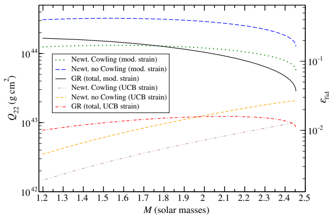
FIG. 10 (color online). The Newtonian Cowling, Newtonian no-Cowling, and full relativistic (including stress contributions) values for the quadrupole deformations (and fiducial ellipticity) of maximally strained strange quark stars vs mass, using the EOS discussed in the text with a breaking strain of 0.1. We show these both for the standard UCB uniform maximum strain and our modification that yields significantly larger quadrupoles in this case.
