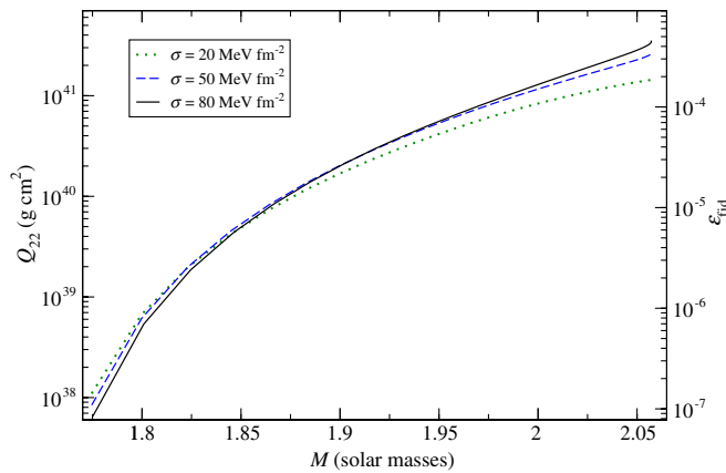
FIG. 8 (color online). The full relativistic maximum quadrupole deformations (and fiducial ellipticity) of hybrid stars vs mass, using the Hy1 EOS with various surface tensions \sigma and a breaking strain of 0.1.
