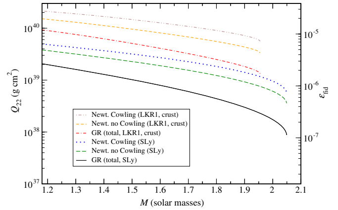
FIG. 6 (color online). The Newtonian Cowling, Newtonian no-Cowling, and full relativistic (including stress contributions) values for the maximum quadrupole deformations (and fiducial ellipticity) due to crustal stresses vs mass, for the SLy EOS with the detailed Douchin and Haensel + Ogata and Ichimaru model for the shear modulus and a breaking strain of 0.1, plus the crustal quadrupoles for the LKR1 EOS with the same crustal model.
