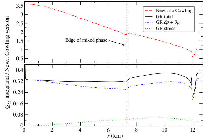
FIG. 4 (color online). Ratios of the Q_{22} integrands with the Newtonian Cowling approximation integrand for the Hy1 EOS and a maximum mass, 2.06M_{\odot} star, with a compactness of 0.49. Note that the top and bottom plots have completely separate vertical axis scalings.
