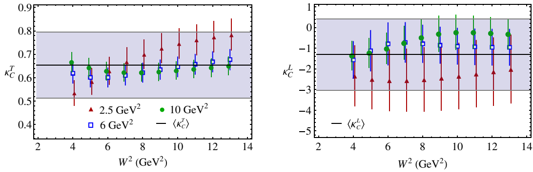
FIG. 7 (color online). Continuum parameters \kappa_C^T (left) and \kappa_C^L (right) fitted to the DIS data, parametrized by the ABM11 global QCD fit [40], as a function of W^2 for fixed Q^2 = 2.5 GeV 2 (red triangles), 6 GeV 2 (blue squares), and 10 GeV 2 (green circles). The average values \langle \kappa_C^{T,L} \rangle are indicated by the solid lines, with the shaded band giving their uncertainty. Note that some of the points have been slightly offset for clarity.
