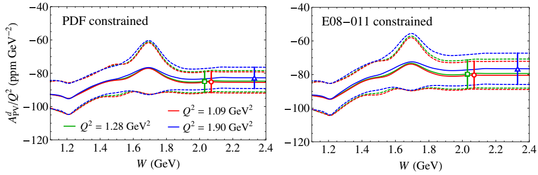
FIG. 15 (color online). Predictions for the parity-violating deuteron asymmetry A_{PV}^d/Q^2 as a function of W (solid) for the DIS region kinematics of the Jefferson Lab E08-011 experiment [54] at Q^2 = 1.28 GeV ^2 (green), 1.09 GeV ^2 (red) and 1.90 GeV ^2 (blue) (see also Table II). The uncertainties (dashed) are computed in the AJM model with the continuum parameters \kappa_C^{T,L} constrained by DIS structure functions (left), and by the E08-011 resonance region data (right). The predictions at the experimental W values [54] are shown as pseudo-data points (open symbols).
