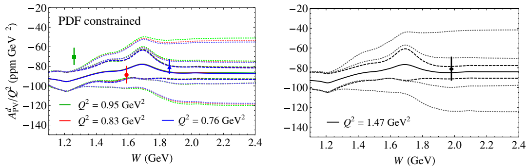
FIG. 12 (color online). Deuteron parity-violating asymmetry A_{PV}^d/Q^2 as a function of W for incident electron energy E = 4.9 GeV (left) and E = 6.1 GeV (right). The data points from the Jefferson Lab E08-011 experiment [15] at W = 1.26 (green square), 1.59 (red circle), 1.86 (blue triangle) and 1.98 GeV (black diamond) correspond to average values of Q^2 = 0.95, 0.83, 0.76 and 1.47 GeV 2 , respectively. The AJM model uncertainties (inner dashed band) are constrained by matching the continuum parameters \kappa_C^{T,L}(d) to the DIS region \gamma Z structure functions [40], and are compared with those computed with errors on \kappa_C^{T,L}(d) of 100% (outer dotted bands) and 25% (inner dotted bands).
