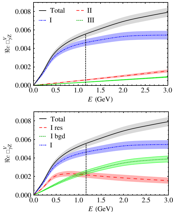
FIG. 14 (color online). Energy dependence of the contributions to \Re e \square_{\gamma Z}^V from the various regions in W and Q^2 displayed in Fig. 2 in the AJM model (top), and the breakdown of Region I into its resonant and nonresonant background components (bottom).
