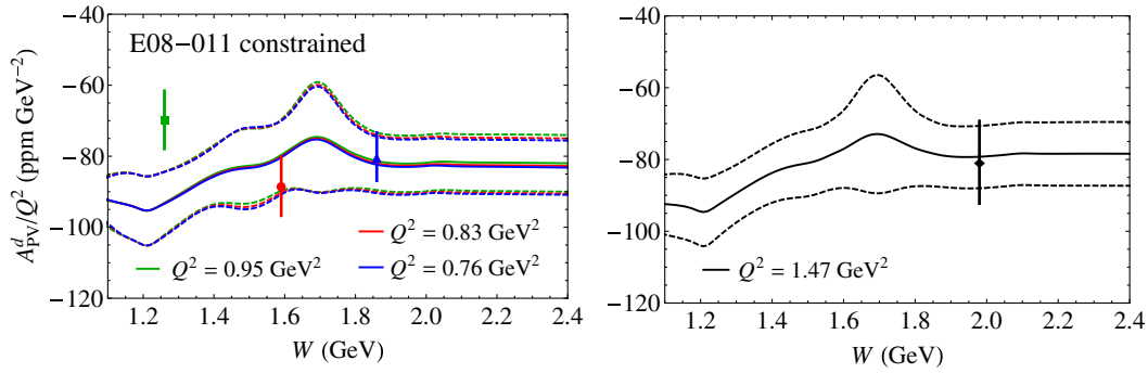
FIG. 13 (color online). As in Fig. 12, but with the AJM model asymmetries (solid) and their uncertainties (dashed) constrained by the E08-011 data [15]. Note the different scale on the ordinate to that in Fig. 12.
