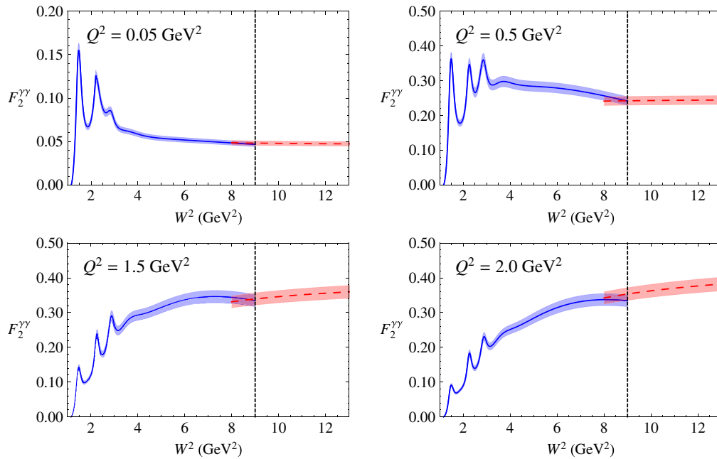
FIG. 3 (color online). Proton F_2^{\gamma\gamma} structure function versus W^2 at fixed Q^2 = 0.05, 0.5, 1.5 and 2 GeV ^2 for the CB fit [24] at low W (blue solid) and VMD + Regge parametrization [29] at high W (red dashed). The boundary between these (corresponding to Regions I and II in Fig. 2) is indicated by the vertical dashed line at W^2 = 9 GeV ^2 .
