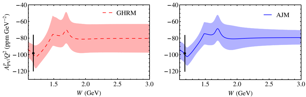
FIG. 10 (color online). Proton parity-violating inelastic asymmetry A_{PV}/Q^2 as a function of W , at fixed incident energy E = 0.69 \text{ GeV} and Q^2 = 0.34 \text{ GeV}^2 , for the GHRM Model II [14] (left) and the AJM model (right). The data point at W = 1.18 \text{ GeV} (black circle) is from the Jefferson Lab G0 experiment [53].
