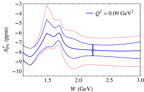
FIG. 16 (color online). AJM model prediction for the proton parity-violating asymmetry A_{PV}^p as a function of W for the Q_{\text{weak}} inelastic measurement [16] at Q^2 = 0.09 GeV ^2 (solid line and open symbol). The AJM model uncertainties (dashed) are compared with those from the GHRM model with 100% uncertainty on the continuum parameters (dotted).
