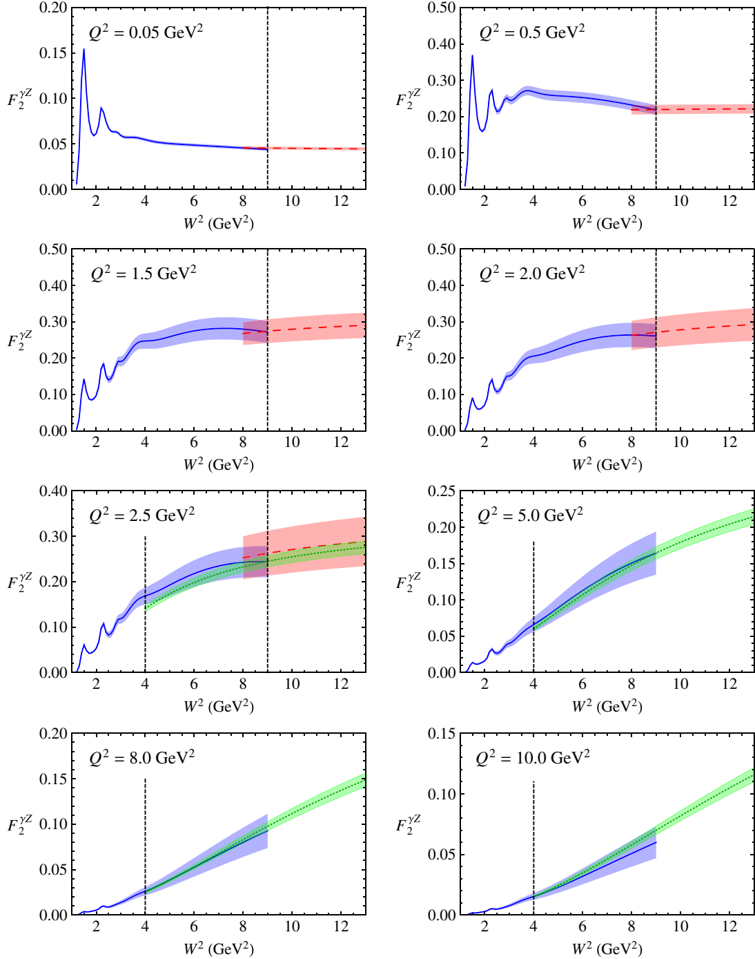
FIG. 8 (color online). Proton F_2^{\gamma Z} structure function versus W^2 at various fixed Q^2 values for the low- W CB fit [24] (blue solid) and the high- W VMD + Regge [29] (red dashed) and ABM11 [40] (green dotted) parametrizations. The boundaries between the Regions I, II and III are indicated by the vertical lines at W^2 = 4 and 9 \text{ GeV}^2 .
