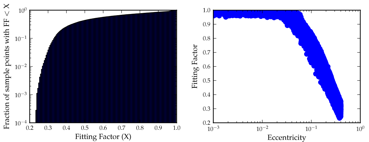
FIG. 1 (color online). The left panel is a cumulative histogram which indicates the fraction of points in the mass-space region where the bank of noneccentric waveforms has a value of \mathcal{FF} less than the associated value on the x axis. The right panel shows the \mathcal{FF} as a function of the binary system’s initial value of eccentricity.
