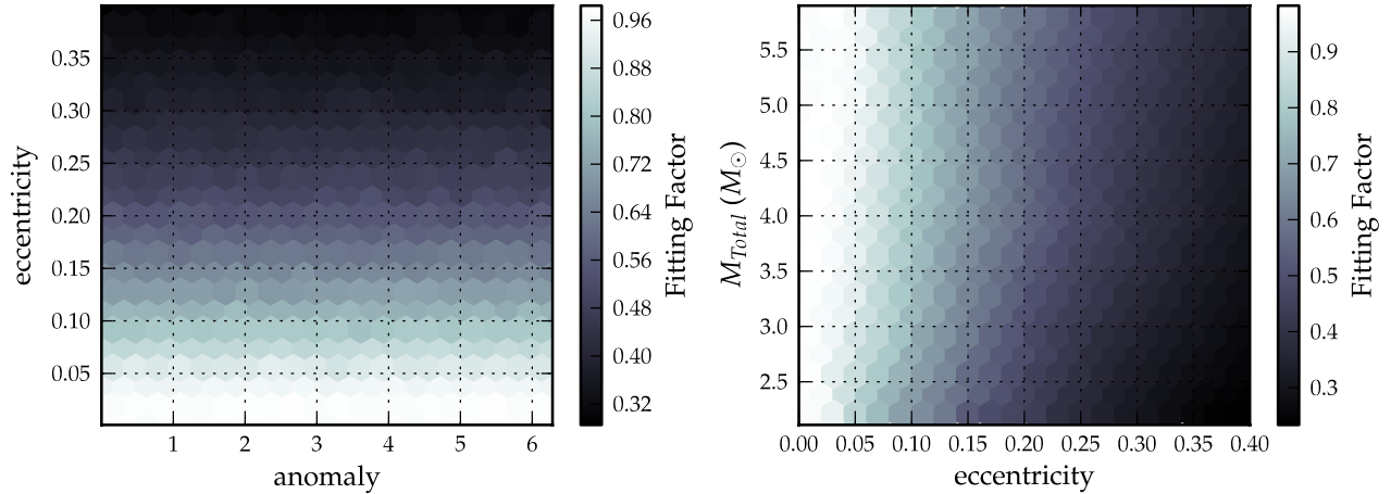
FIG. 2 (color online). The left panel shows the \mathcal{FF} as a function of the initial value of the eccentricity and the anomaly of the trajectory for binaries with component masses 1M_{\odot} < m < 3M_{\odot} . The right panel shows the correlation of the \mathcal{FF} with the initial orbital eccentricity and the total mass of the binary.
