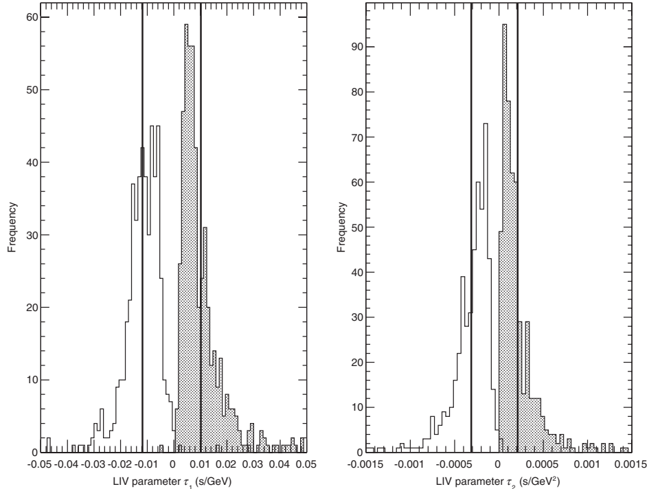
FIG. 18. Distributions of the lower and upper 99% C.L. limits for n = 1 (left pad) and n = 2 (right pad) for GRB 090510. The vertical lines denote the means of the distributions, used for constructing the calibrated CIs.
