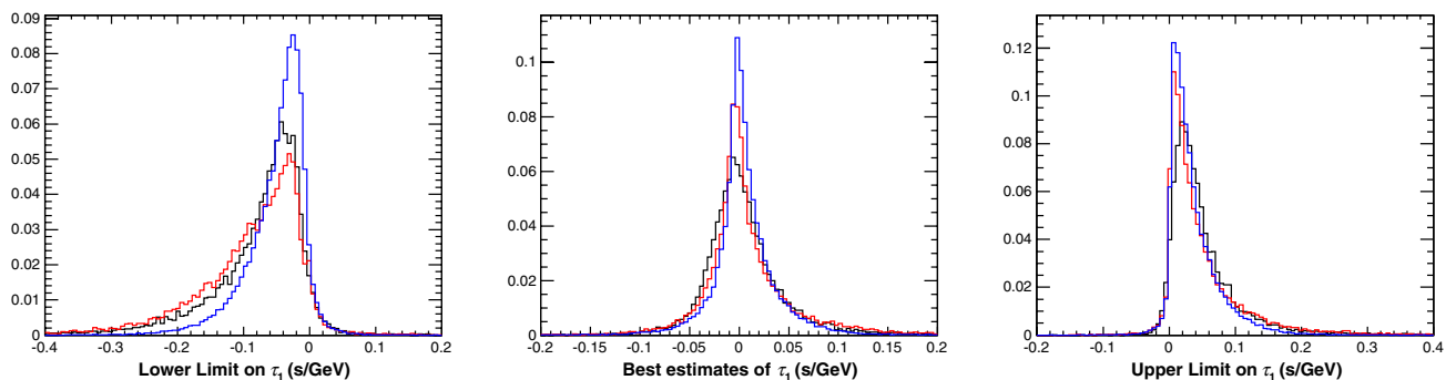
FIG. 20 (color online). Histograms of the 95% (one-sided) C.L. lower limits (left panel), best estimates (middle panel), and upper limits (right panel) of the LIV parameter \tau_1 produced by PV (black), SMM (red), and ML (blue) on simulated data sets.
