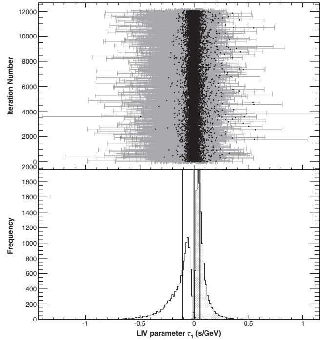
FIG. 14. Top: 99% C.L. CIs produced by the application of PV on the GRB 090510-inspired simulated data set for \tau_1 = 0 s/GeV. The black dots denote the best estimates of the LIV parameter. Bottom: distributions of the lower (left) and upper limits (right) of these confidence intervals. The two external vertical lines denote the medians of the two distributions, and the middle vertical line denotes the mean of the best estimates.
