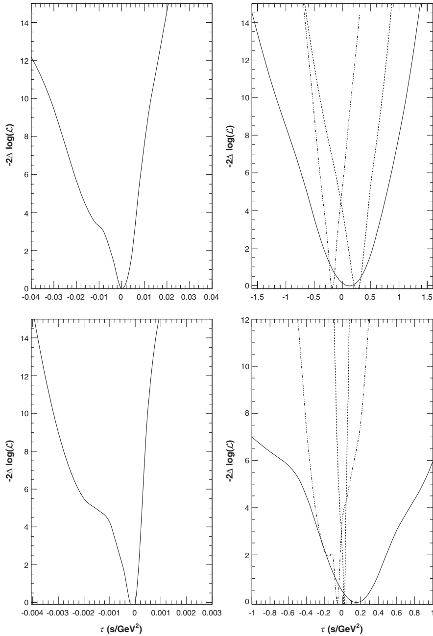
FIG. 8. -2\Delta \ln(\mathcal{L}) curves for linear (top row) and quadratic (bottom row) dependence of the speed of light on energy. Left column: GRB 090510. Right column: GRBs 080916C (full line), 090902B (dotted line), and 090926A (dashed double-dotted line).
