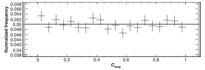
FIG. 16. Normalized empirical distribution P_{C_{\text{emp}}} (histogram) obtained from the application of PV on the GRB 090510-inspired data set for \tau_1 = 0 s/GeV superimposed on its theoretical expectation (uniform distribution, shown with the horizontal line). The fact that the empirical distribution follows a uniform distribution supports the validity of the assumptions behind our CI construction.
