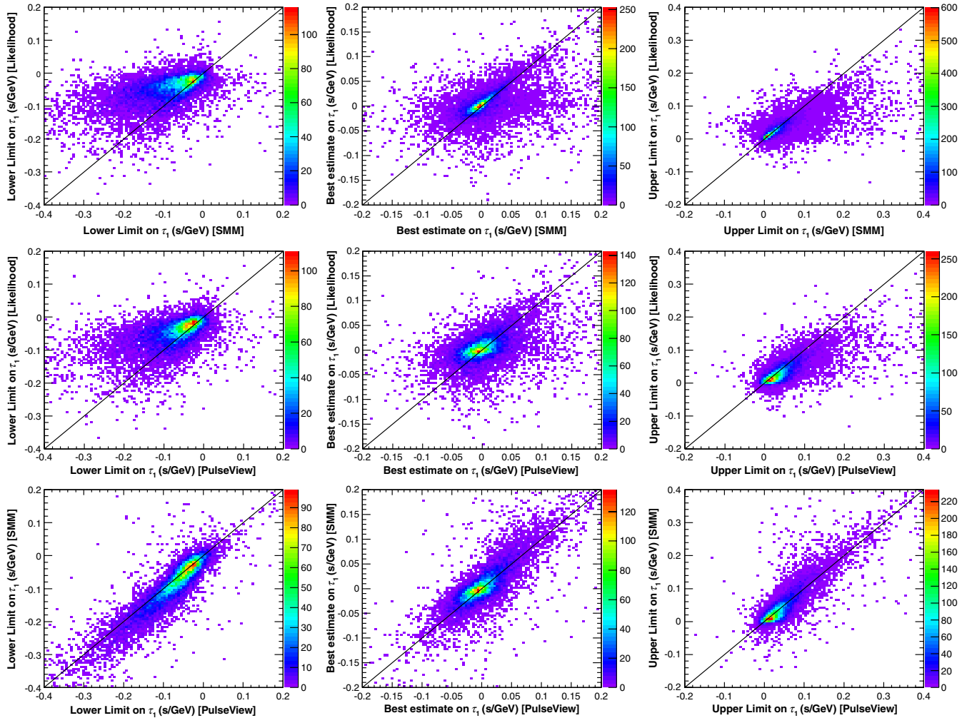
FIG. 21 (color online). One-to-one comparisons of the 95% (one-sided) C.L. lower and upper limits (left and right columns, respectively) and of the best estimates (middle column) on the LIV parameter \tau_1 produced by our three methods on simulated data sets: ML vs SMM (top row), ML vs PV (middle row), SMM vs PV (bottom row).
