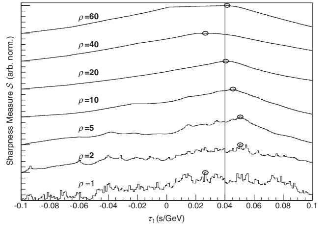
FIG. 3. Curves of SMM’s sharpness measure \mathcal{S}(\tau_n) versus the trial value of the LIV parameter \tau_1 , each produced using a different \rho value. These curves were generated using the GRB 090510-inspired data set described in Appendix A after the application of a dispersion equal to +0.04 s/GeV (value denoted with the vertical line). The circles denote the maxima of the curves, the positions of which are used to produce \hat{\tau}_1 . As can be seen, too small or too large values of \rho correspond to a reduced accuracy for measuring the position of the peak.
