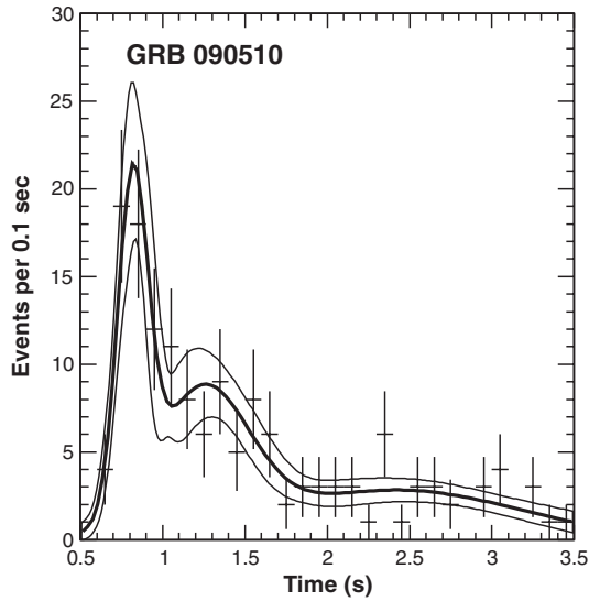
FIG. 6. Template light-curve fit for GRB 090510 used by the ML method. Actual data (histogram), fit template (thick curve), \pm 1\sigma error ranges of the fit (external thin curves).
