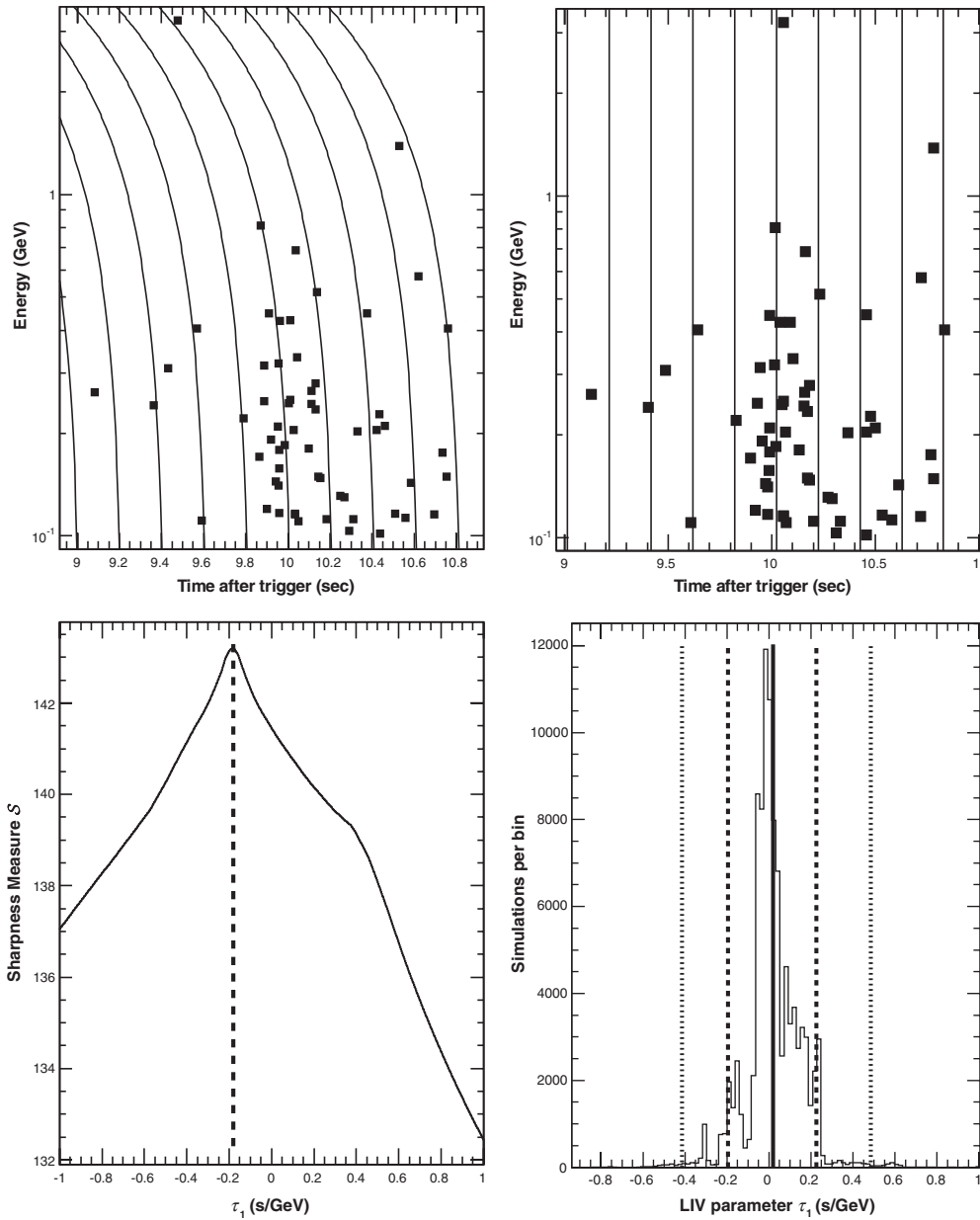
FIG. 11. SMM’s results for GRB 090926A and n = 1 . Top left: photons detected in the default time interval, top right: SMM’s maximally-sharp version of these events. The curves/lines in the top row act as guides to the eye for the effects of a dispersion equal to the best measured value of \hat{\tau}_1 = -0.17 s/GeV (left figure) and zero (right figure). The bottom figures are of the same type as the figures in the right column of Fig. 5.
