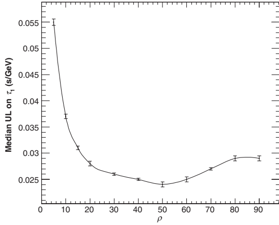
FIG. 4. The median of the distribution of 99% C.L. upper limits (generated from simulated data sets inspired by the detected light curve) versus \rho . The error bars show the 1\sigma statistical uncertainty (arising from the finite number of simulated data sets). This distribution is used for choosing the value of SMM’s \rho parameter for the GRB 090510 n = 1 application.
