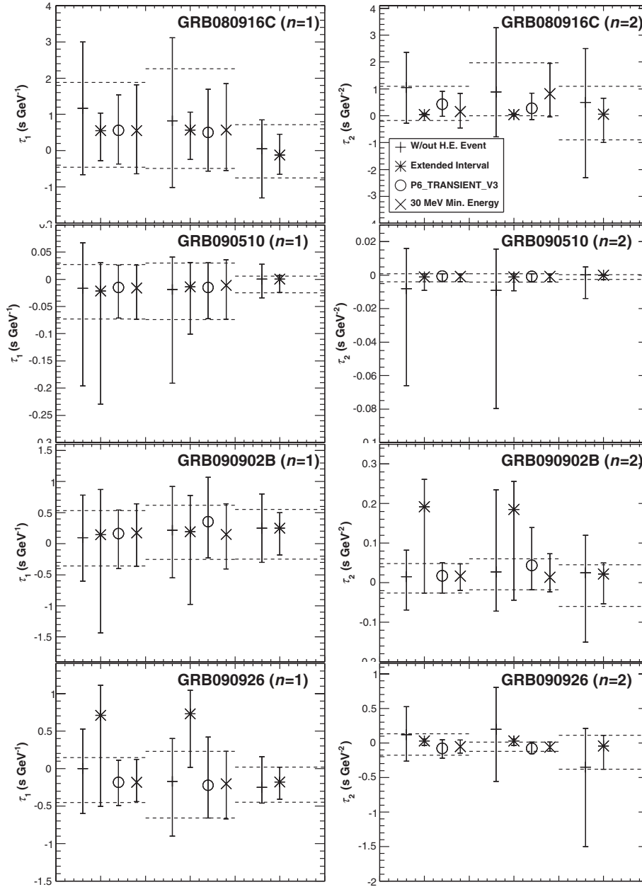
FIG. 22. Comparison between the 99% C.L. CIs on \tau_n obtained with the default configuration (horizontal dashed lines) to those obtained with modified configurations or data sets (vertical error bars). There are three groups of results in each figure, each corresponding to a different method: PV, SMM, ML (from left to right). The ML method CIs shown were produced directly from the data, instead of using calibration simulations.
