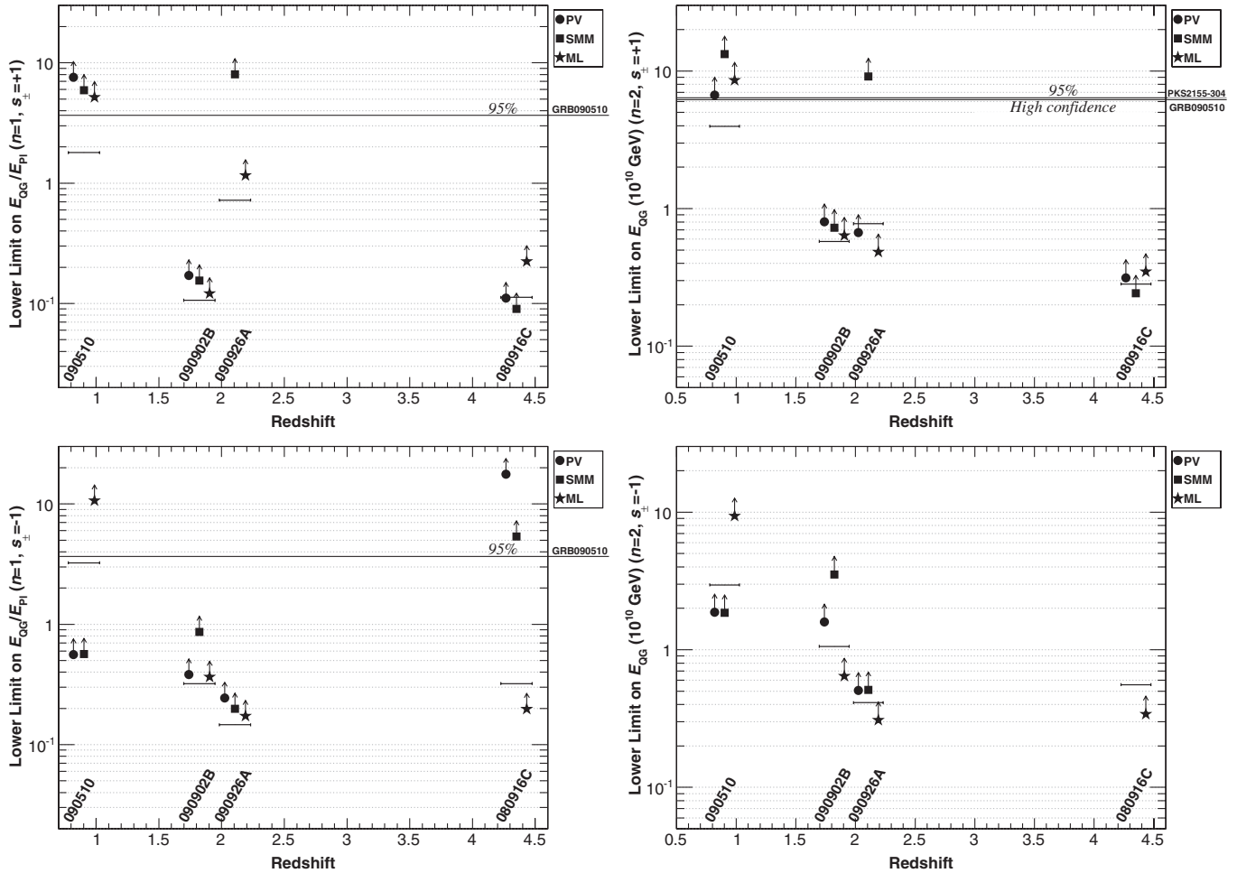
FIG. 10. Our 95% (one-sided) C.L. lower limits on E_{QG,1} (left) and E_{QG,2} (right) LIV versus the redshift for s_{\pm} = +1 (top; subluminal case) and s_{\pm} = -1 (bottom; superluminal case). Similarly to Fig. 9, each triplet of markers corresponds to one GRB and shows limits calculated using the constraints on \tau_n (i.e., without taking into account any source-intrinsic effects). The horizontal bars correspond to the averaged over the three methods lower limits on E_{QG} produced using the constraints on \tau_{LIV} (i.e., after accounting for GRB-intrinsic effects). On the left-hand plots we denote with the horizontal line the limit obtained by Fermi on GRB 090510 (DisCan; 95% limit obtained from paper’s Supplementary Information) [25]. On the top right plot we also denote the “high confidence” and “very high confidence” limits obtained by Fermi on GRB 090510 [25] and the 95% C.L. limit from H.E.S.S. study on PKS 2155-304 [31].
