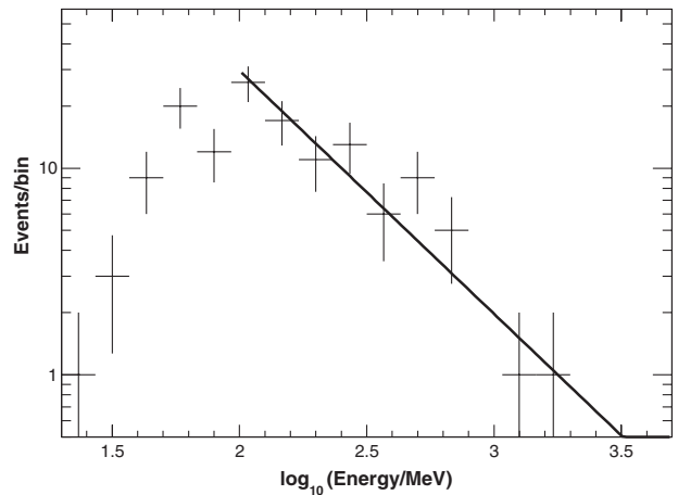
FIG. 7. Fit of the spectrum of detected events from GRB 080916C used to produce the index \gamma of the S(E) function used by the ML method.
