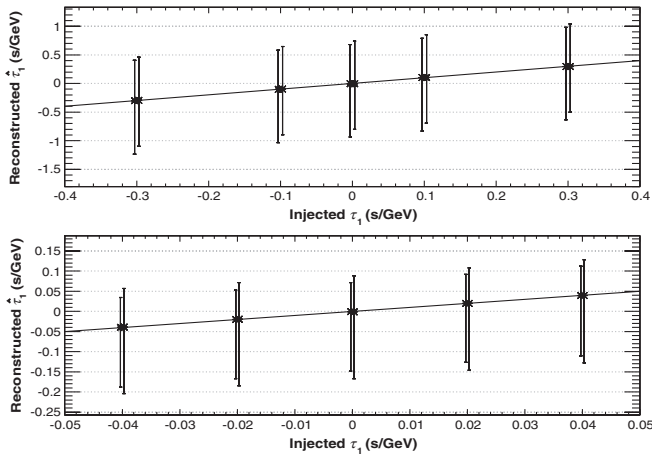
FIG. 15. Calibration plots demonstrating some of the simulation results from the GRB 090902B- and 090510-inspired data sets, top and bottom, respectively. Each pair of intervals corresponds to a different value of the true (injected) LIV parameter \tau_1 , and shows the results from PV (left interval) and SMM (right interval). The markers show the means of the best estimates, and the edges of the intervals correspond to the means of the upper and lower 99% C.L. limits on \tau_1 .
