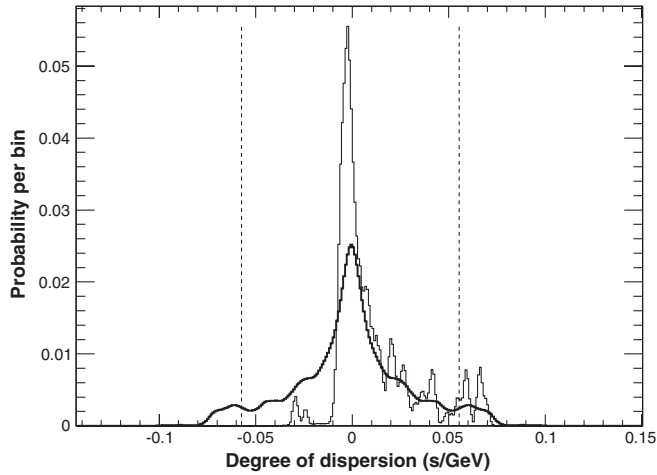
FIG. 12. Demonstration of the generation of CIs on \tau_{\text{LIV}} for GRB 090510, PairView, and n = 1 . The thin curve shows the normalized distribution f_r used to approximate P_{\mathcal{E}}(\epsilon) (the same distribution is also shown with different binning in the bottom left panel of Fig. 5), the thick curve shows the autocorrelation function P_{\mathcal{E}}(\epsilon') calculated using Eq. (26), and the dashed lines show its 5% and 95% quantiles used for constructing the 90% C.L. CI on \tau_{\text{LIV}} .
