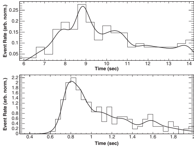
FIG. 13. Two of the light-curve templates used in our verification tests, one inspired by GRB 090902B (top) and one by GRB 090510 (bottom). The histograms are the GRB light curves (as actually detected), and the curves are our templates (produced by a KDE of the histograms).
