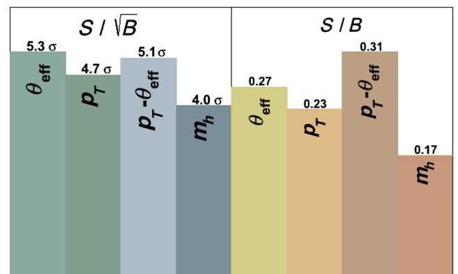
FIG. 6 (color online). Signal significance using various methods of choosing pairs, case I at 14 TeV, with 40 \text{ fb}^{-1} of data.
