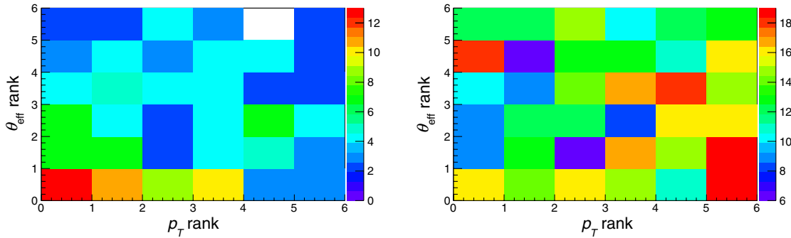
FIG. 4 (color online). p_T vs \theta_{\text{eff}} ranking for correct (left) and wrong (right) b -jet pairs falling inside the mass window [100,140] GeV in signal events, case I at 14 TeV.
