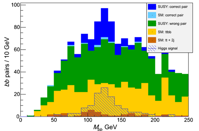
FIG. 5 (color online). B -jet pair invariant mass, case I at 14 TeV.
