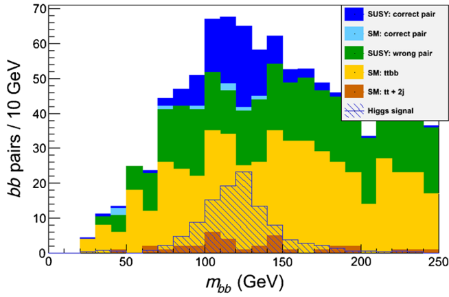
FIG. 7 (color online). b -jet pair invariant mass, case II at 14 TeV.
