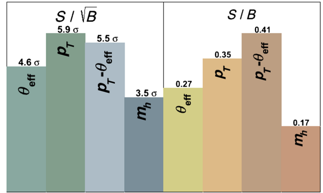
FIG. 8 (color online). Signal significance using various methods of choosing pairs, case II at 14 TeV, with 40 \text{ fb}^{-1} of data.
