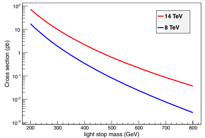
FIG. 2 (color online). The next-to-leading-order cross section of stop pair production at the 8 TeV and 14 TeV LHC generated by Prospino2 [18].
