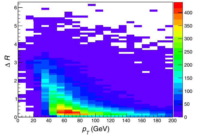
FIG. 3 (color online). p_T vs \Delta R for nontop b\bar{b} quark pairs in t\bar{t}b\bar{b} events.
