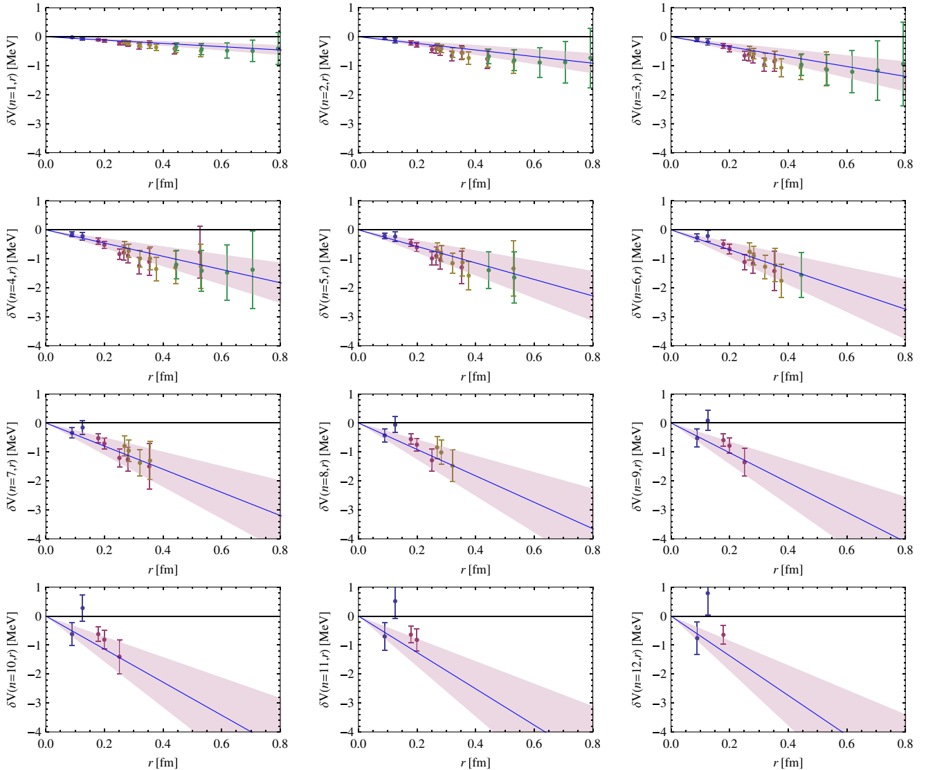
FIG. 1 (color online). Shifts in the static potential computed in Ref. [5] fitted to the simple form discussed in the text.
