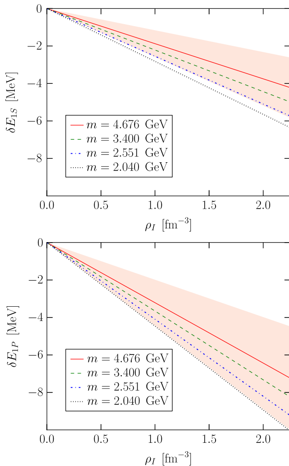
FIG. 2 (color online). Shifts in the energies of the 1S (upper) and 1P (lower) states in quarkonium as a function of the isospin density, computed in a potential model. Results are shown for four different values of the heavy-quark mass with the uncertainty shown only for the mass closest to the physical bottom-quark mass, m = 4.676 GeV (uncertainties for the other masses are of similar size).
