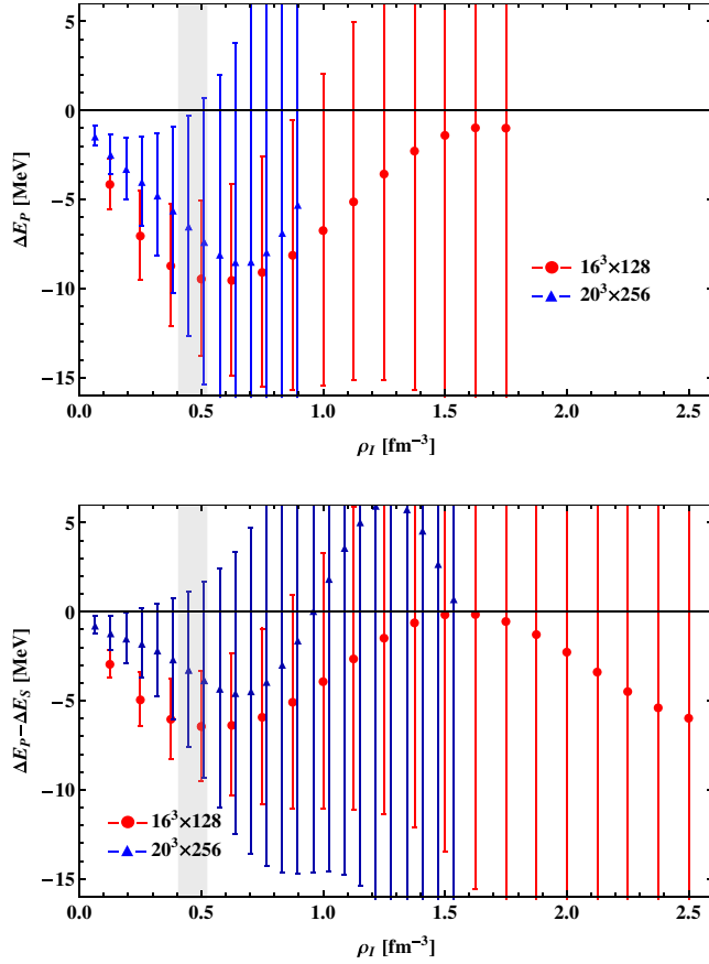
FIG. 14 (color online). Upper panel: the shift in the spin-averaged 1P energy as a function of the isospin charge density. Lower panel: the shift of the spin-averaged 1P - 1S splitting. The vertical band shows the isospin density at which the pionic energy density is peaked relative to the Stefan-Boltzmann expectation. The results are for a_s m = 2.75 .
