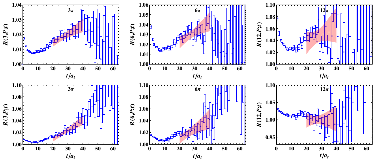
FIG. 13 (color online). The correlator ratios corresponding to the spin-averaged P -wave energy in a medium corresponding to isospin charges n = 3, 6 , and 12 . Data are shown for a_s m = 2.75 on the 20^3 \times 256 (upper) and 16^3 \times 128 (lower) ensembles.
