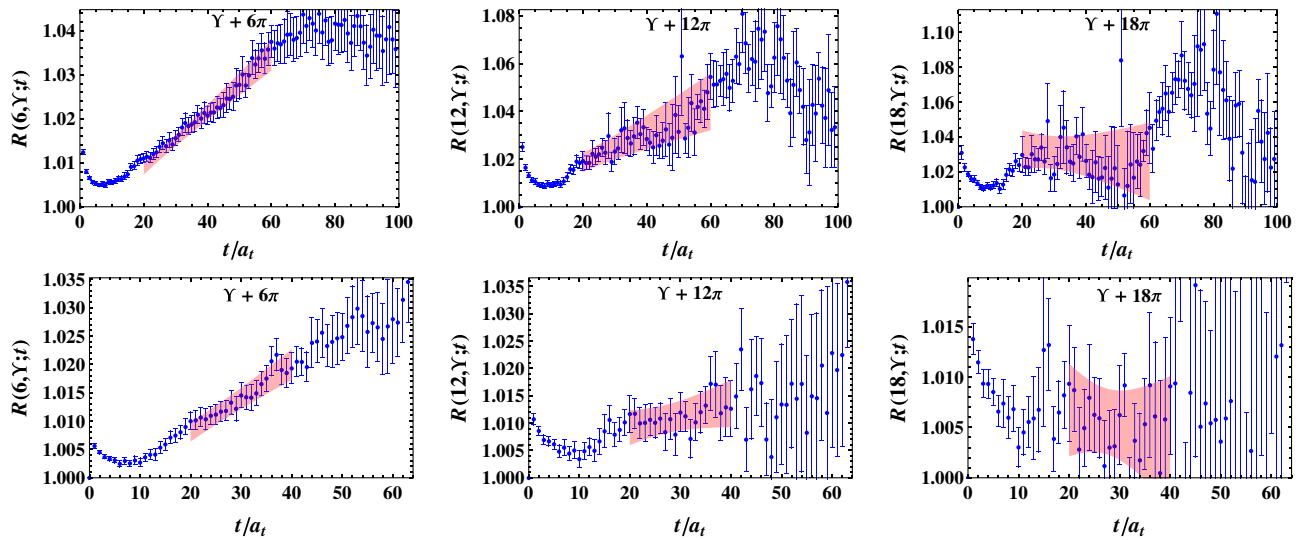
FIG. 8 (color online). The correlator ratios for the Y in a medium corresponding to isospin charges n = 6, 12, 18 . The shaded bands show the statistical uncertainties of fits of the form given in Eq. (18). Data are shown for a_s m = 2.75 on the 20^3 \times 256 (upper) and 16^3 \times 128 (lower) ensembles.
