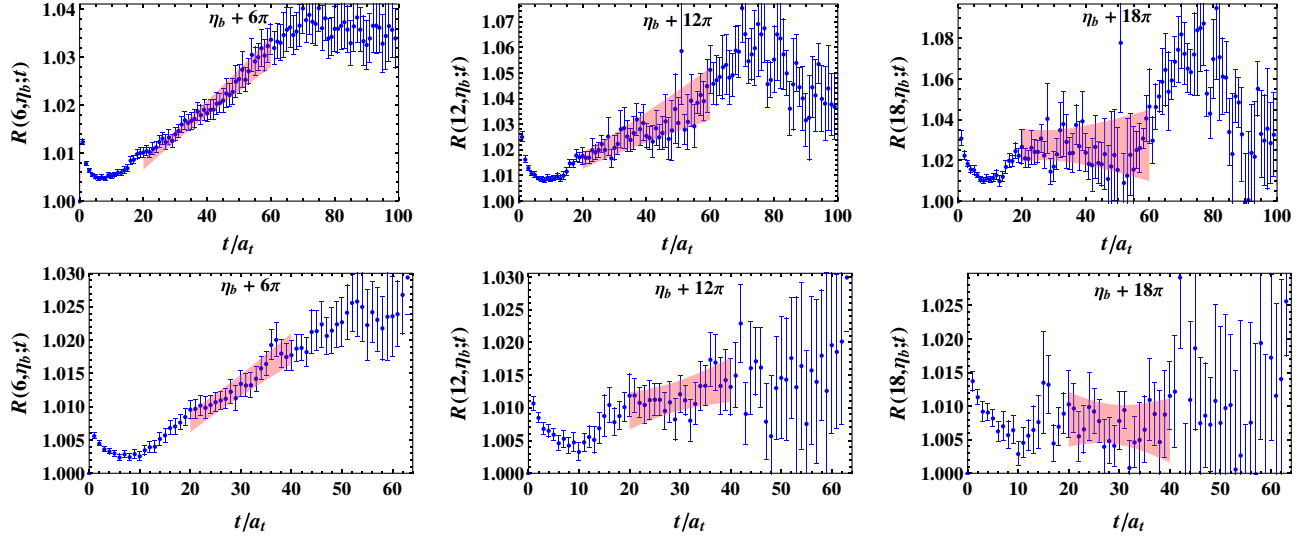
FIG. 9 (color online). The correlator ratios for the \eta_b in a medium corresponding to isospin charges n = 6, 12, 18 . The shaded bands show the statistical uncertainties of fits of the form given in Eq. (18). Data are shown for a_s m = 2.75 on the 20^3 \times 256 (upper) and 16^3 \times 128 (lower) ensembles.
