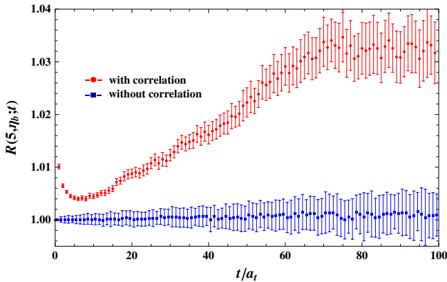
FIG. 5 (color online). The ratio R(5, \eta_b; t) computed with and without the correct correlation between the \eta_b and many-pion system on the 20^3 \times 256 ensemble, as discussed in the main text. The time dependence, which is related to the energy shift through Eq. (18), only appears when correlations are included.
