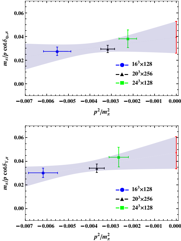
FIG. 6 (color online). Extracted inverse phase shifts for \eta_b - \pi and Y - \pi scattering (at m_\pi \approx 390 MeV). Fitting the phase shift to p \cot \delta(p)/m_\pi = -\frac{1}{m_\pi a} + \frac{m_\pi r}{2} \frac{p^2}{m_\pi^2} , as shown by the shaded band, we can extract the scattering length shown by the point at p^2/m_\pi^2 = 0 .
