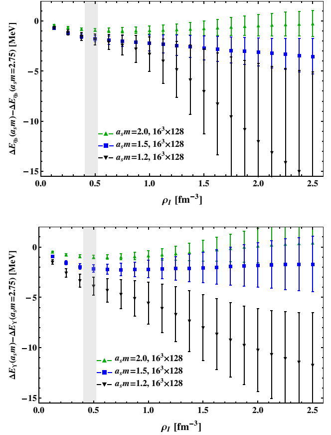
FIG. 15 (color online). The difference of the \eta_b (upper) and Y (lower) energy shift for a given heavy-quark mass from the shift for a_s m = 2.75 is shown as a function of the isospin charge density. Results are shown for the 16^3 \times 128 ensemble.
