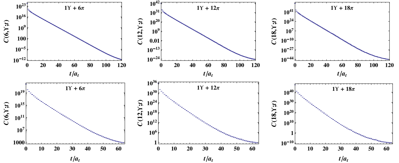
FIG. 7 (color online). The correlators for the Y in a medium corresponding to isospin charge n for n = 6, 12 , and 18 are shown. Data are presented for a_s m = 2.75 on the 20^3 \times 256 (upper) and 16^3 \times 128 (lower) ensembles. Correlators for the \eta_b in medium behave similarly.
