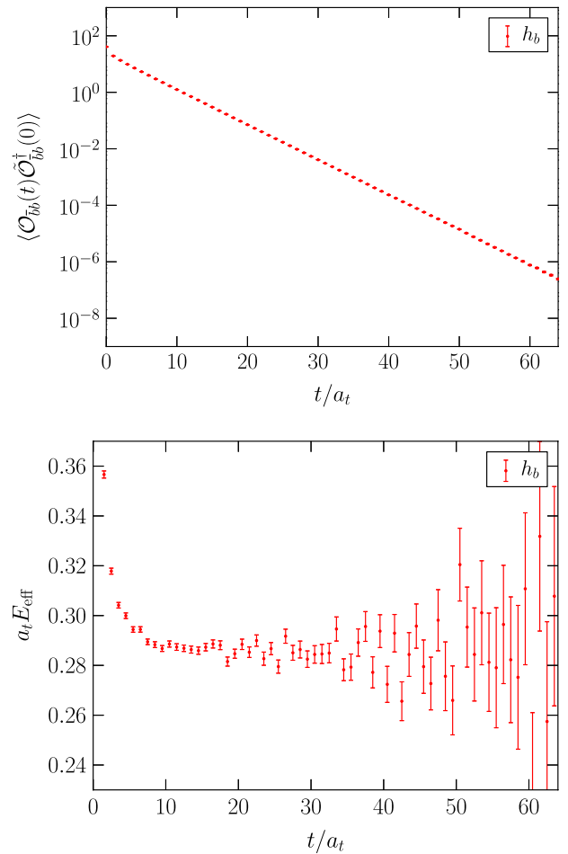
FIG. 4 (color online). h_b correlator (upper) and effective energy (lower) on the 16^3 \times 128 ensemble, for a_s m = 2.75 .
