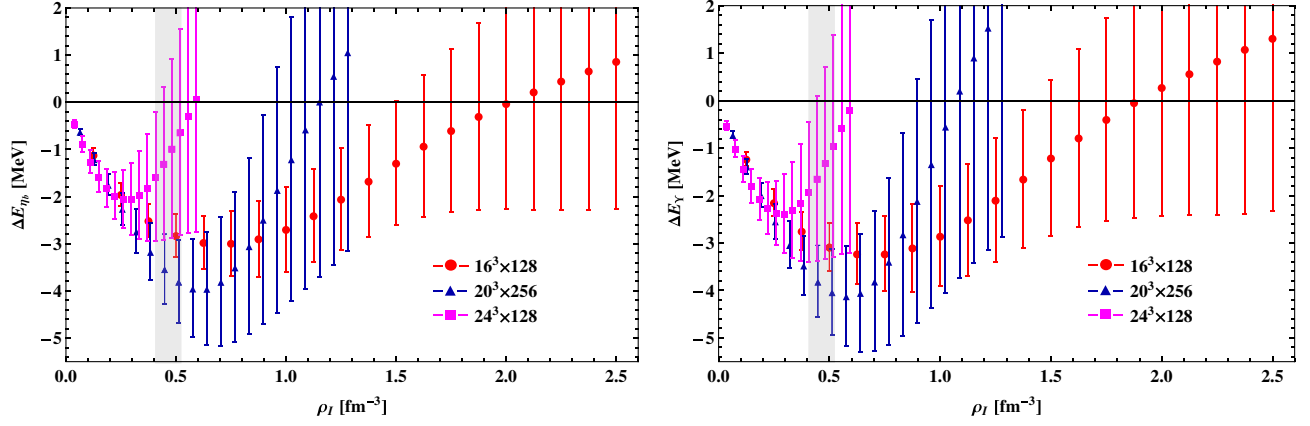
FIG. 10 (color online). The dependence of the energy shift on the isospin charge density is shown for the three lattice volumes for the \eta_b (left panel) and Y (right panel). The results are for a_s m = 2.75 . The shaded vertical band in each plot shows the region where there is a peak in the ratio of the pionic energy density to the Stefan-Boltzmann expectation (see Fig. 22 of Ref. [6]).
