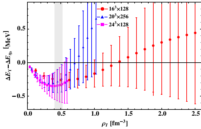
FIG. 12 (color online). Isospin density dependence of the shift of the S -wave hyperfine splitting between the Y and \eta_b states in medium. The results are for a_s m = 2.75 .
