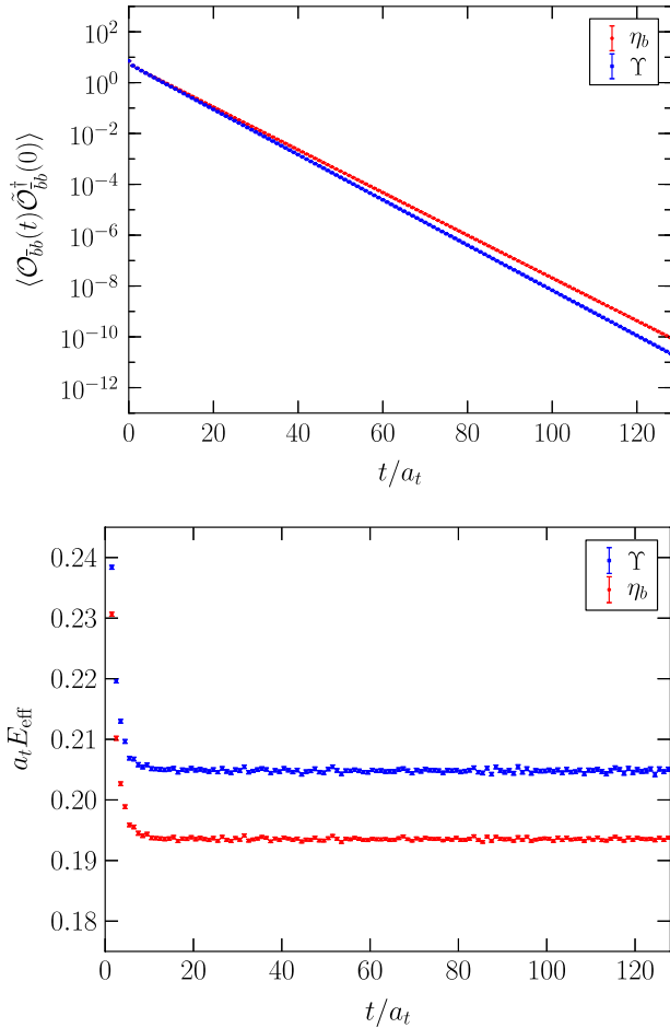
FIG. 3 (color online). \eta_b and \Upsilon correlators (upper) and effective energies (lower) on the 20^3 \times 256 ensemble, for a_s m = 2.75 . The vertical ordering of the legend in each panel is the same as that of the data.
