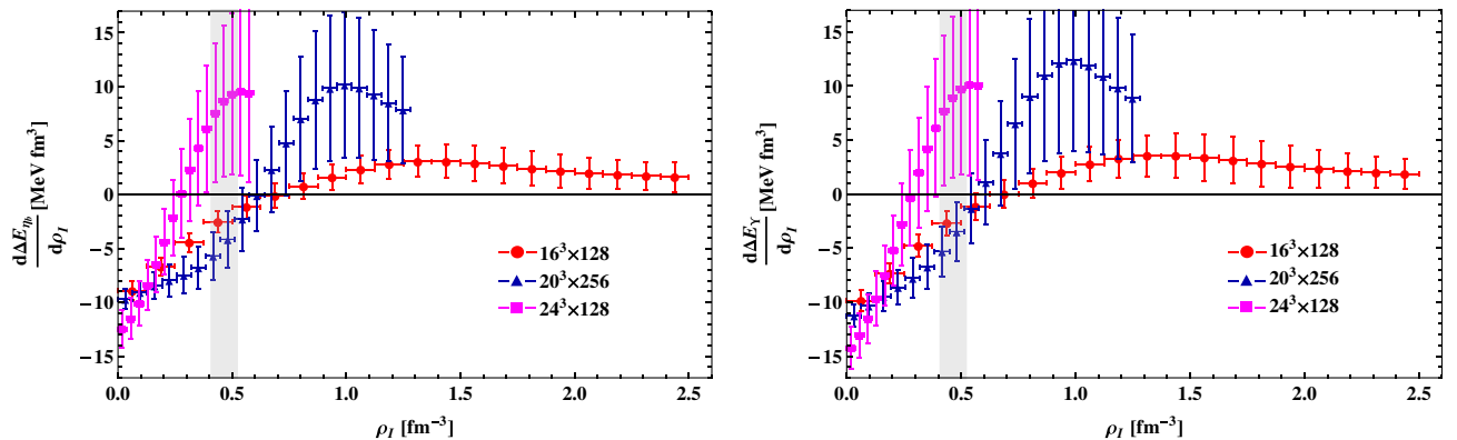
FIG. 11 (color online). The slope d(\Delta E)/d\rho_I of the \eta_b energy shift (left panel) and Y energy shift (right panel), approximated using correlated finite differences. The data sets and shaded bands are as described in Fig. 10.
