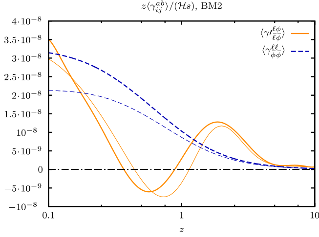
FIG. 11 (color online). Washout reaction densities due to \ell\bar{\ell} \leftrightarrow \bar{\phi}\phi and \ell\phi \leftrightarrow \bar{\ell}\bar{\phi} scattering processes for benchmark point 2. Compare Fig. 10.
