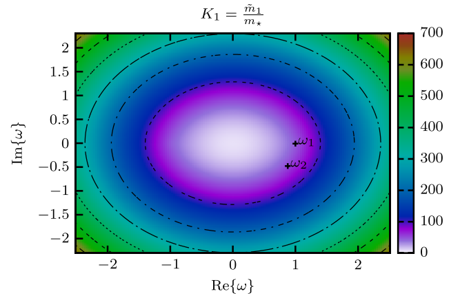
FIG. 22 (color online). Washout parameter for N_1 decay in the complex \omega plane. The values for the benchmark points are K_1(\omega_1) = 47.20 and K_1(\omega_2) = 54.97 . K_1 has a minimum value of K_1(0) = 8.28 .
