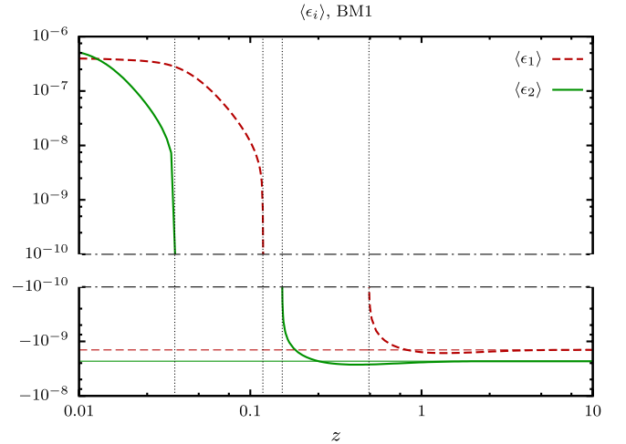
FIG. 16 (color online). Averaged self-energy CP -violating parameters for Majorana neutrino and Higgs decay for benchmark point 1 as a function of the inverse temperature. Thin lines represent the value in the zero temperature limit. With conventional dispersion relations, the decay N_1 \rightarrow \ell\phi is active at z > 4.93 \times 10^{-1} but replaced at high temperatures ( z < 1.18 \times 10^{-1} ) by \bar{\phi} \rightarrow N_1\ell . The decay N_2 \rightarrow \ell\phi is active at z > 1.54 \times 10^{-1} but replaced at high temperatures ( z < 3.62 \times 10^{-2} ) by \bar{\phi} \rightarrow N_2\ell .
