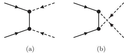
FIG. 3. Two-body scattering process \ell\ell \leftrightarrow \bar{\phi}\bar{\phi} .
