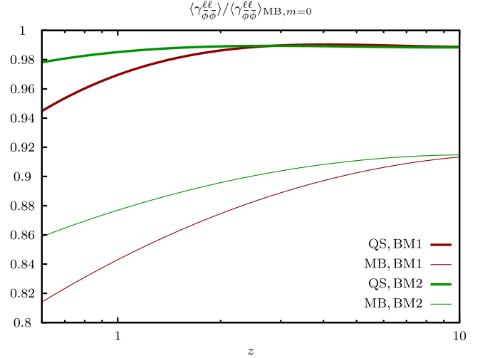
FIG. 12 (color online). Ratio of the reaction density computed using thermal masses with (thick lines) and without (thin lines) the quantum-statistical terms to the canonical one for the two sets of parameters.
