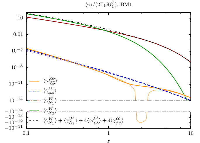
FIG. 13 (color online). Washout reaction densities due to \ell\bar{\ell} \leftrightarrow \bar{\phi}\phi and \ell\phi \leftrightarrow \bar{\ell}\bar{\phi} scattering processes for benchmark point 1 in the approximation of massless leptons and Higgs. For comparison the washout reaction densities for N_1 and N_2 (inverse) decays are shown as well. Note that the normalization differs from the one used in Figs. 10 and 11. For the present choice of parameters, contributions by 2 \leftrightarrow 2 scatterings are strongly suppressed by the smallness of the couplings.
