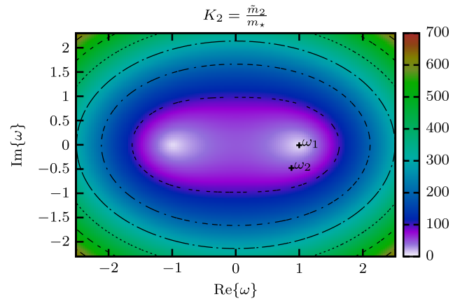
FIG. 23 (color online). Washout parameter for N_2 decay in the complex \omega plane. The values for the benchmark points are K_2(\omega_1) = 9.22 and K_2(\omega_2) = 53.38 . K_2 has a minimum value of K_2(-1) = K_2(1) = 8.28173 .
