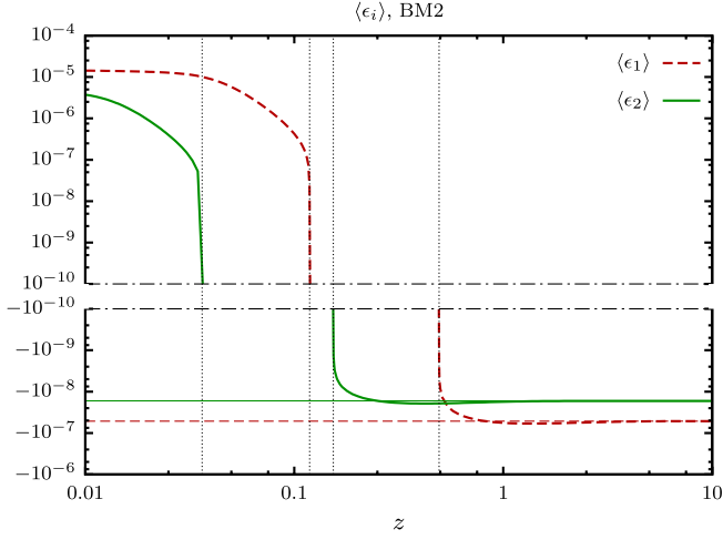
FIG. 17 (color online). Averaged self-energy CP -violating parameters for Majorana neutrino and Higgs decay for benchmark point 2. See caption of Fig. 16.
