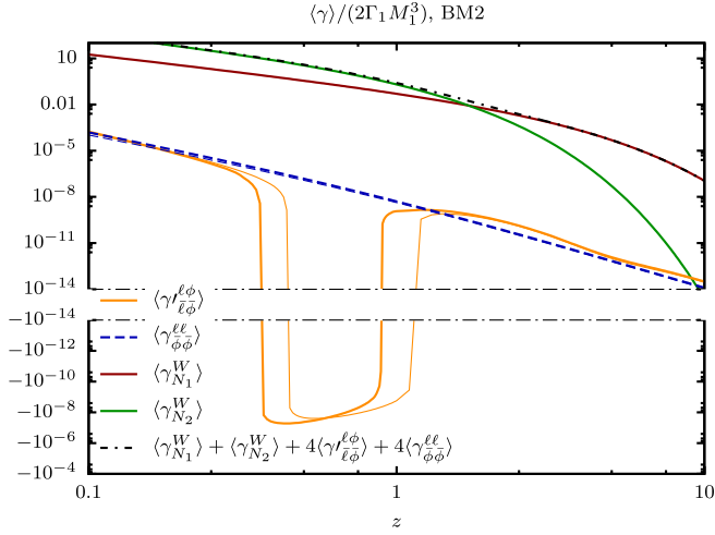
FIG. 14 (color online). Washout reaction densities due to \ell\ell \leftrightarrow \bar{\phi}\bar{\phi} and \ell\phi \leftrightarrow \bar{\ell}\bar{\phi} scattering processes as well as (inverse) decays for benchmark point 2. Compare Fig. 13.
