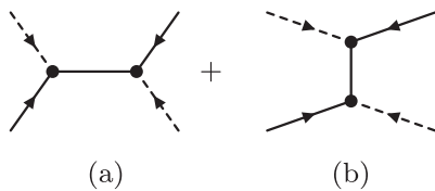
FIG. 2. Two-body scattering process \bar{\ell}\bar{\phi} \leftrightarrow \ell\phi . Both graphs contribute with all N_i as intermediate states. Here (a) is the s -channel contribution and we read (b) as t -channel contribution.
