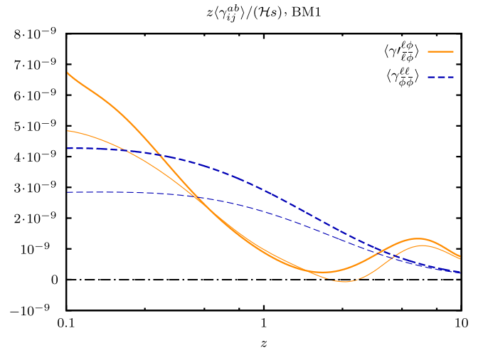
FIG. 10 (color online). Washout reaction densities due to \ell\ell \leftrightarrow \bar{\phi}\bar{\phi} and \ell\phi \leftrightarrow \bar{\ell}\bar{\phi} scattering processes for benchmark point 1 in the approximation of massless leptons and Higgs. Shown are the reaction densities computed using the Boltzmann approximation (42) (thin lines), and taking into account the quantum-statistical effects, (35) (thick lines). The (RIS subtracted) reaction densities \langle\gamma_{ij}^{ab}\rangle may be negative as they are not the physical rates for the 2 \leftrightarrow 2 scattering process.
