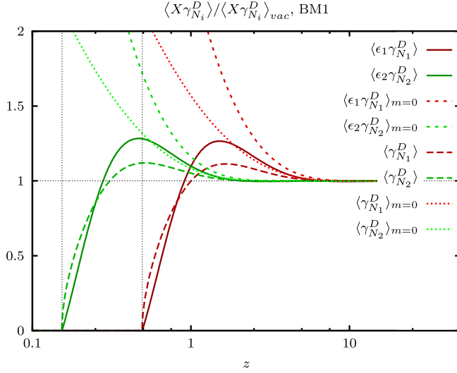
FIG. 9 (color online). Decay and CP -violating reaction densities with thermal lepton and Higgs masses, \langle X \gamma_{N_i}^D \rangle , and with zero masses, \langle X \gamma_{N_i}^D \rangle_{m=0} , for the two Majorana neutrinos N_1 and N_2 . The values are normalized to the corresponding reaction density in the conventional approximation \langle X \gamma_{N_i}^D \rangle_{vac} . The thermal enhancement due to quantum-statistical factors is overcompensated by the phase space suppression due to thermal masses at high temperatures. Note that we show only the self-energy contribution to the CP -violating reaction densities.
