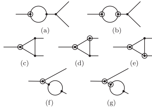
FIG. 21. Circlings contributing to the self-energy (a), (b) and vertex (c)–(e) CP -violating parameter for Majorana neutrino decay and for Higgs decay (f), (g), (c)–(e). The contributions by graphs (b), (f) vanish since N_i and N_j cannot be on-shell simultaneously for i \neq j . Contributions by graphs (c)–(e) are suppressed if the cut is through an internal Majorana neutrino line.
