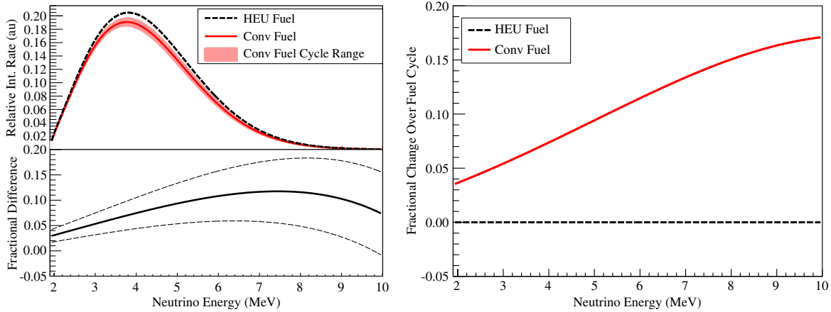
FIG. 5 (color online). Left: Detected reactor \bar{\nu}_e spectra from conventional commercial and HEU fuel (top panel), and their spectral differences (bottom panel). The band indicates the change in the spectral shape over one fuel cycle. Right: Fractional change in spectrum over one fuel cycle for conventional and HEU reactors.
