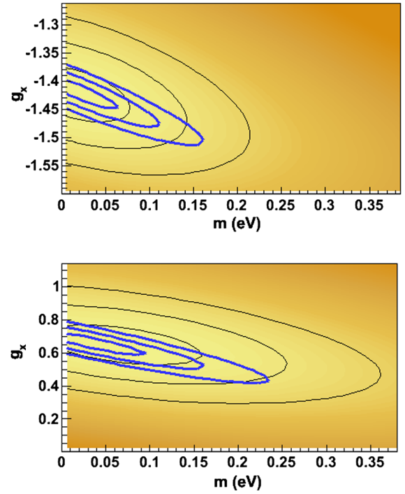
FIG. 1 (color online). 1-, 2-, 3- \sigma probability contours from WMAP + AQS for the bosonic HDM parameters in the case of bosons (up) and boson-antiboson pairs (down) models. Thicker (blue) contours refer to Planck + AQS.
