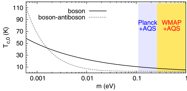
FIG. 2 (color online). Critical temperatures of condensation (evaluated today) as a function of the mass for each model. For bosons, the lower limit T_{c,0}^{\phi} \geq 10.33 K is higher than our best fit of T_0^{\phi} = 2.14 K. For boson-antiboson, the limiting-critical temperature is comparable with the bosonic temperature.
