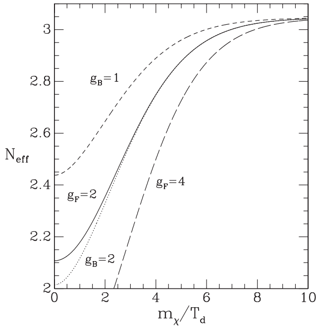
FIG. 1. The effective number of neutrino degrees of freedom, N_{\text{eff}} , that would be deduced from cosmic microwave background observations for a thermal dark matter particle with mass m_\chi , assuming sudden decoupling of the cosmic neutrinos at a temperature T_d . Curves correspond, top to bottom, to a g = 1 boson (short dash), g = 2 fermion (solid), g = 2 boson (dotted), and g = 4 fermion (long dash).
