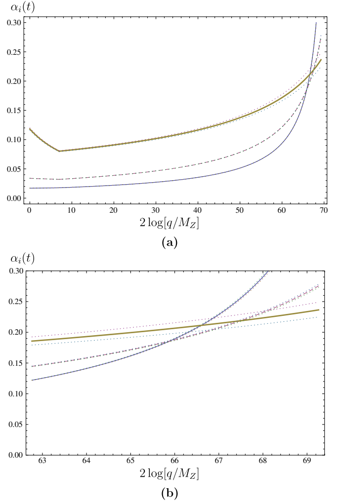
FIG. 2 (color online). Two-loop RG flow of gauge couplings in scenario B: (a) evolution of SU(3)_C , SU(2)_W and U(1)_Y couplings from the EW scale to the GUT scale for \tilde{T}_S = 3\text{ TeV} and n_S = 0 ; (b) running of SM gauge couplings near the scale M_X for \tilde{T}_S = 3\text{ TeV} and n_S = 0 . The parameters and notations are the same as in Fig. 1.
