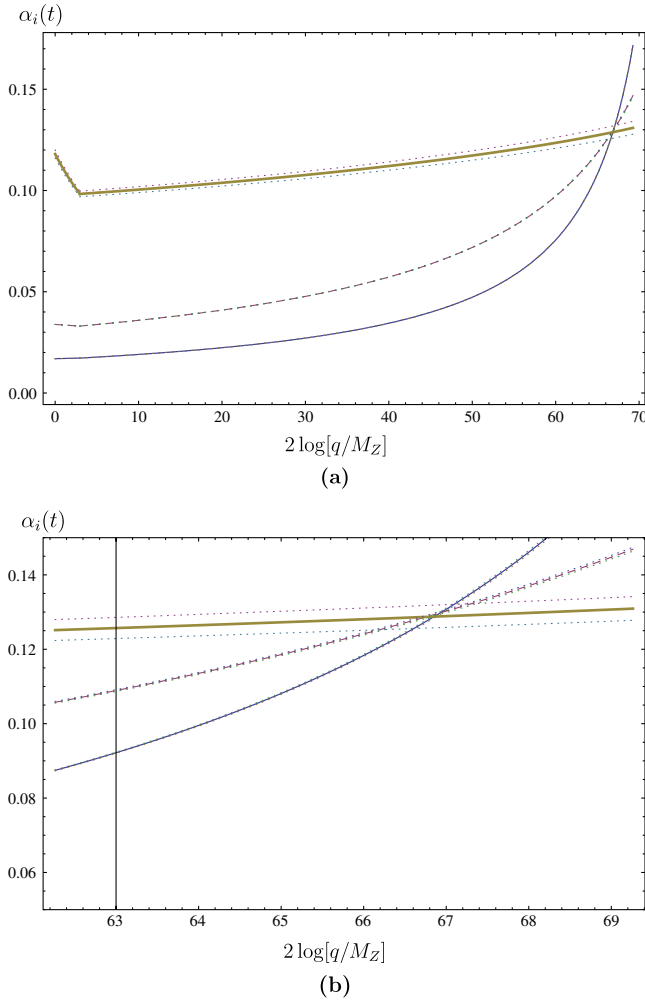
FIG. 1 (color online). Two-loop RG flow of gauge couplings in scenario A: (a) RG flow of SU(3)_C , SU(2)_W and U(1)_Y couplings from M_Z to M_X for T_S = 400\text{ GeV} and n_S = 1 ; (b) running of SM gauge couplings in the vicinity of M_X for T_S = 400\text{ GeV} and n_S = 1 . Thick, dashed and solid lines correspond to the running of SU(3)_C , SU(2)_W and U(1)_Y couplings, respectively. We used \tan\beta = 10 , \alpha_s(M_Z) = 0.118 , \alpha(M_Z) = 1/127.9 , \sin^2\theta_W = 0.231 and \kappa_1(T_S) = \kappa_2(T_S) = \kappa_3(T_S) = \lambda_1(T_S) = \lambda_2(T_S) = \lambda_3(T_S) = g'_1(T_S) . The dotted lines represent the uncertainty in \alpha_i(t) caused by the variation of the strong gauge coupling from 0.116 to 0.120 at the EW scale.
