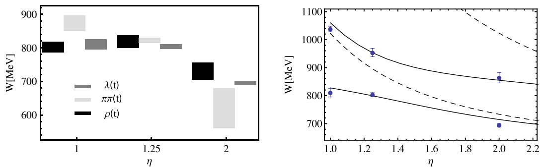
FIG. 2 (color online). Left panel: Ground state energies for the three different elongations extracted using different methods. Right panel: Ground and first excited state energies compared to the effective range formula using the parameters extracted from our fits. The dashed lines represent the expected two-pion energies in the absence of interaction, i.e., W_n = 2\sqrt{m_\pi^2 + (2\pi n/\eta L)^2} .
