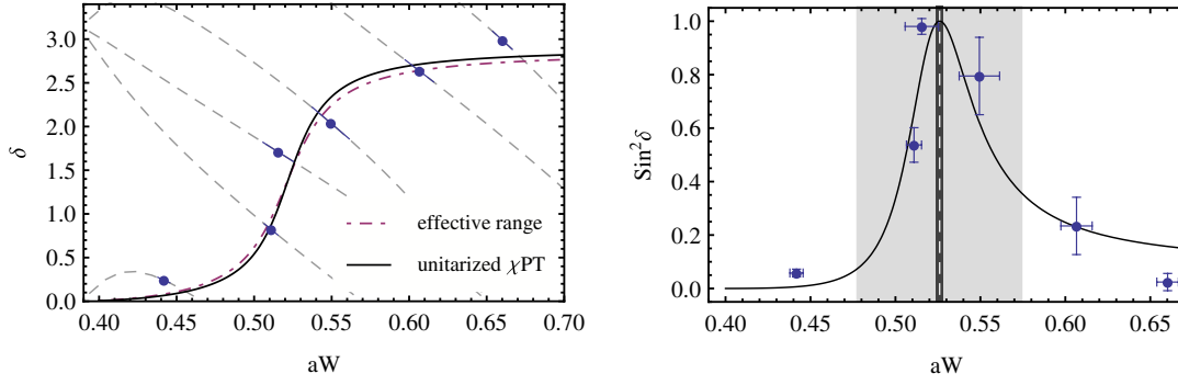
FIG. 3 (color online). Left panel: Scattering phase shifts computed in this study, effective range formula fit, and the results from unitarized \chi PT [14]. The dashed lines describe the energy dependence of the phase shift according to Eq. (8). Right panel: Cross section as a function of the center-of-mass energy. The dashed line indicates the \rho mass, the narrow dark band its error, and the shadowed box indicates the resonance region m_\rho \pm \Gamma .
