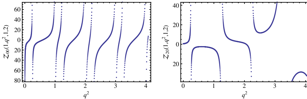
FIG. 5 (color online). Z_{00}(1, q^2, 1, 2) and Z_{20}(1, q^2, 1, 2) .
