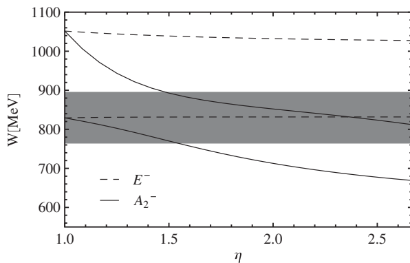
FIG. 1. Estimated spectrum for m_\pi = 300 MeV, g_{\rho\pi\pi} = 6 , and m_\rho = 830 MeV. The lattice size is set to L = 3 fm. The two curves indicate the ground and first excited states. The shaded region is the resonance region, i.e., m_\rho \pm \Gamma_\rho .
