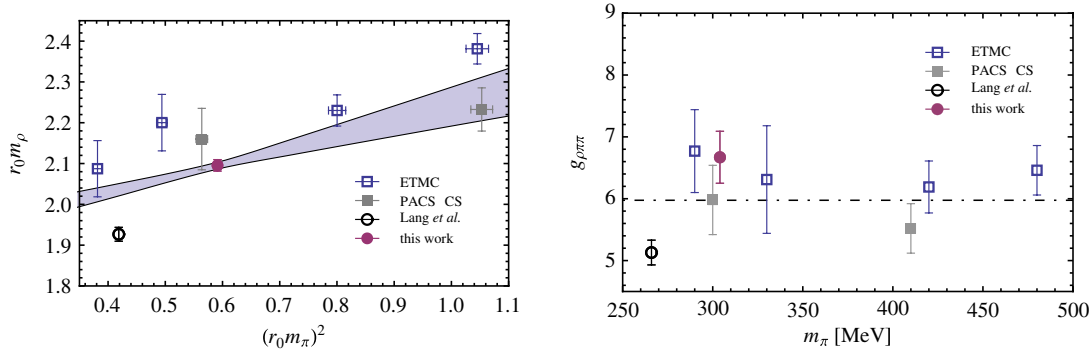
FIG. 4 (color online). Left panel: m_\rho versus m_\pi from recent lattice studies. We use lattice units to remove the uncertainty associated with setting the scale. The band represents the prediction from unitarized \chi PT [14] (note that this is not a fit to our data). Right panel: Coupling as a function of m_\pi from recent lattice studies. The dot-dashed line is the Particle Data Group result [15].
