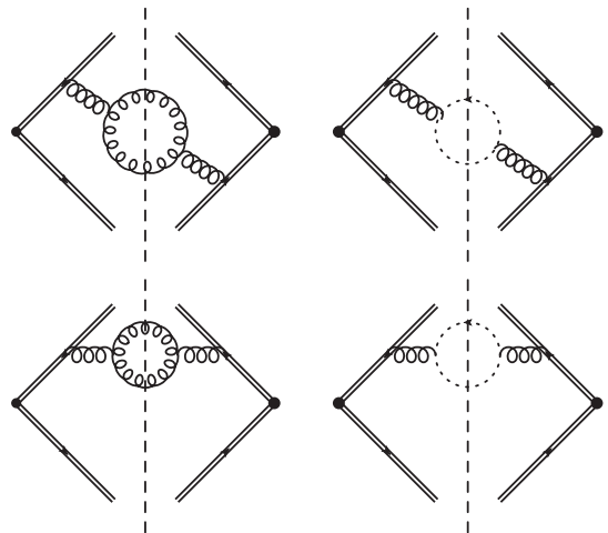
FIG. 4. Diagrams involving gluon or ghost bubbles with two cut particles. The four additional diagrams obtained by a flip about the horizontal or vertical axis are not shown. Diagrams with one cut particle for wave function renormalization and coupling renormalization are also not displayed.
