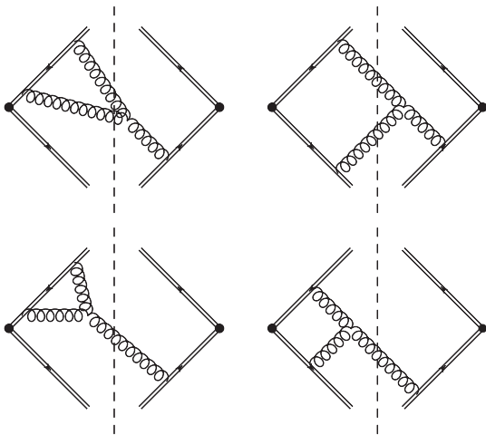
FIG. 7. Triple gluon Y-diagrams for the \mathcal{O}(\alpha_s^2) correction to \Omega_1(r) . The 12 additional diagrams obtained by a horizontal flip or complex conjugation are not shown. Diagrams with all 3 gluons coupled to Wilson lines of the same direction vanish.
