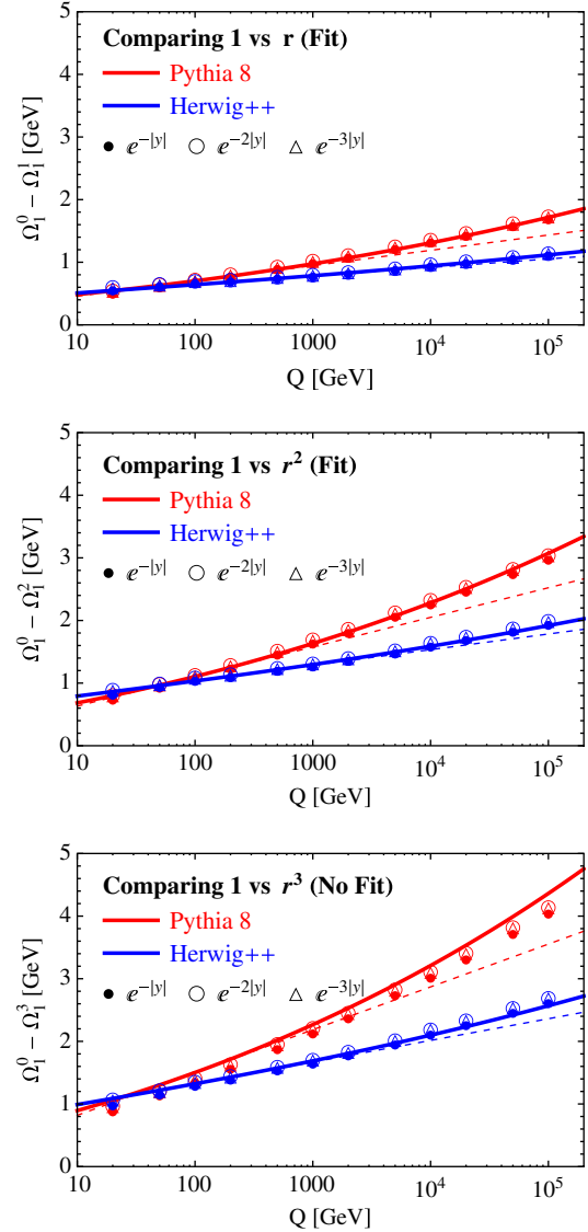
FIG. 8 (color online). Universal power corrections extracted from Pythia 8.162 (upper solid and dashed lines and dots) and Herwig++ 2.6.0 (lower solid and dashed lines and dots) for the generalized angularities \tau_{(n,a)} . We use the measured power corrections in the first two plots to fit for \Omega(r, \mu_0) at Q = 100 GeV, using Eq. (64) to evolve to different Q scales. The curves in the third plot are then predicted. The dashed curves show the approximate formula in Eq. (66).
