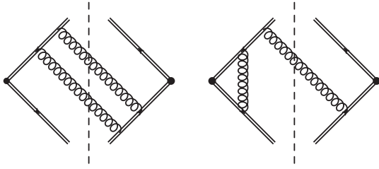
FIG. 5. Purely Abelian \mathcal{O}(\alpha_s^2) diagrams. Either gluon line crossing the cut can be the source. The 4 additional diagrams obtained by a flip about the horizontal or vertical axis are not shown.
