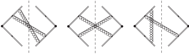
FIG. 6. Independent emission diagrams with Abelian and non-Abelian contributions. The four additional diagrams obtained by a horizontal flip or complex conjugation are not shown.
