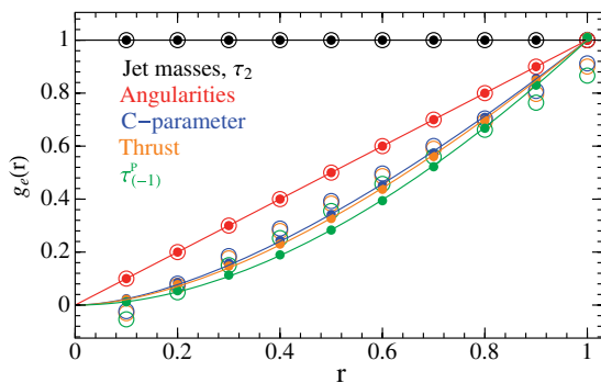
FIG. 2 (color online). From top to bottom, the g_e(r) functions for jet masses and 2-jettiness, angularities, C parameter, thrust, and the P -scheme angularity with a = -1 . Lines correspond to exact numerical values, open circles to two terms from the basis of Sec. IVD, and filled circles to three terms from the basis.
