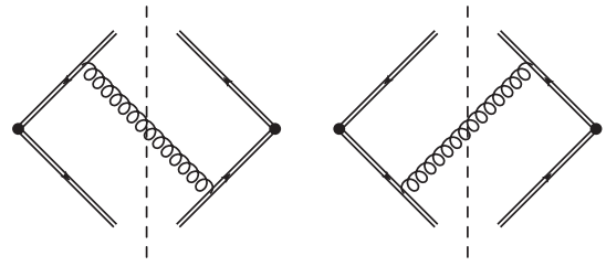
FIG. 3. Tree-level graphs for \Omega_1(r, \mu) .
