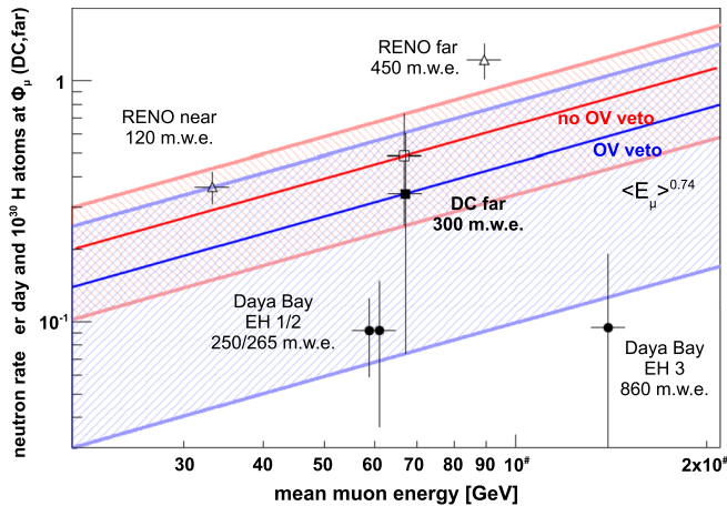
FIG. 2 (color online). Scaling of DC fast- n background rates and comparison with quoted values. Empty (full) markers indicate quoted results using a selection without (with) an external muon veto; lines and shaded bands represent our scaling of the DC measurements with their uncertainty [blue, forward hatched (with OV veto); red, backward hatched (without OV veto)]. Values were scaled by number of H atoms and normalized to muon flux at DC far site.
