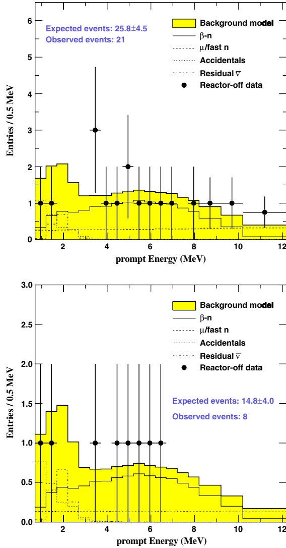
FIG. 1 (color online). \bar{\nu}_e candidates in the reactor-off data sample, with breakdown by components. Top and bottom figures show DCI and DCII selection results, respectively. Black points: data; histogram: background + \bar{\nu}_e expectation.
