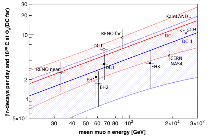
FIG. 3 (color online). Scaling of DC \beta - n -decay rates and comparison with quoted values. Results were scaled by a number of carbon atoms and normalized to muon flux at the DC far site. Solid lines correspond to rate uncertainties in the reactor-off analysis: DCI (red solid line) and open data points compare the total \beta - n rate, while DCII (blue solid line) and filled data points correspond to analyses with an extended veto following showering muons. Shaded regions indicate uncertainties (red, backward-hatched DCI; blue, forward-hatched DCII).
