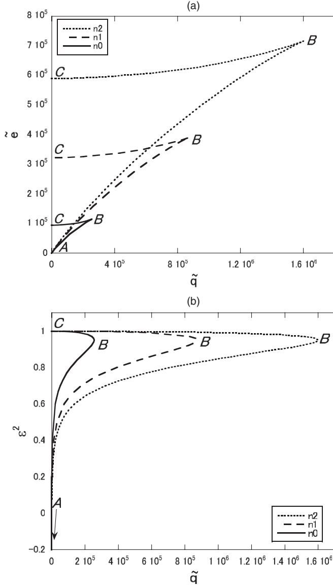
FIG. 12. (a) \tilde{q} - \tilde{e} and (b) \tilde{q} - \epsilon^2 relations for V_{\text{grav}} : K = -0.1 .
