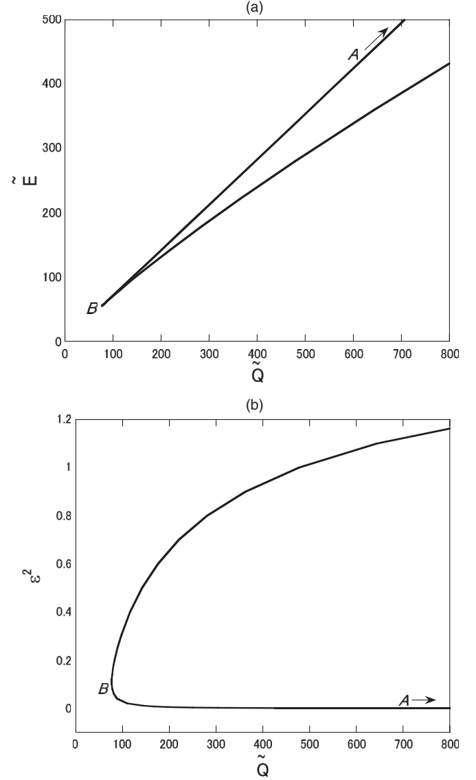
FIG. 13. (a) \tilde{Q} - \tilde{E} and (b) \tilde{Q} - \epsilon^2 relations for V_{\text{gauge}} .
