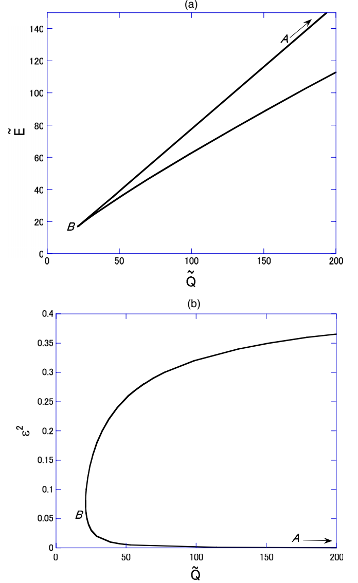
FIG. 7 (color online). (a) \tilde{Q} - \tilde{E} and (b) \tilde{Q} - \epsilon^2 relations for type I Q -balls in the V_4 model: \tilde{m}^2 = 0.6 .
