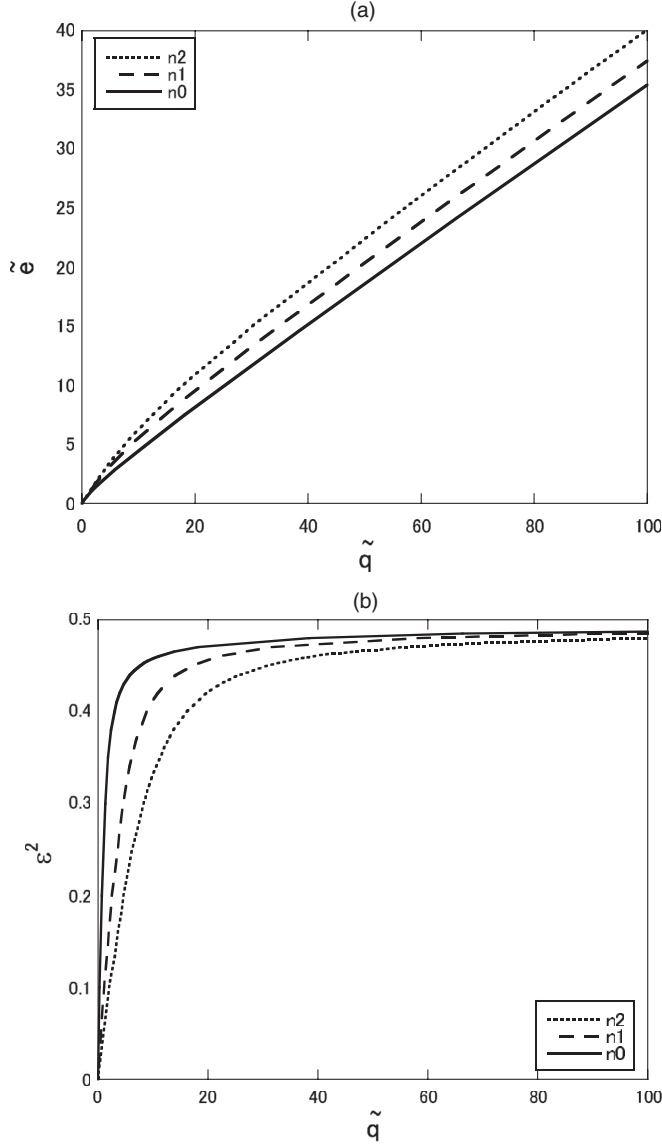
FIG. 4. (a) \tilde{q} - \tilde{\epsilon} and (b) \tilde{q} - \tilde{\epsilon}^2 relations for type I Q -tubes in the V_3 model: \tilde{m}^2 = 0.6 .
