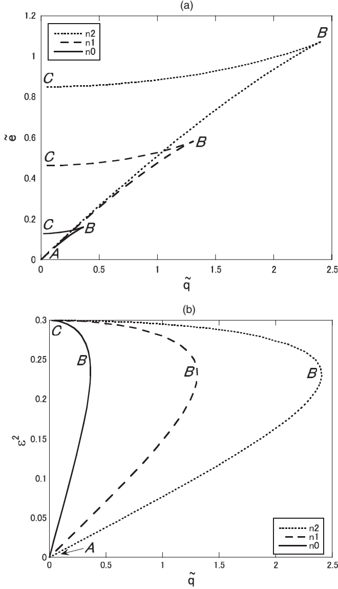
FIG. 6. (a) \tilde{q} - \tilde{\epsilon} and (b) \tilde{q} - \epsilon^2 relations for type I Q -tubes in the V_3 model: \tilde{m}^2 = 0.3 .
