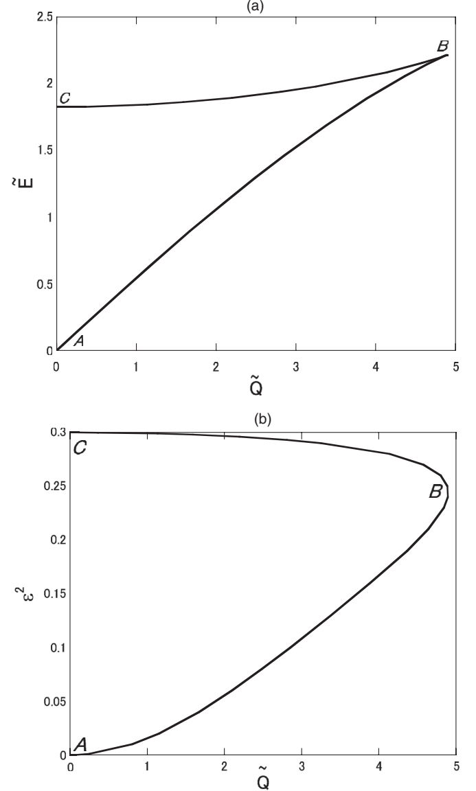
FIG. 5. (a) \tilde{Q} - \tilde{E} and (b) \tilde{Q} - \tilde{\epsilon}^2 relations for type I Q -balls in the V_3 model: \tilde{m}^2 = 0.3 .
