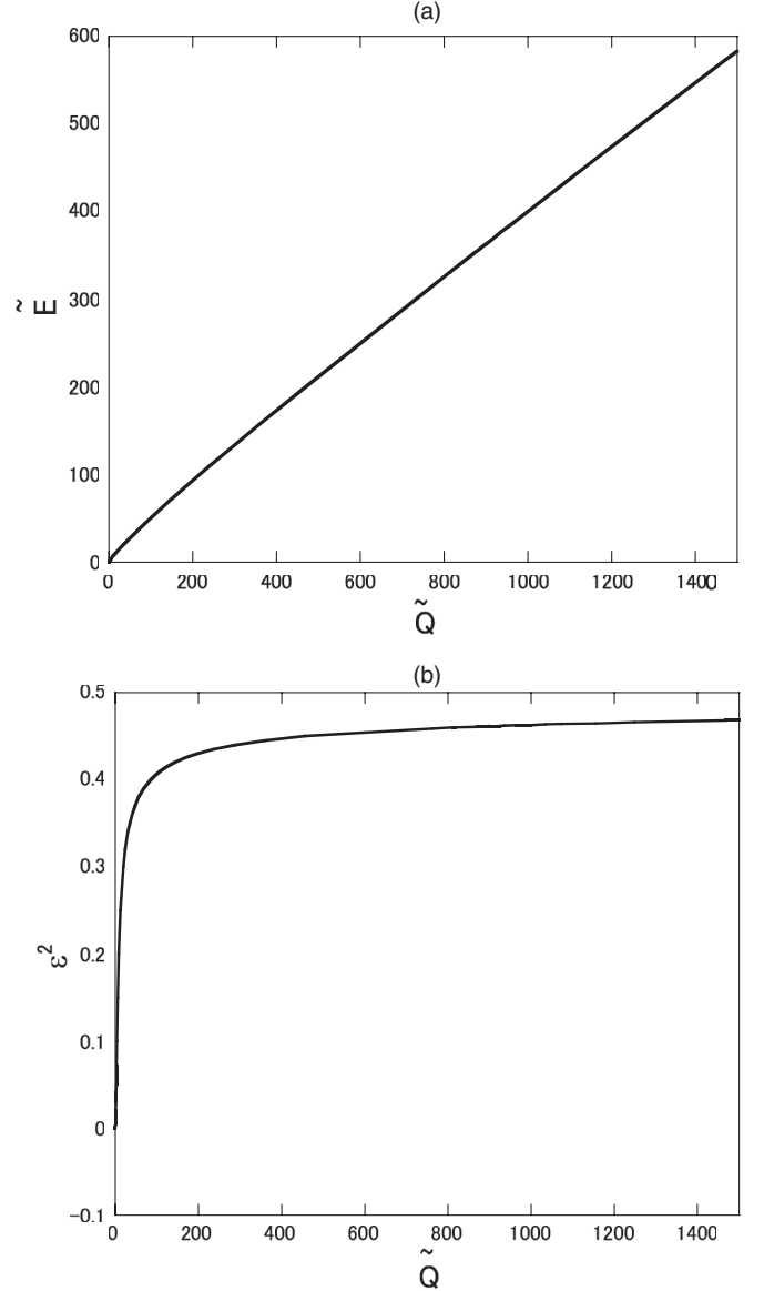
FIG. 3. (a) \tilde{Q} - \tilde{E} and (b) \tilde{Q} - \epsilon^2 relations for type I Q -balls in the V_3 model: \tilde{m}^2 = 0.6 .
